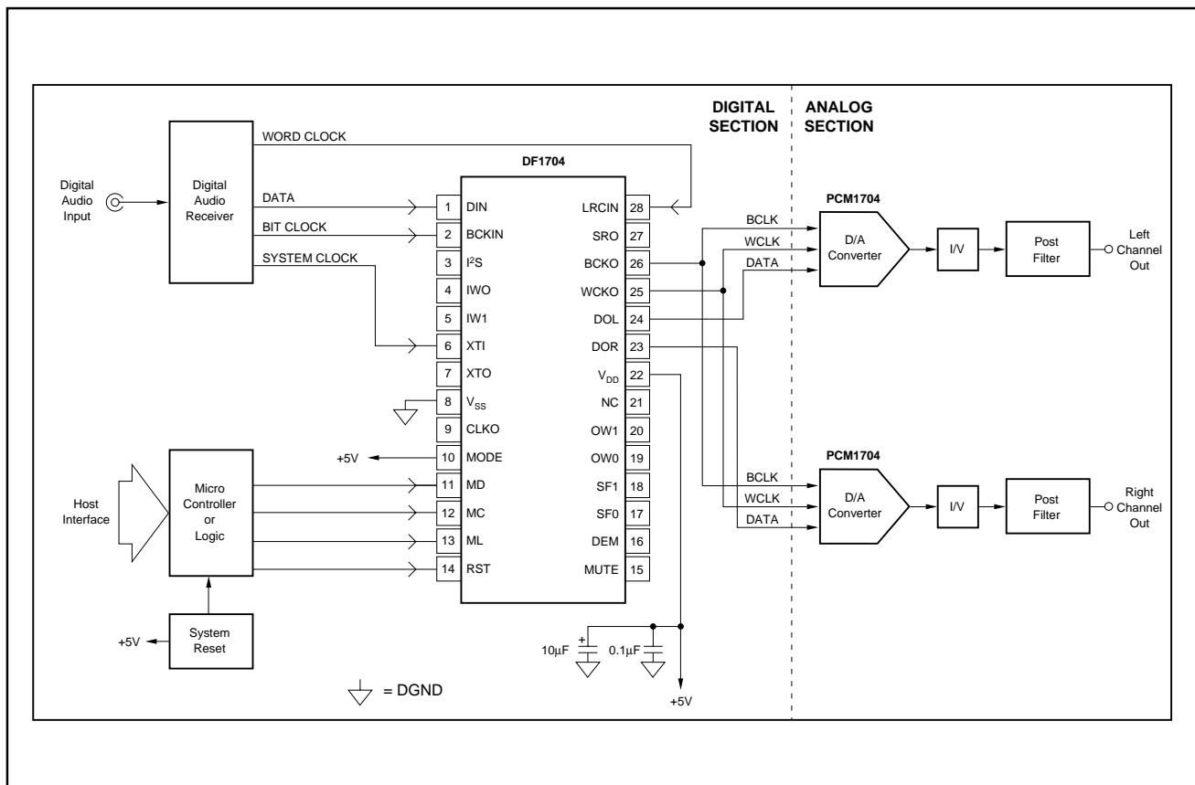
FIGURE 14. DF1704 Typical Application Circuit.
