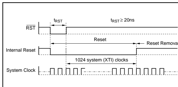
FIGURE 3. External Forces Reset Timing.
