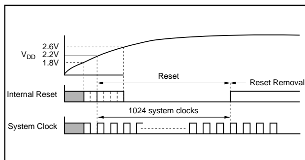
FIGURE 2. Internal Power-On Reset Timing.
