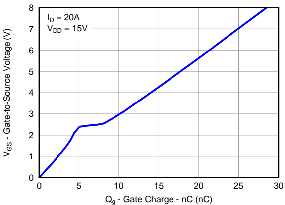
Figure 14. Control MOSFET Gate Charge
