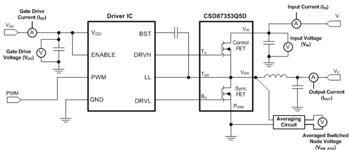
Figure 32. Typical Application
