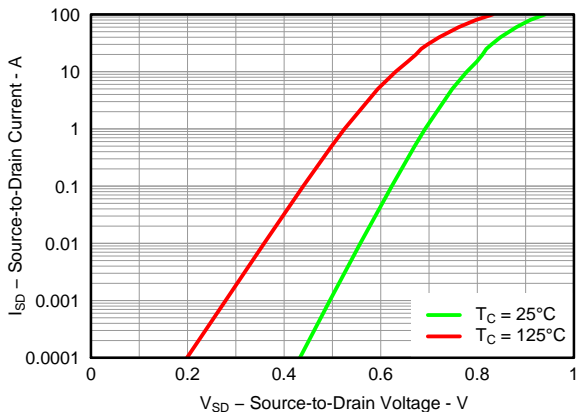
Figure 24. Control MOSFET Body Diode
