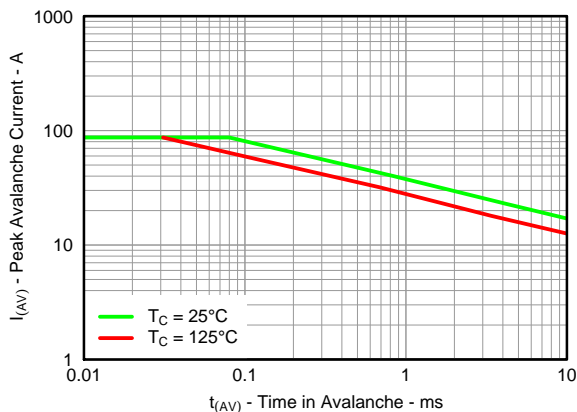
Figure 26. Control MOSFET Unclamped Inductive Switching
