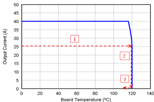
Figure 33. Power Block SOA
