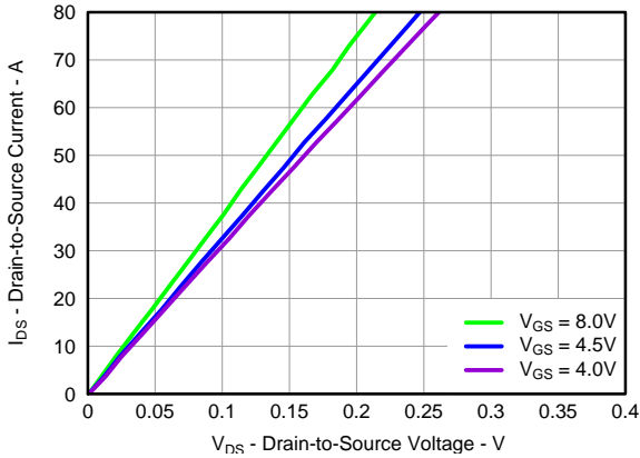
Figure 10. Control MOSFET Saturation
