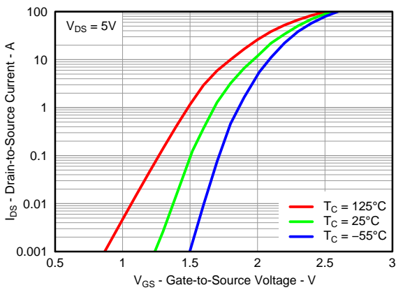
Figure 12. Control MOSFET Transfer
