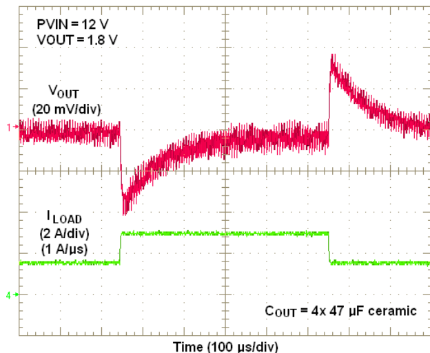
Figure 20. PVIN = 12V, VOUT = 1.8V, 1.5A Load Step
