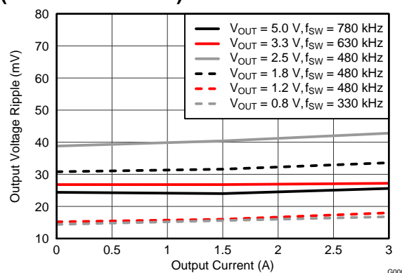
Figure 2. Voltage Ripple vs. Output Current
