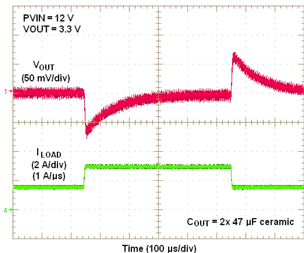
Figure 22. PVIN = 12V, VOUT = 3.3V, 1.5A Load Step
