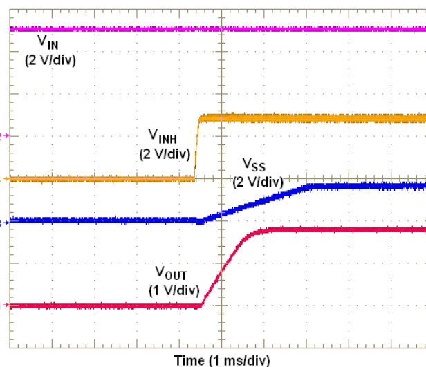
Figure 31. Inhibit Turn-On
