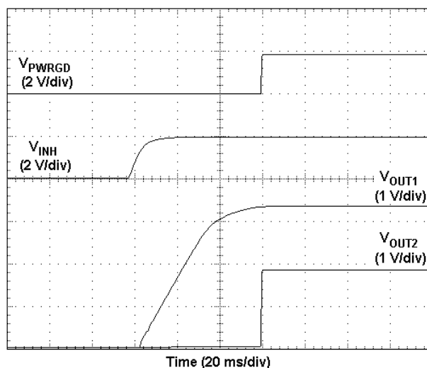
Figure 37. Sequencing Waveforms
