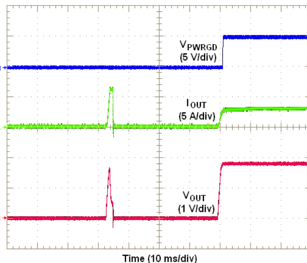
Figure 34. Removal of Overcurrent Condition
