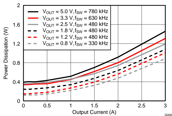
Figure 3. Power Dissipation vs. Output Current
