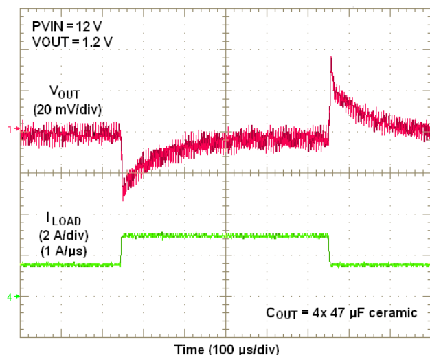
Figure 18. PVIN = 12V, VOUT = 1.2V, 1.5A Load Step
