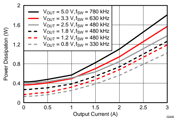
Figure 13. Power Dissipation vs. Output Current
