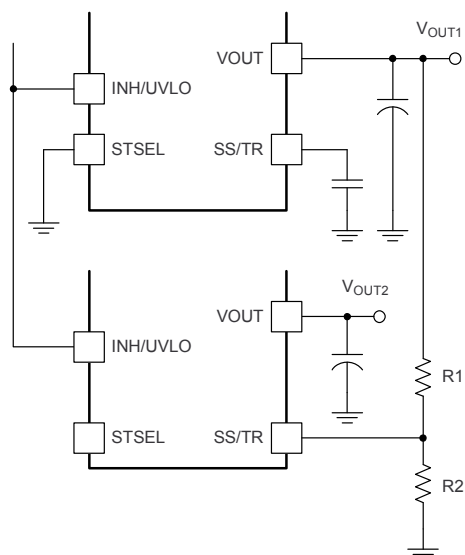
Figure 38. Simultaneous Tracking Schematic
