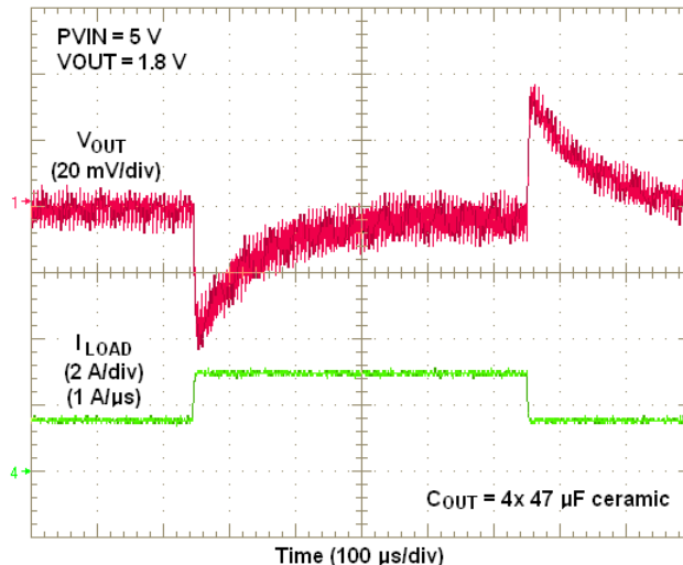
Figure 21. PVIN = 5V, VOUT = 1.8V, 1.5A Load Step
