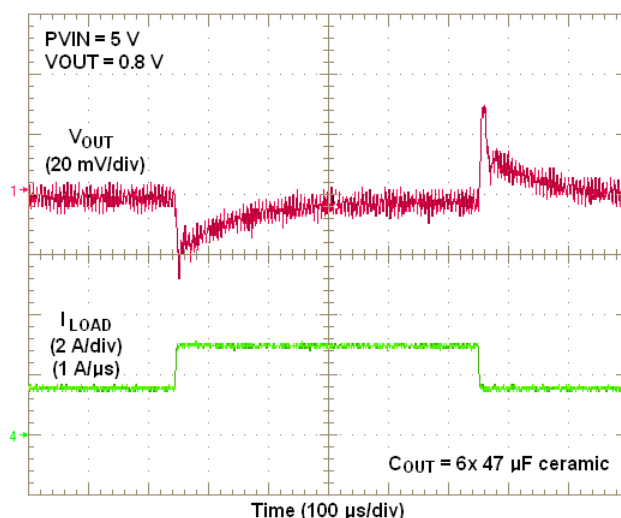
Figure 17. PVIN = 5V, VOUT = 0.8V, 1.5A Load Step
