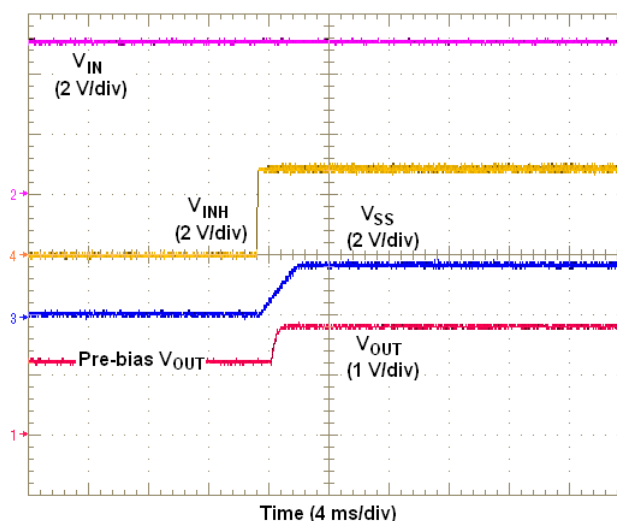
Figure 28. Start-up into Pre-bias
