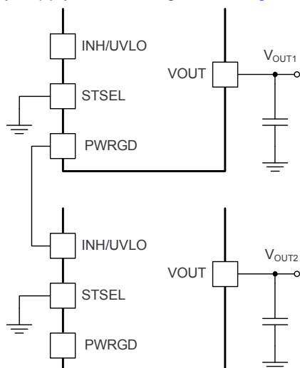
Figure 36. Sequencing Schematic
