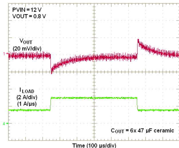
Figure 16. PVIN = 12V, VOUT = 0.8V, 1.5A Load Step
