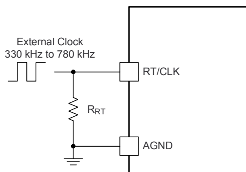
Figure 35. CLK/RT Configuration
