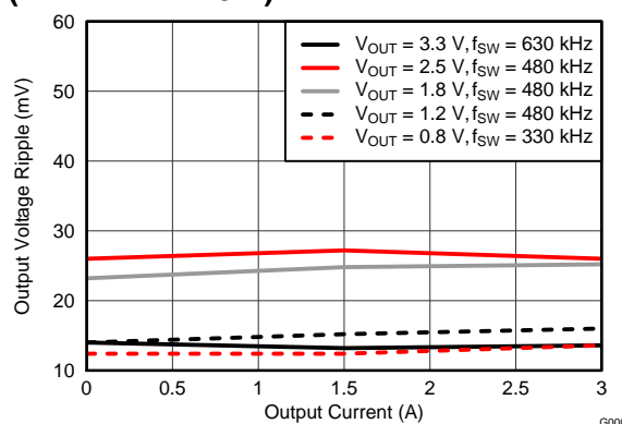
Figure 7. Voltage Ripple vs. Output Current
