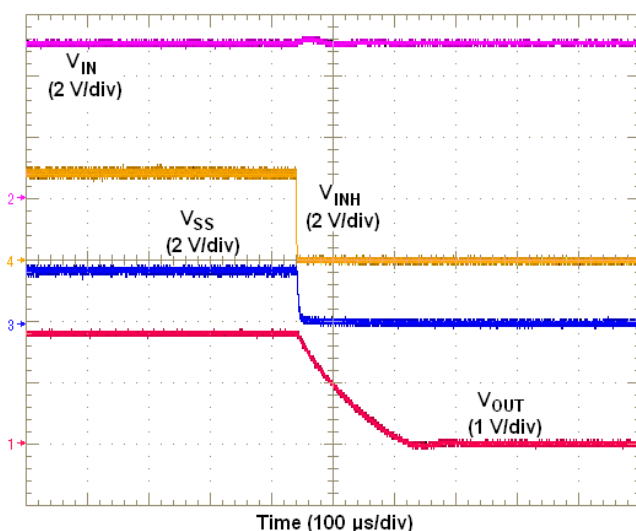
Figure 30. Inhibit Turn-Off
