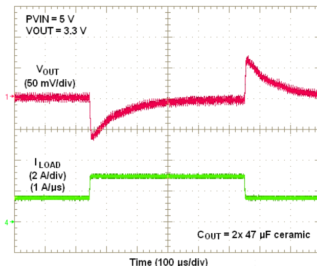
Figure 23. PVIN = 5V, VOUT = 3.3V, 1.5A Load Step
