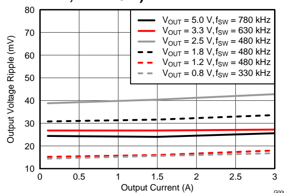
Figure 12. Voltage Ripple vs. Output Current
