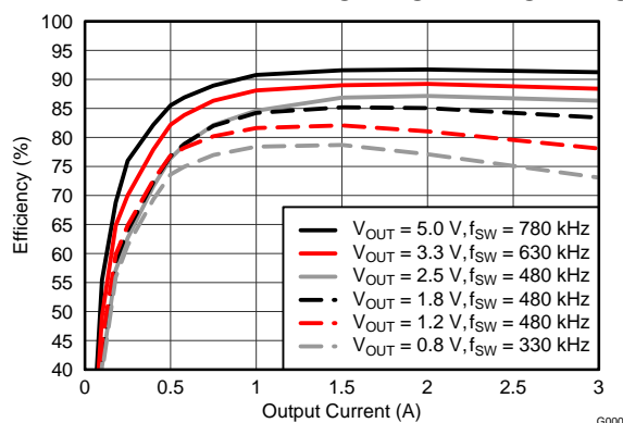
Figure 1. Efficiency vs. Output Current
