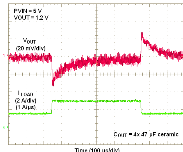
Figure 19. PVIN = 5V, VOUT = 1.2V, 1.5A Load Step
