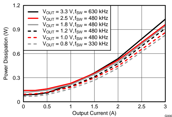
Figure 8. Power Dissipation vs. Output Current
