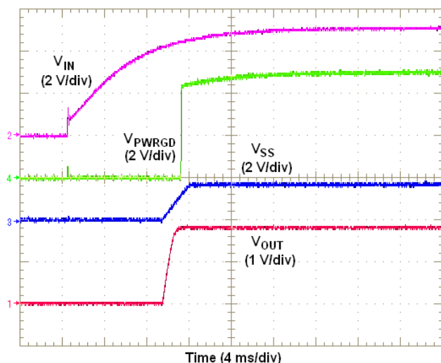
Figure 27. Start-Up Waveforms
