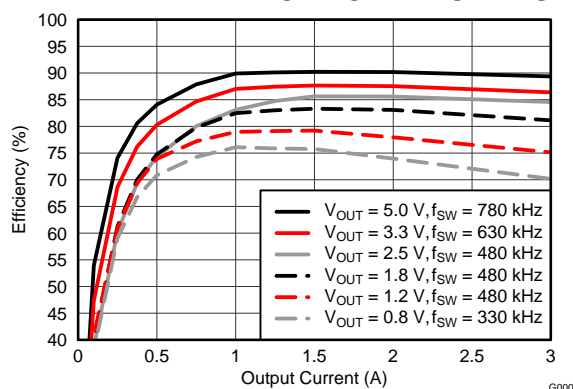
Figure 11. Efficiency vs. Output Current
