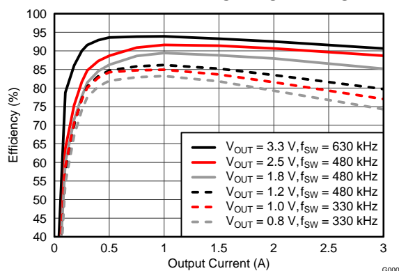
Figure 6. Efficiency vs. Output Current
