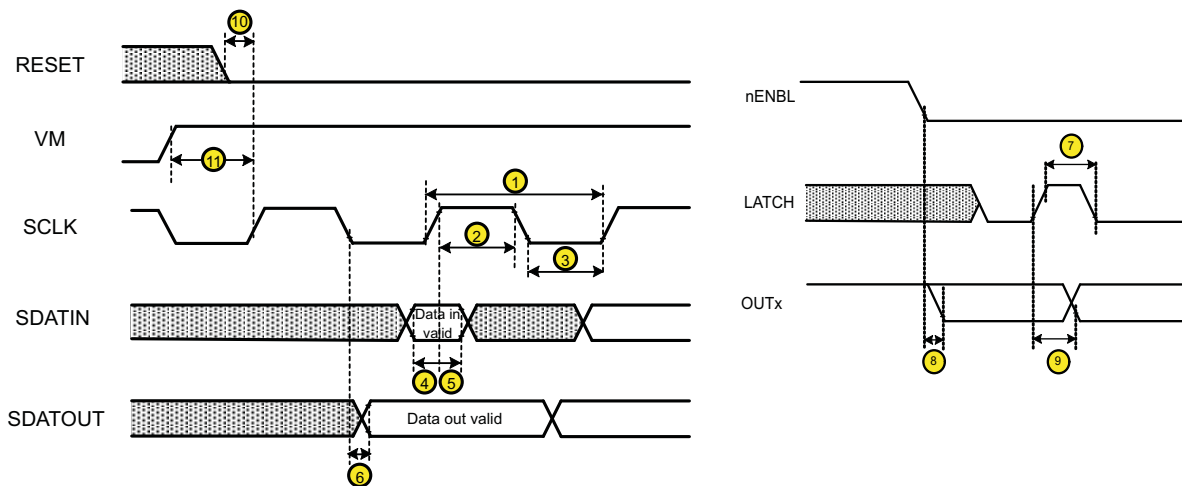
Figure 1. DRV8804 Timing Requirements
