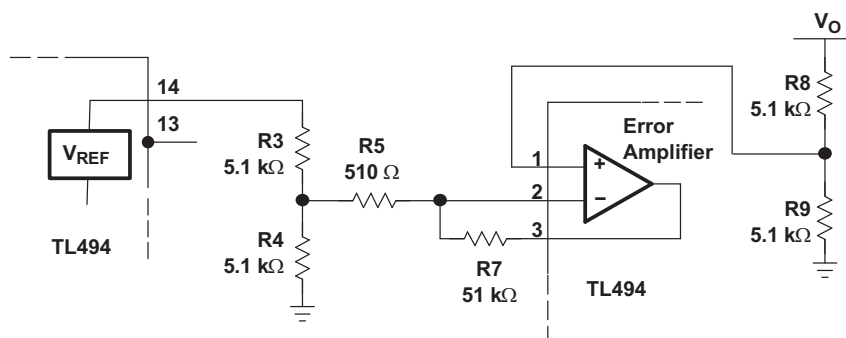
Figure 11. Error-Amplifier Section
