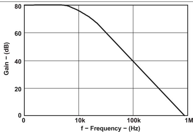
Figure 2. Amplifier Voltage Amplification vs Frequency
