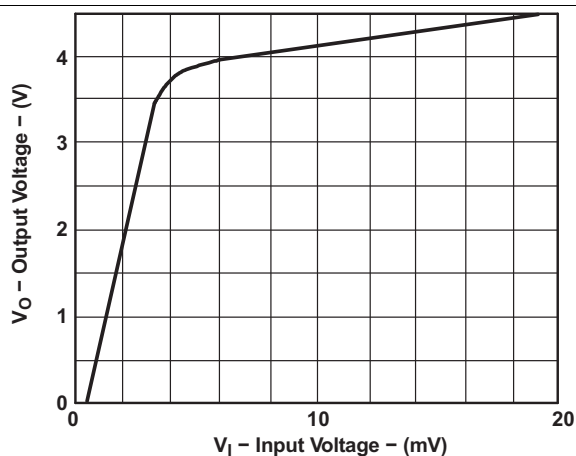
Figure 3. Error Amplifier Transfer Characteristics
