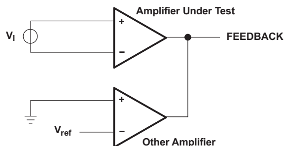
Figure 6. Amplifier Characteristics
