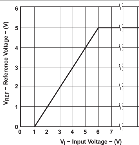
Figure 16. Reference Voltage vs Input Voltage
