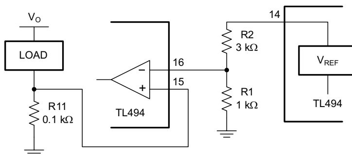
Figure 12. Current-Limiting Circuit
