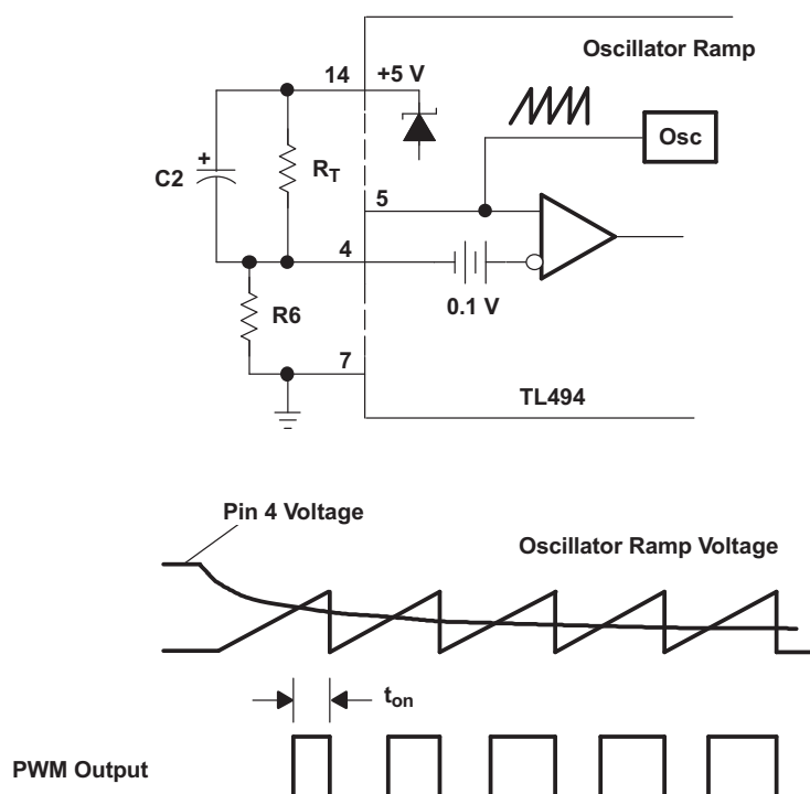
Figure 13. Soft-Start Circuit
