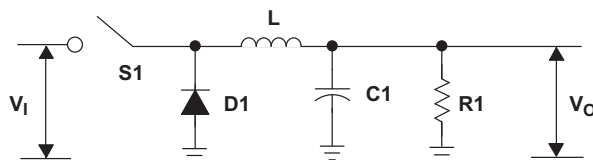
Figure 14. Switching Circuit
