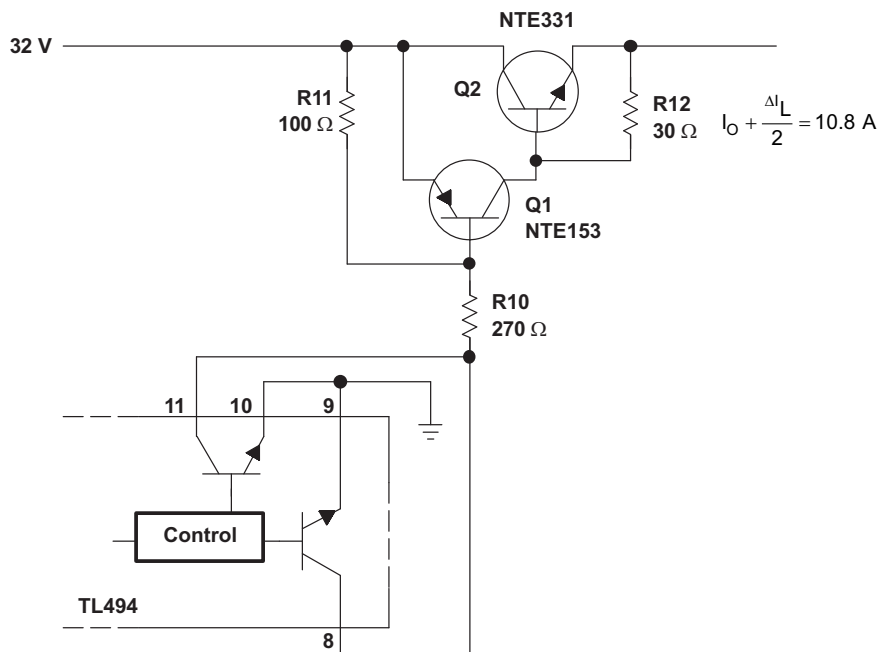
Figure 15. Power-Switch Section
