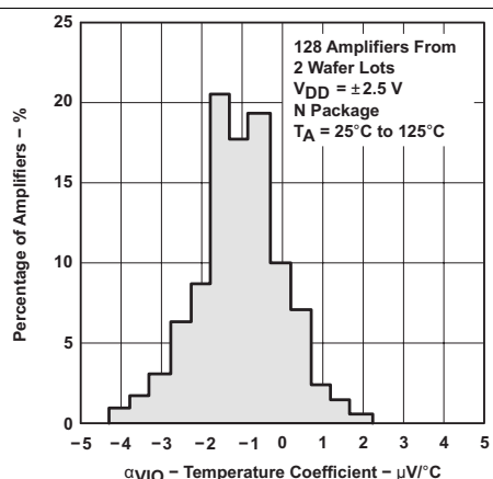
Figure 9. Distribution of TLC2274 vs Input Offset Voltage Temperature Coefficient
