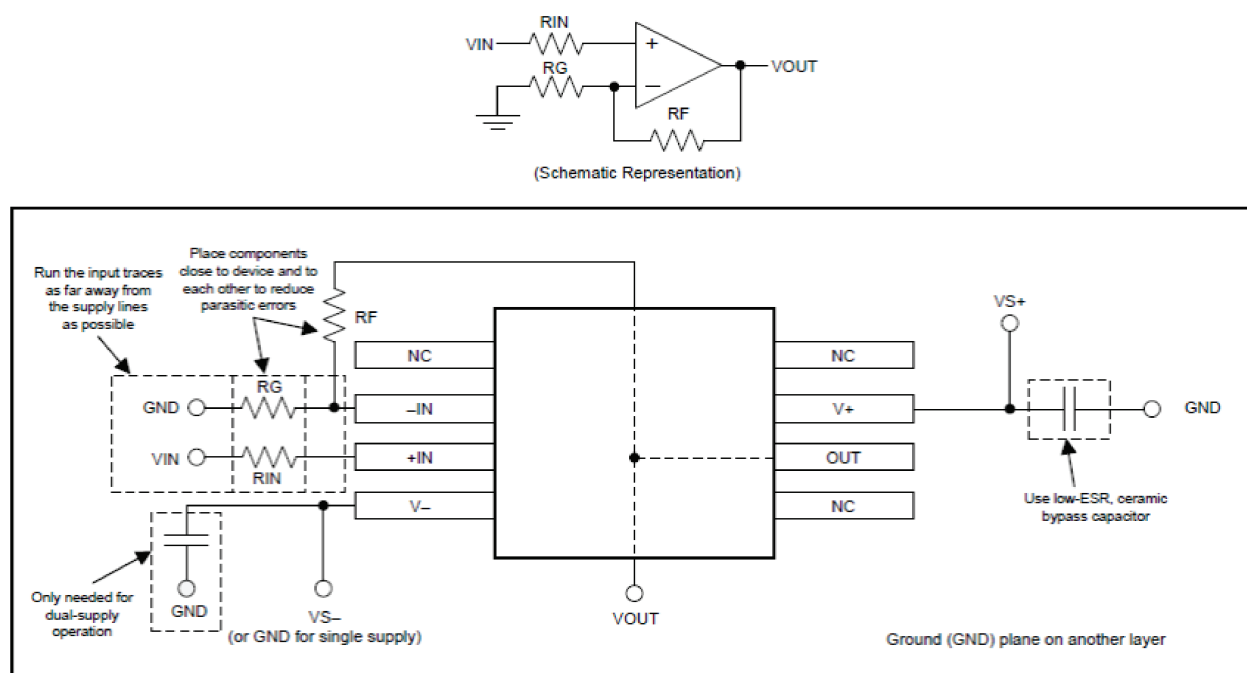
Figure 63. Layout Example
