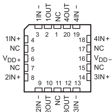
TLC2274 FK Package 20-Pin LCCC Top View
