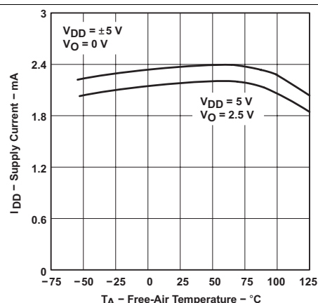
Figure 38. TLC2272 Supply Current vs Free-Air Temperature
