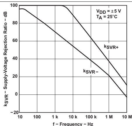
Figure 34. Supply-Voltage Rejection Ratio vs Frequency
