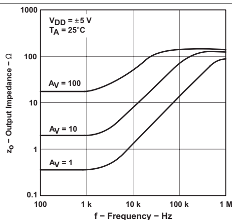
Figure 30. Output Impedance vs Frequency
