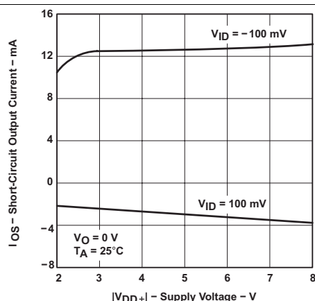
Figure 20. Short-Circuit Output Current vs Supply Voltage
