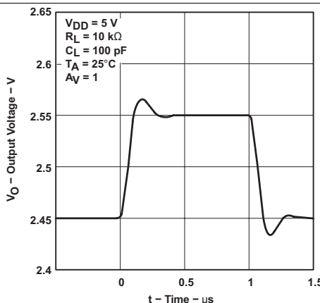
Figure 48. Voltage-Follower Small-Signal Pulse Response
