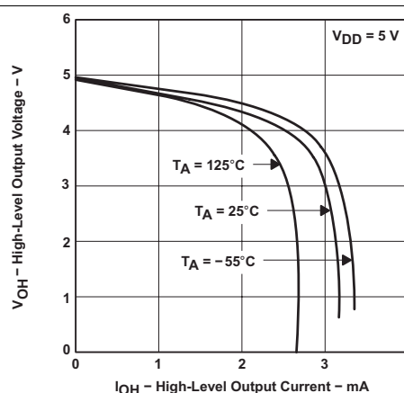
Figure 14. High-Level Output Voltage vs High-Level Output Current
