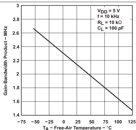
Figure 56. Gain-Bandwidth Product vs Free-Air Temperature
