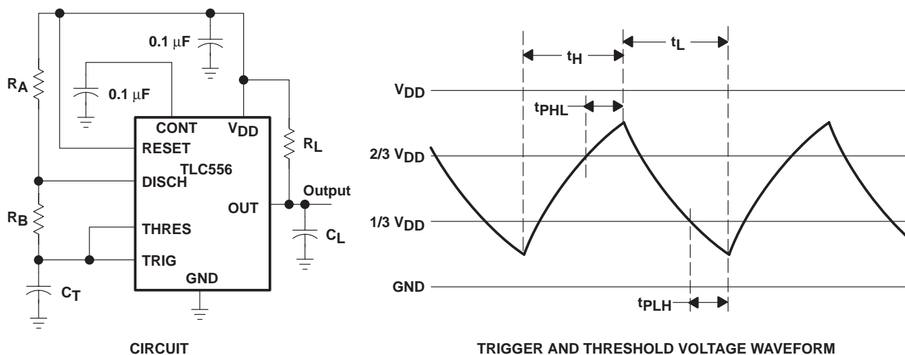
Figure 3. Astable Operation
