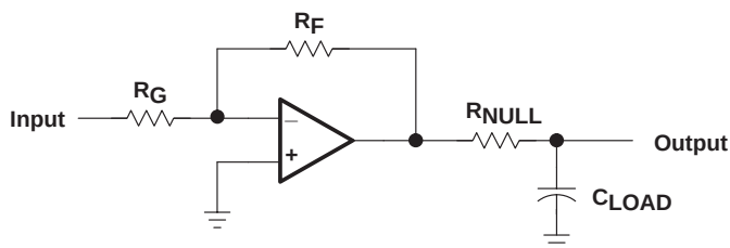
Figure 58. Driving a Capacitive Load
