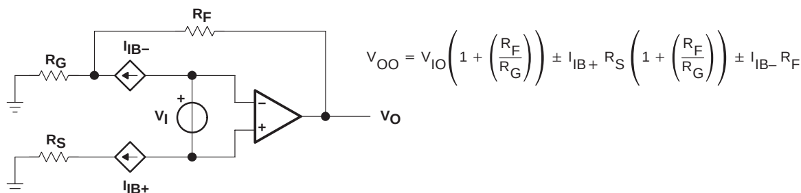
Figure 59. Output Offset Voltage Model
