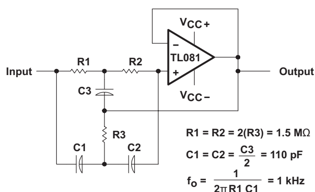
Figure 26. High-Q Notch Filter
