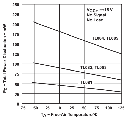
Figure 10. Total Power Dissipation vs Free-Air Temperature
