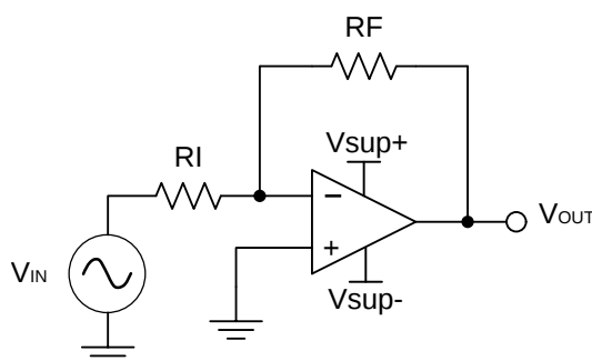
Figure 23. Schematic for Inverting Amplifier Application
