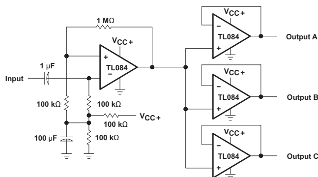
Figure 27. Audio-Distribution Amplifier
