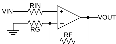
Figure 31. Operational Amplifier Schematic for Noninverting Configuration
