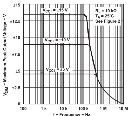
Figure 1. Maximum Peak Output Voltage vs Frequency
