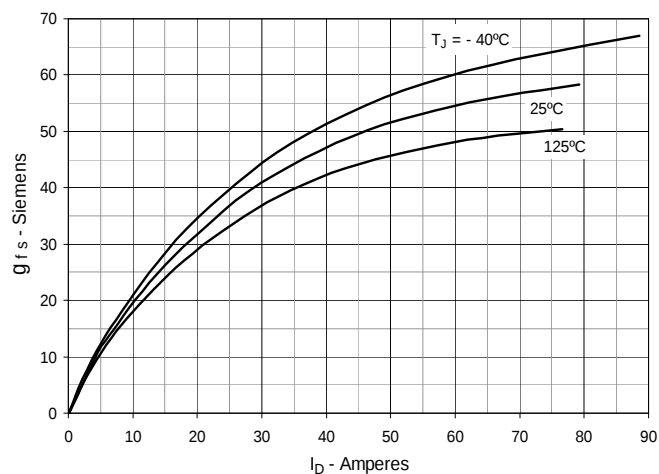
Fig. 8. Transconductance
