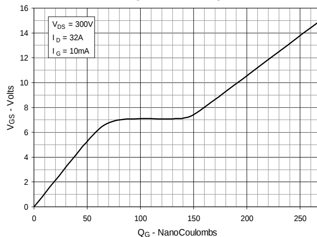
Fig. 10. Gate Charge
