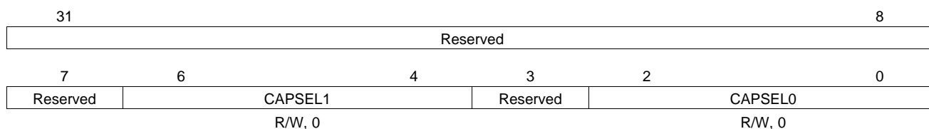
Figure 4-43. CFGRTI Register Bit Layout (0x4000 0014)
