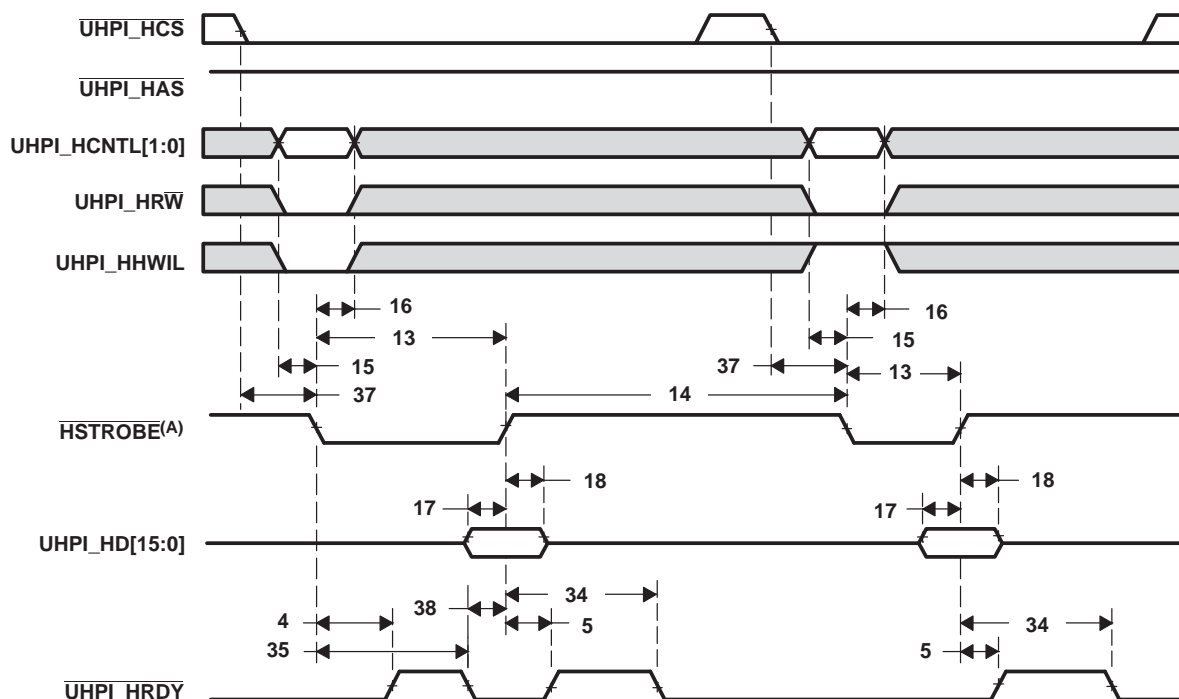
Figure 4-25. Multiplexed Read Timings With UHPI_HAS Held High
