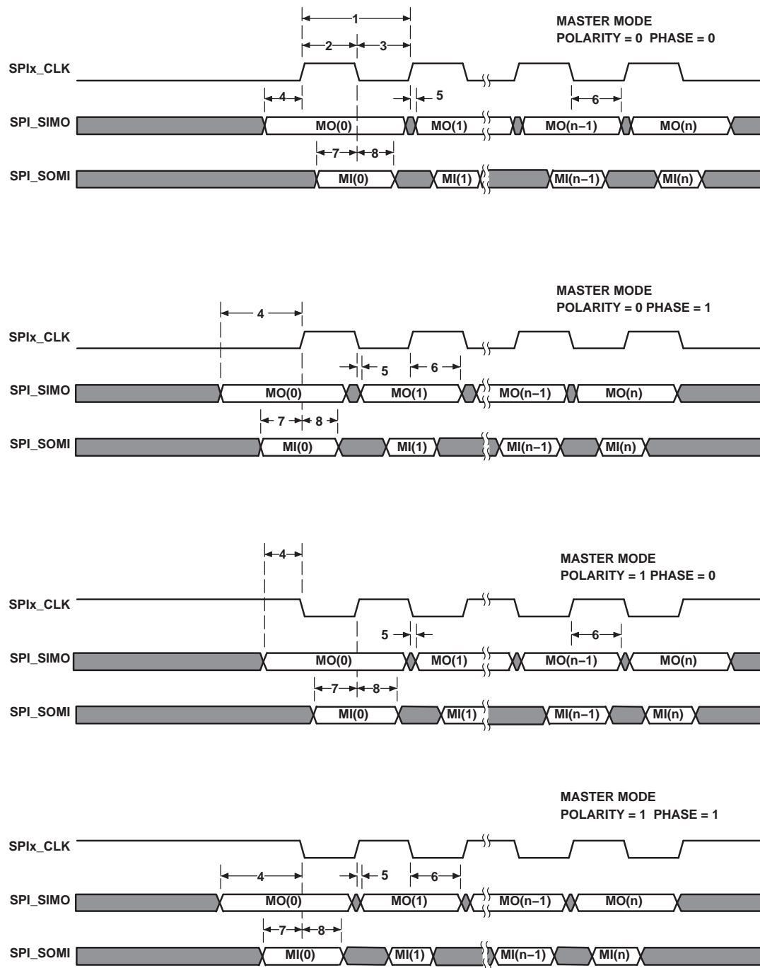
Figure 4-35. SPI Timings—Master Mode
