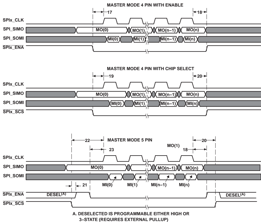
Figure 4-37. SPI Timings—Master Mode (4-Pin and 5-Pin)
