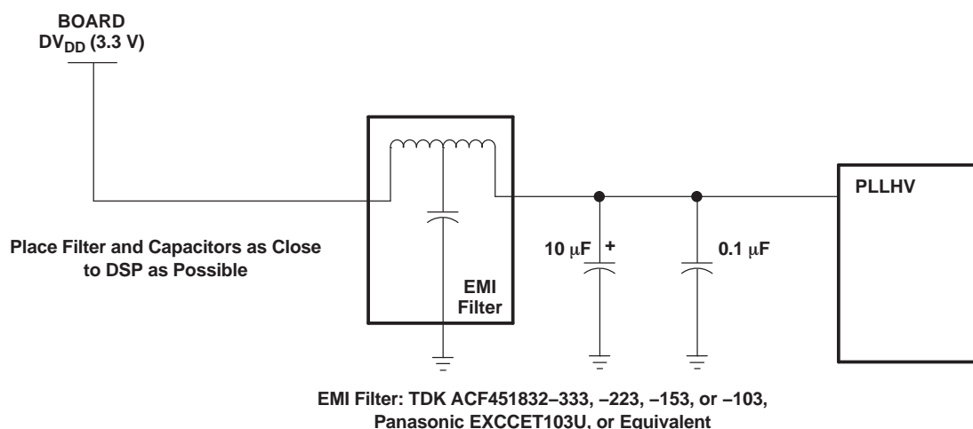
Figure 4-46. PLL Power Supply Filter
