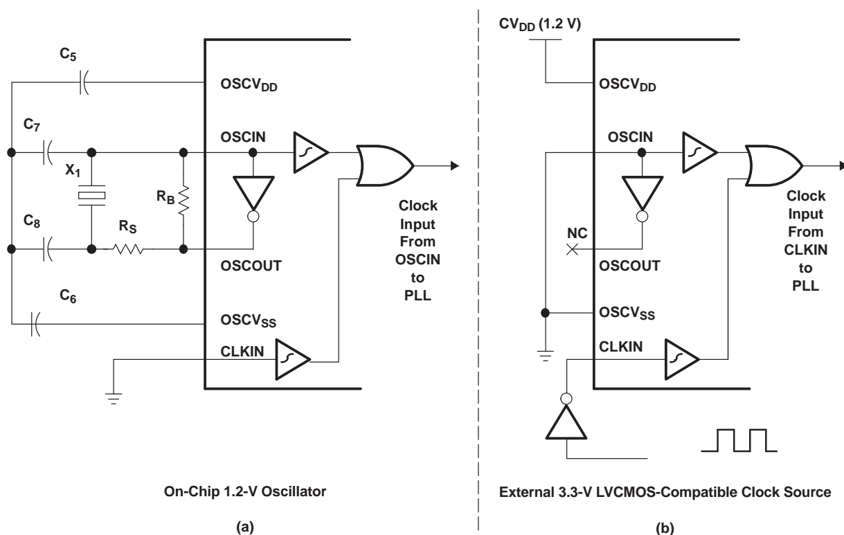
Figure 4-44. C672x Clock Input Options
