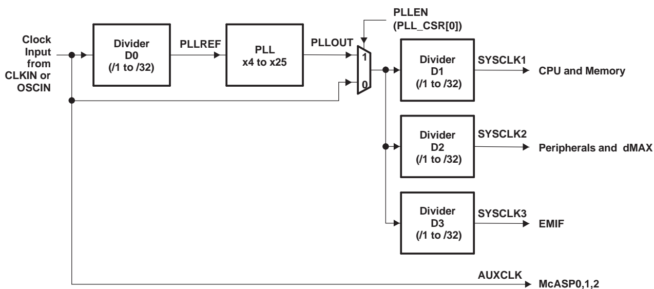
Figure 4-45. PLL Topology
