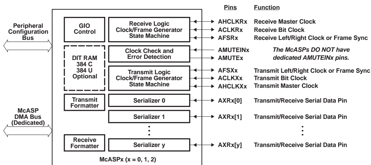
Figure 4-27. McASP Block Diagram
