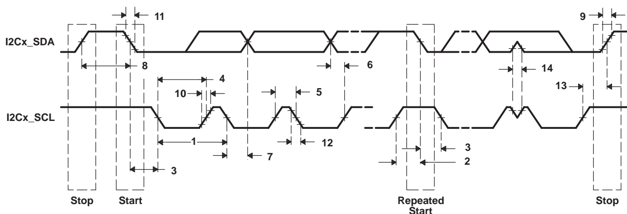
Figure 4-40. I2C Receive Timings
