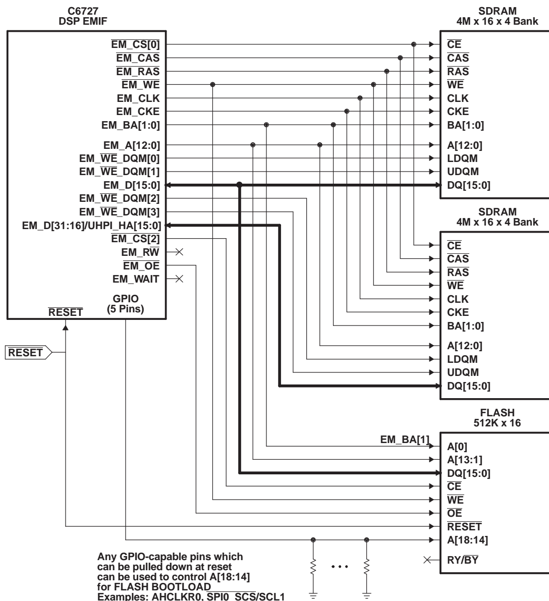
Figure 4-8. C6727 DSP 32-Bit EMIF Example
