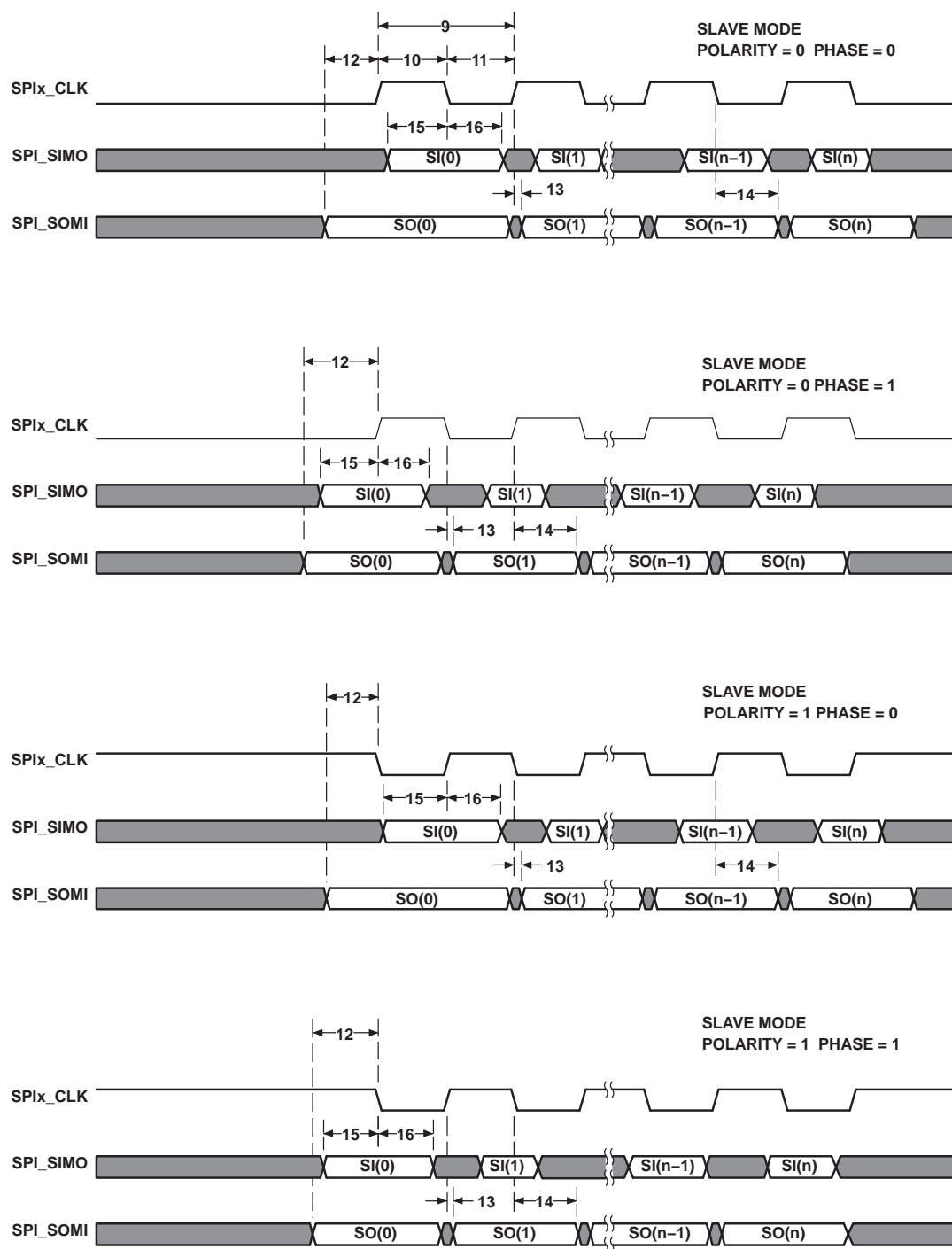
Figure 4-36. SPI Timings—Slave Mode
