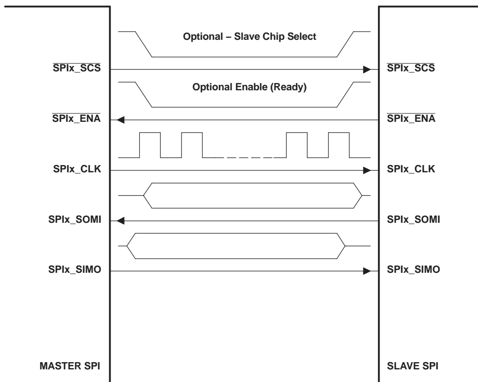
Figure 4-34. Illustration of SPI Master-to-SPI Slave Connection
