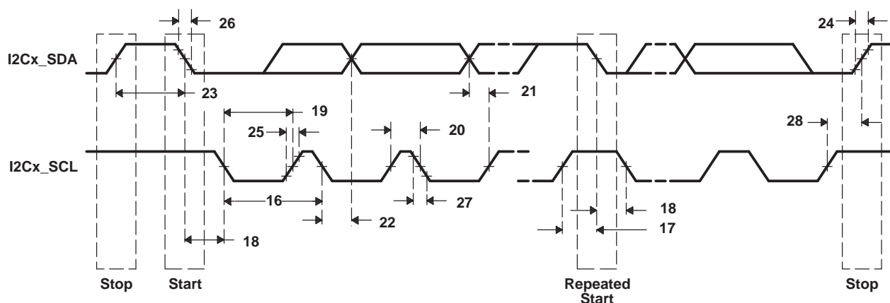
Figure 4-41. I2C Transmit Timings
