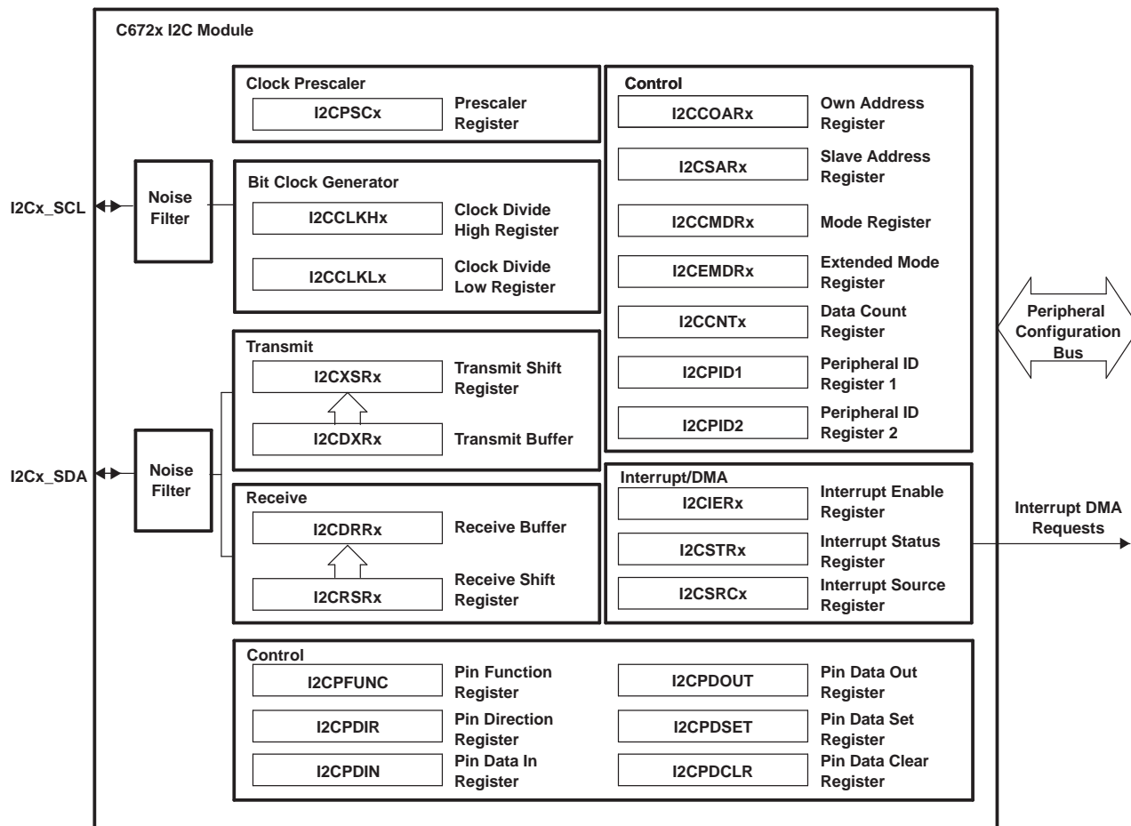
Figure 4-39. I2C Module Block Diagram
