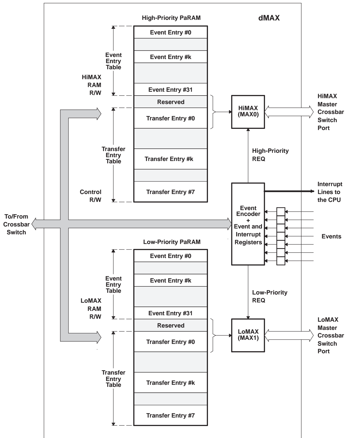
Figure 4-6. dMAX Controller Block Diagram
