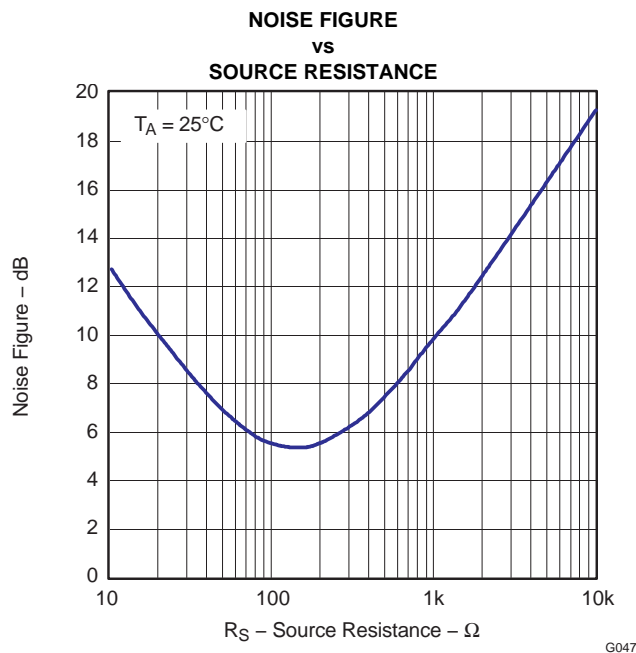
Figure 52. Noise Figure vs Source Resistance
