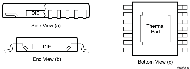
Figure 49. Views of Thermally Enhanced PWP Package
