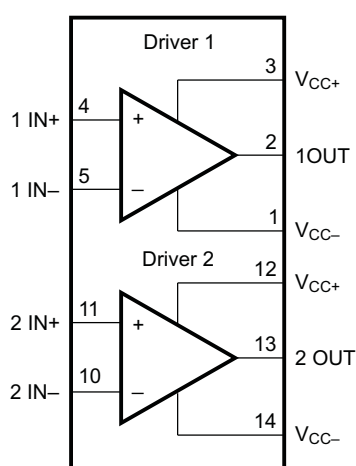
Functional Block Diagram
