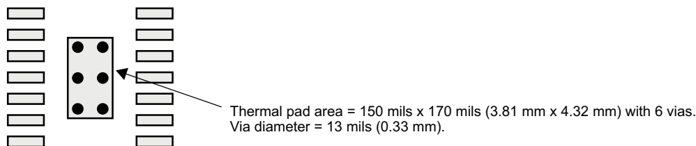
Figure 58. PowerPAD PCB Etch and Via Pattern Minimum Requirements
