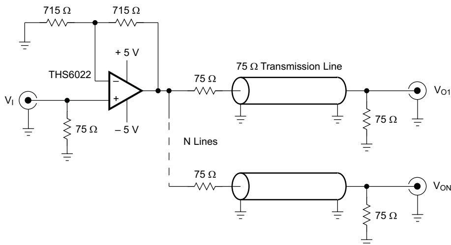
Figure 65. Video Distribution Amplifier Application
