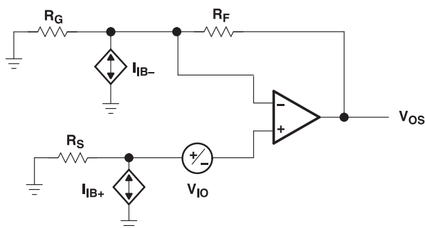
Figure 50. Output Offset Voltage Model
