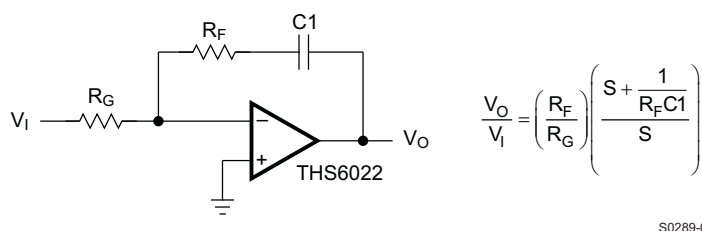
Figure 63. Inverting CFB Integrator
