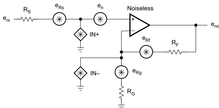
Figure 51. Noise Model
