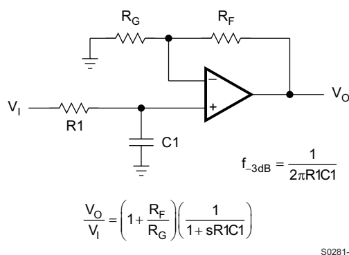
Figure 61. Single-Pole Low-Pass Filter
