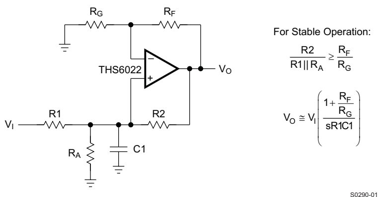
Figure 64. Noninverting CFB Integrator
