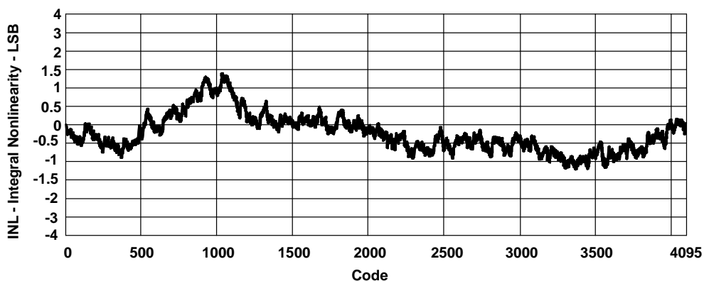
Figure 8. Integral Nonlinearity
