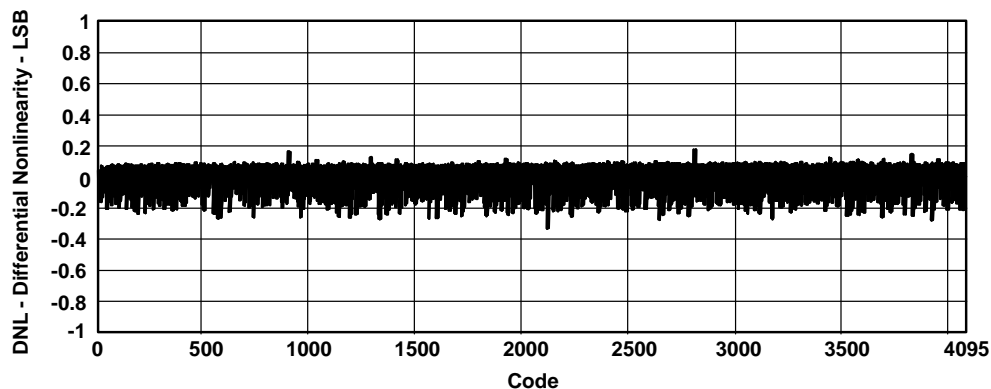
Figure 7. Differential Nonlinearity
