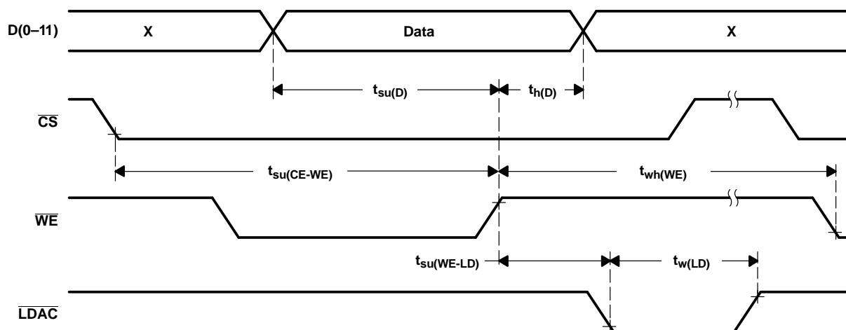
Figure 1. Timing Diagram
