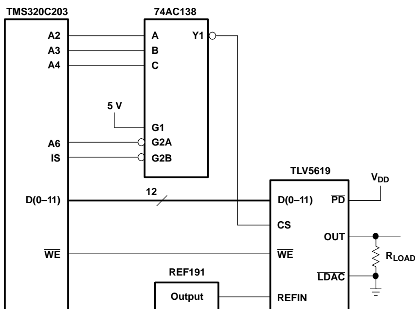
Figure 13. TLV5619 to TMS320C203 DSP Interface Connection
