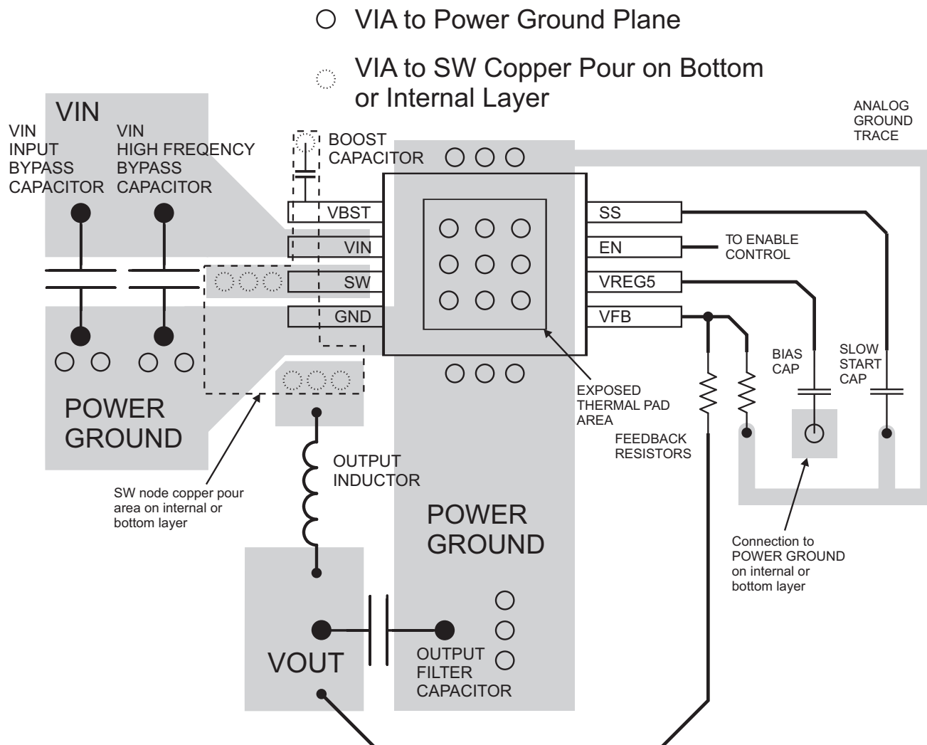
Figure 17. PCB Layout
