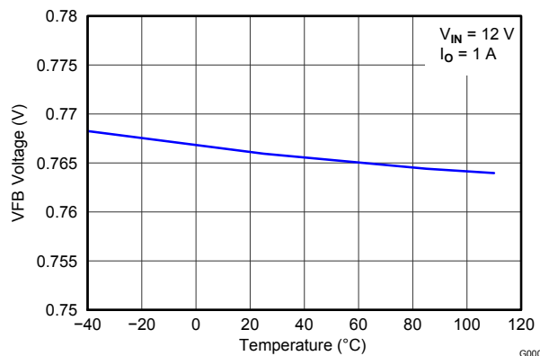
Figure 14. VFB VOLTAGE vs JUNCTION TEMPERATURE
