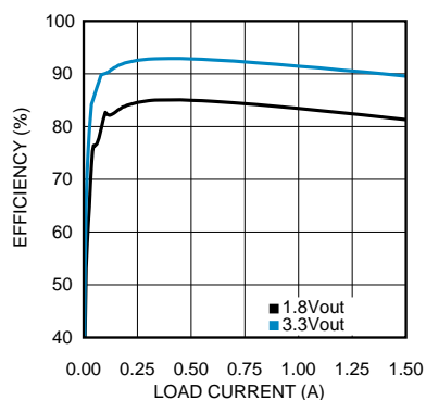
Efficiency vs Load Current - "X" V_{IN} = 5V
