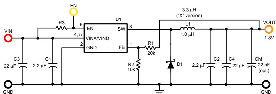
Figure 22. Typical Application Schematic
