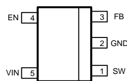
Figure 2. 5-Pin SOT-23 See Package Number DBV (R-PDSO-G5)
