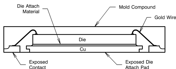
Internal WSON Connection
