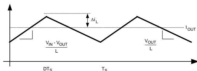
Figure 23. Inductor Current
