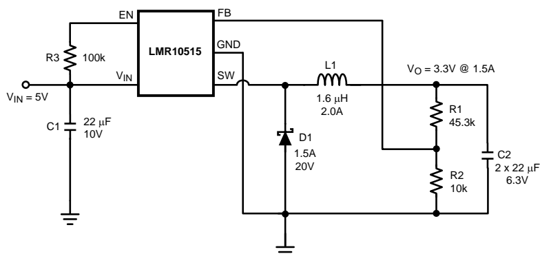
Figure 27. LMR10515Y (3MHz): V_{IN} = 5V , V_O = 3.3V @ 1.5A
