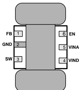
Figure 24. 6-Lead WSON PCB Dog Bone Layout
