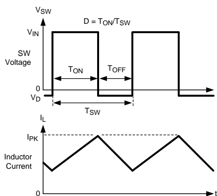
Figure 21. Typical Waveforms
