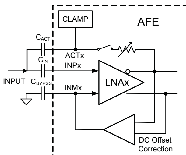
Figure 59. AFE5808A LNA With DC Offset Correction Circuit
