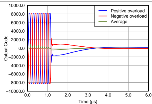
Figure 53. Pulse Inversion Asymmetrical Positive Input
