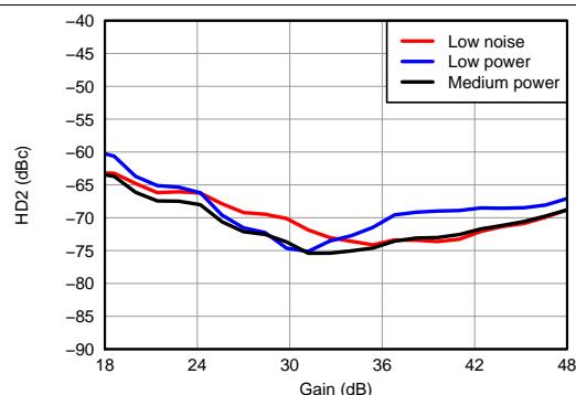
Figure 41. HD2 vs Gain
