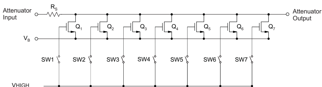
Figure 61. Simplified Voltage Controlled Attenuator (Digital Structure)
