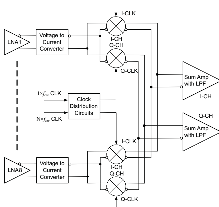
Figure 63. Simplified Block Diagram of CW Path
