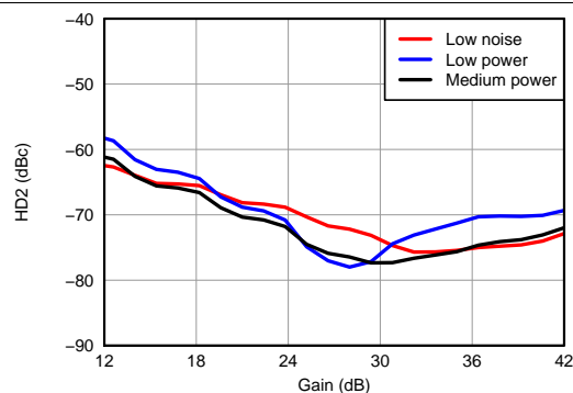
Figure 39. HD2 vs Gain
