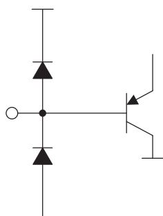
Figure 72. Equivalent Circuits of V_{CNTLP/M}
