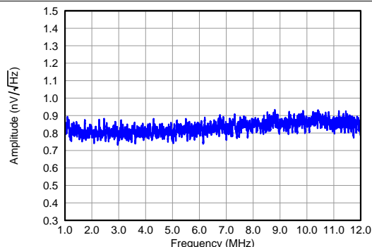
Figure 27. IRN and Low-Noise Mode
