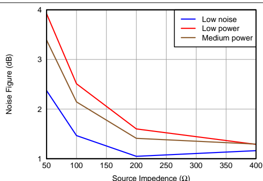
Figure 36. Noise Figure vs Power Modes Without Termination
