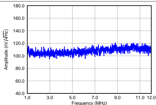
Figure 26. ORN and Low-Power Mode
