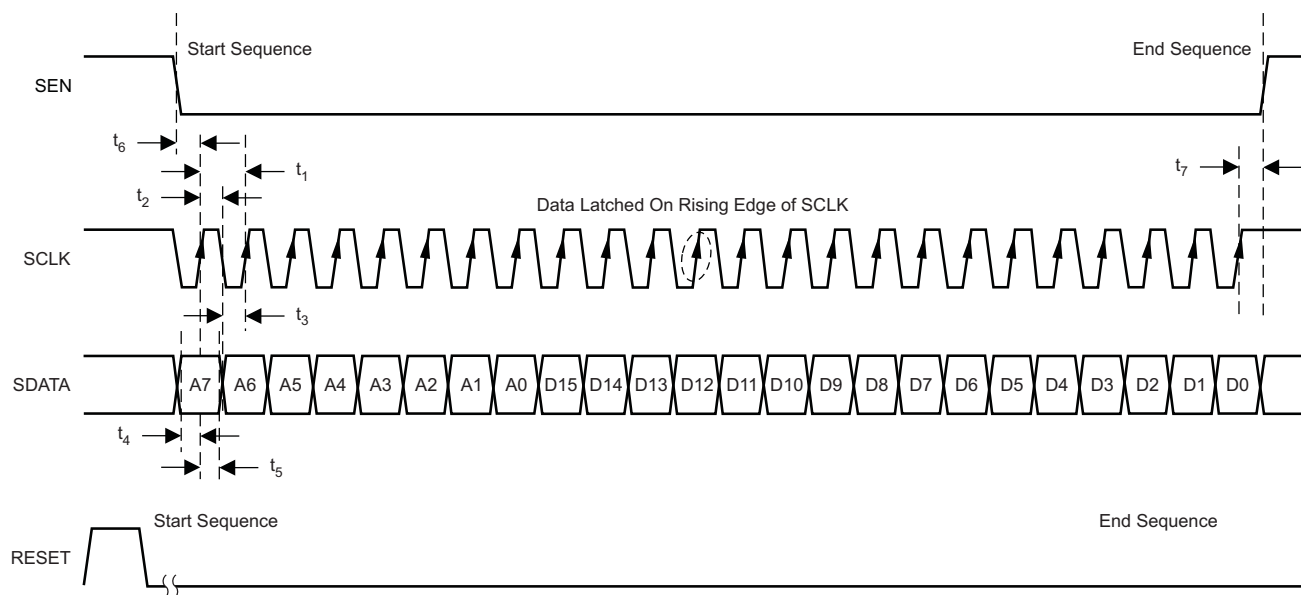
Figure 77. SPI Timing
