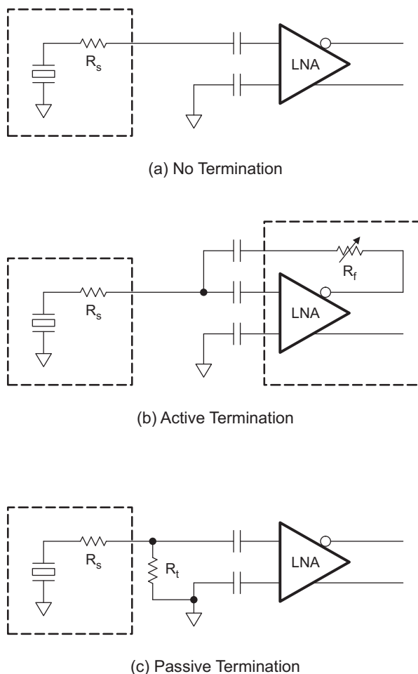
Figure 82. Termination Configurations
