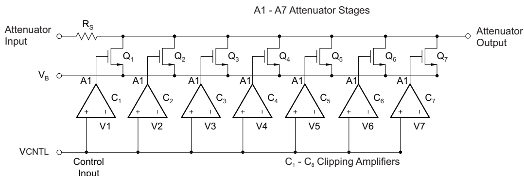
Figure 60. Simplified Voltage Controlled Attenuator (Analog Structure)
