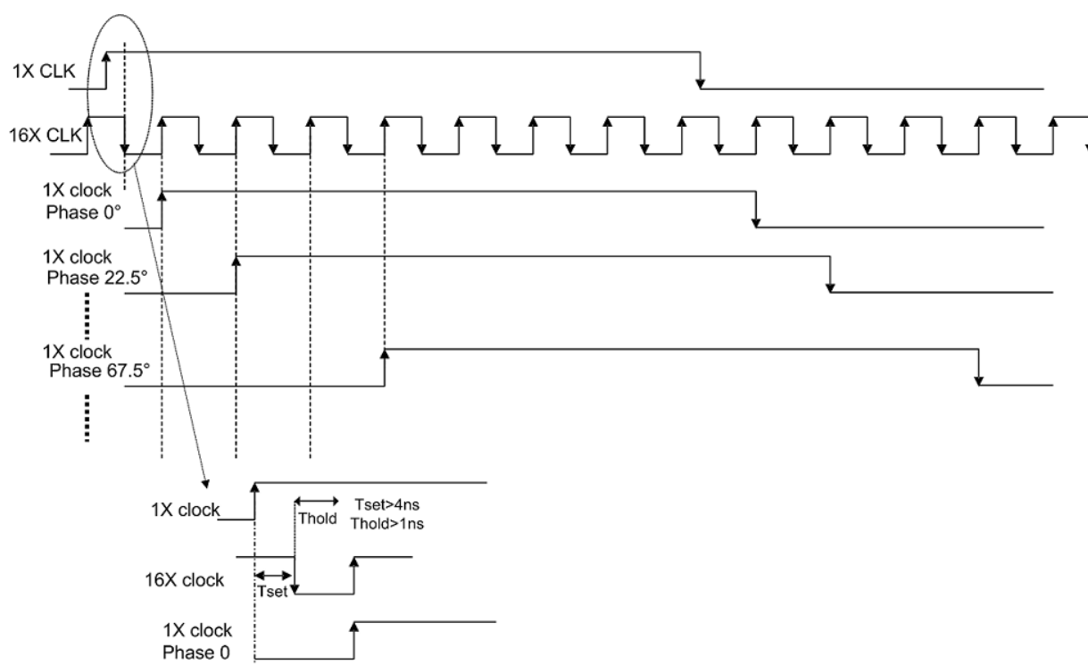
Figure 67. 1x and 16x CW Clock Timing
