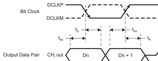
Figure 1. LVDS Timing Diagrams
