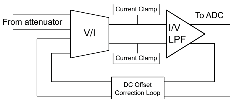
Figure 62. Simplified Block Diagram of PGA
