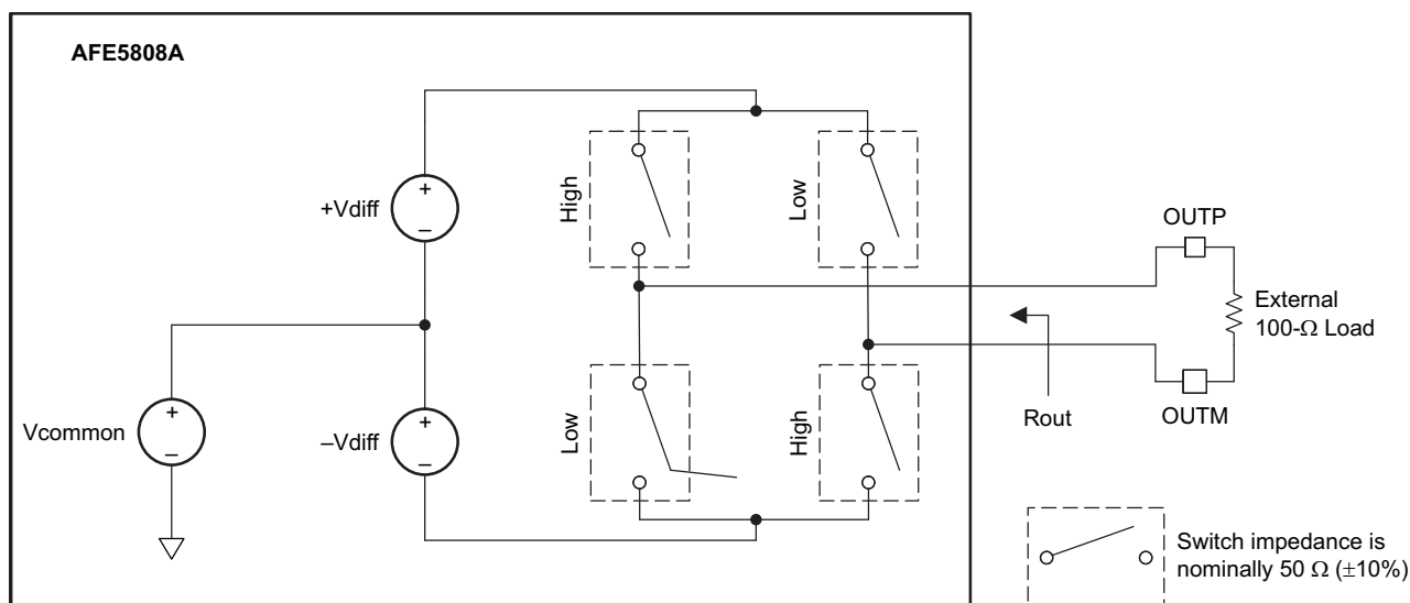
Figure 75. Equivalent Circuits of LVDS Outputs
