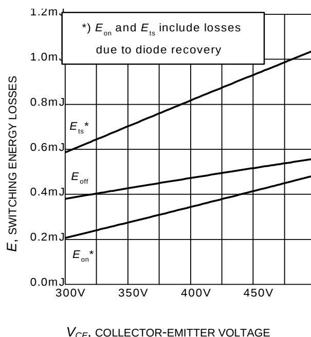
Figure 16. Typical switching energy losses as a function of collector emitter voltage (inductive load, T_J = 175^\circ\text{C} , V_{GE} = 0/15\text{V} , I_C = 15\text{A} , r_G = 15\Omega , Dynamic test circuit in Figure E)
