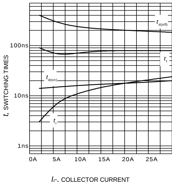
Figure 9. Typical switching times as a function of collector current (inductive load, T_J=175^{\circ}\text{C} , V_{CE} = 400\text{V} , V_{GE} = 0/15\text{V} , r_G = 15\Omega , Dynamic test circuit in Figure E)
