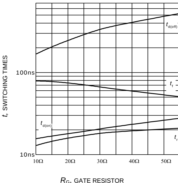
Figure 10. Typical switching times as a function of gate resistor (inductive load, T_J = 175^{\circ}\text{C} , V_{CE}= 400\text{V} , V_{GE} = 0/15\text{V} , I_C = 15\text{A} , Dynamic test circuit in Figure E)
