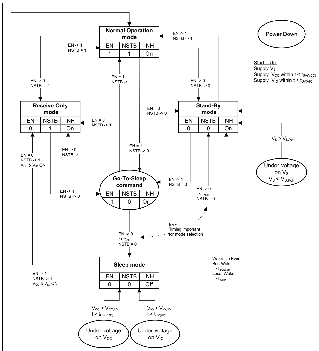
Figure 4 Operation Modes
