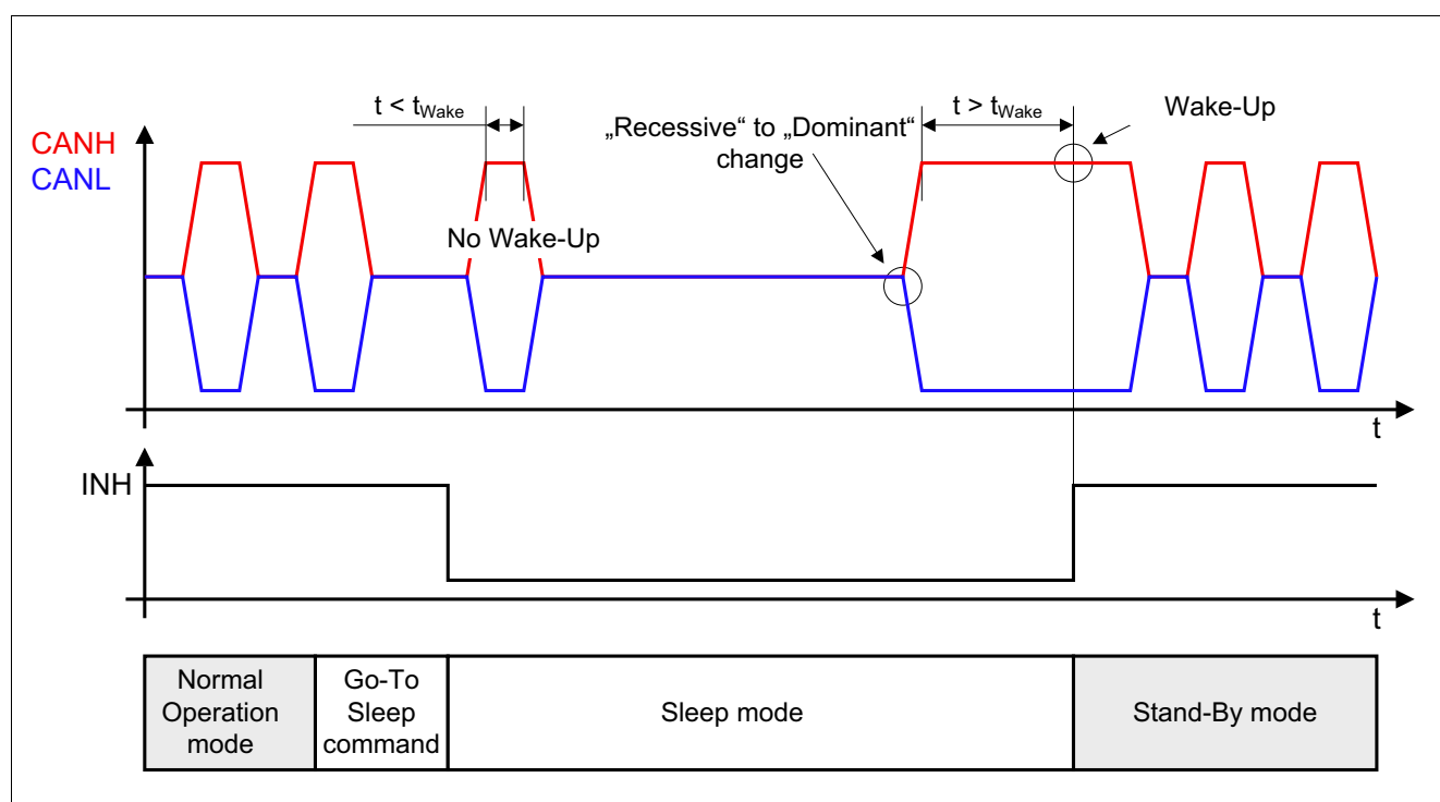
Figure 6 Remote Wake-Up
