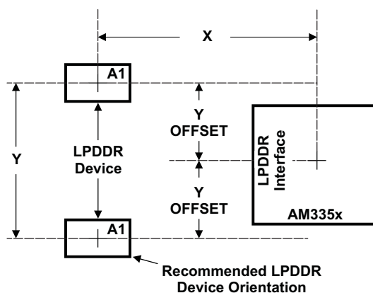
Figure 7-34. AM335x Device and LPDDR Device Placement
