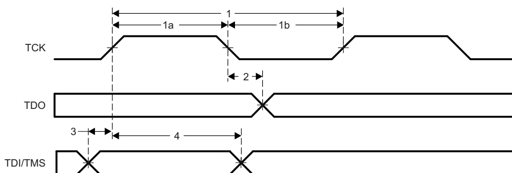
Figure 7-70. JTAG Timing
