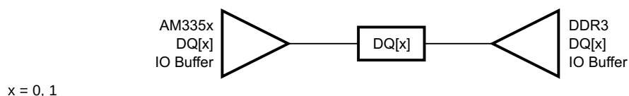
Figure 7-63. DQ[x] Topology
