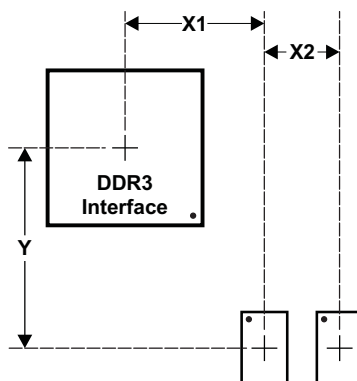
Figure 7-50. Placement Specifications
