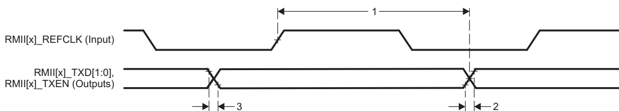
Figure 7-12. RMII[x]_TXD[1:0], RMII[x]_TXEN Timing - RMII Mode
