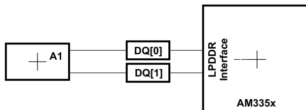
Figure 7-37. DQS[x] and DQ[x] Routing and Topology
