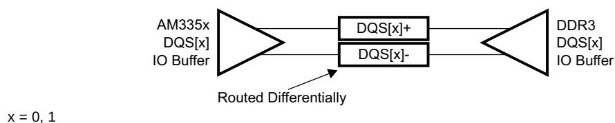
Figure 7-62. DQS[x] Topology
