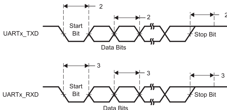
Figure 7-114. UART Timings
