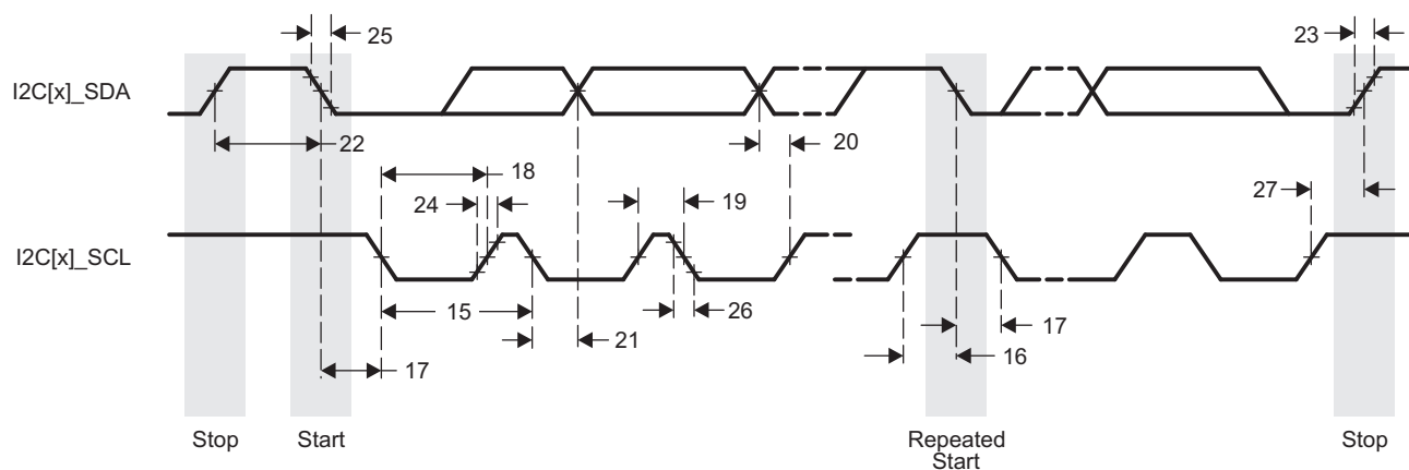
Figure 7-69. I²C Transmit Timing
