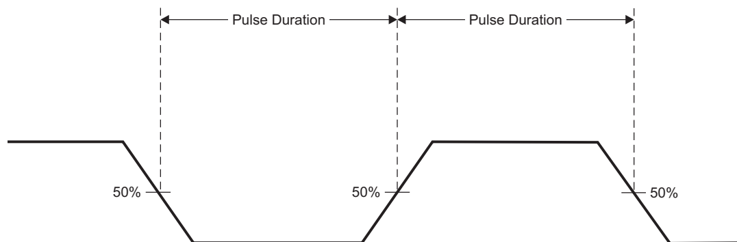
Figure 7-115. UART IrDA Pulse Parameters
