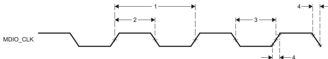
Figure 7-4. MDIO_CLK Timing
