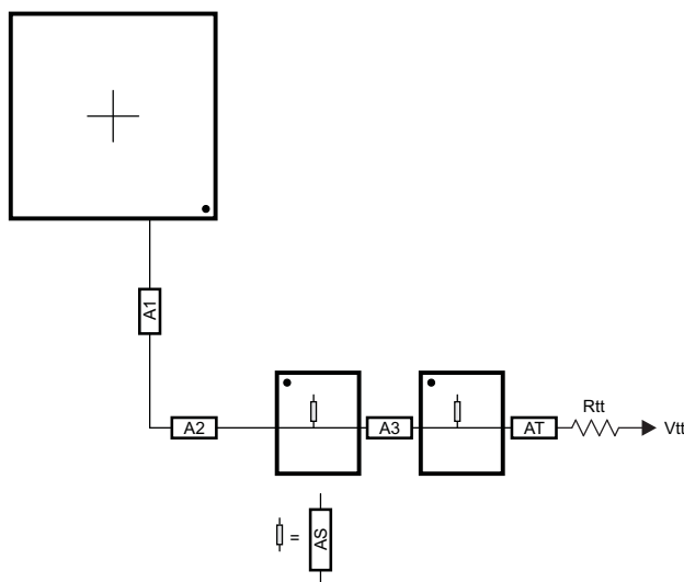
Figure 7-55. ADDR_CTRL Routing for Two Single-Side DDR3 Devices
