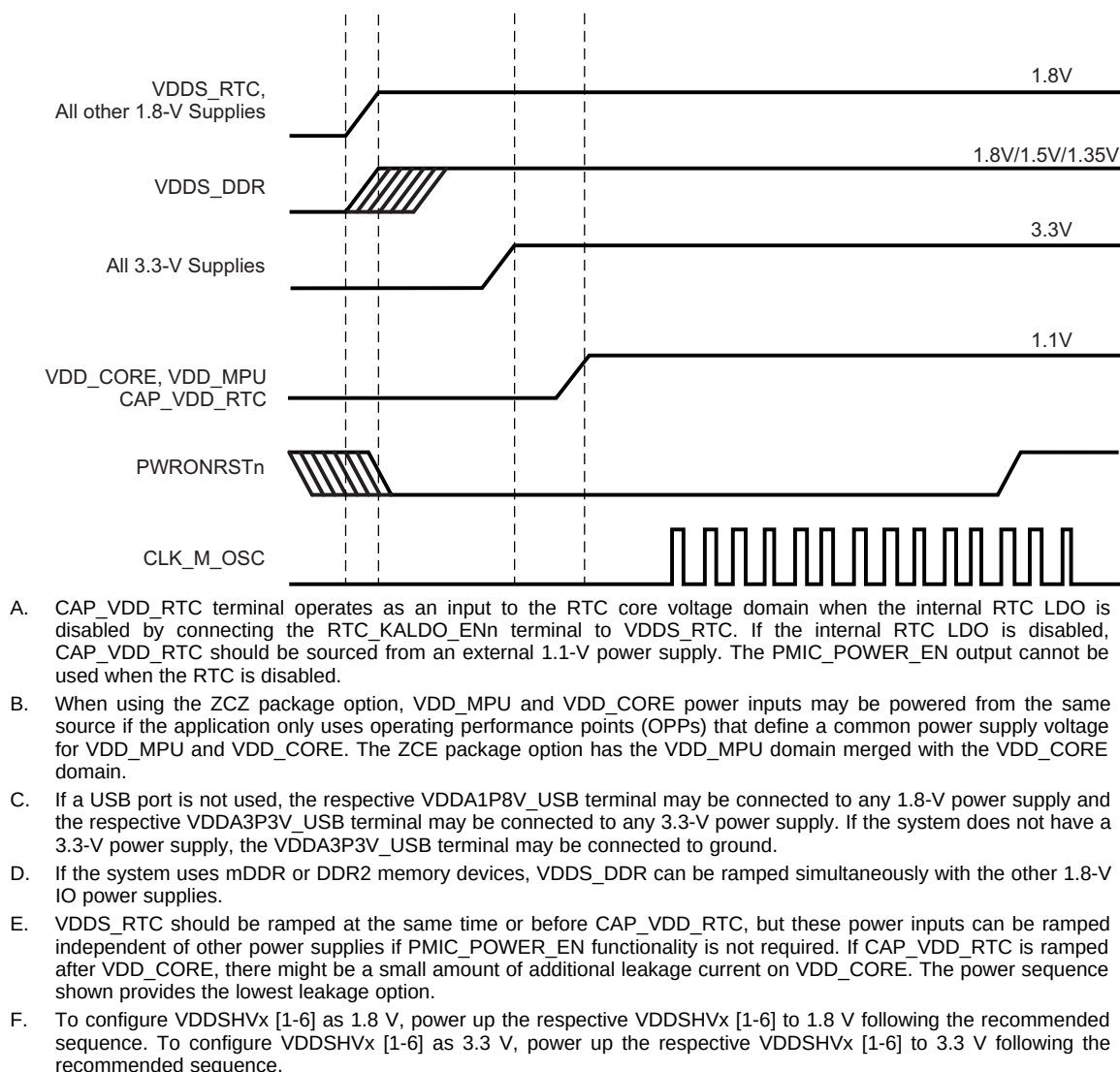
Figure 6-6. Power-Supply Sequencing with RTC Feature Disabled
