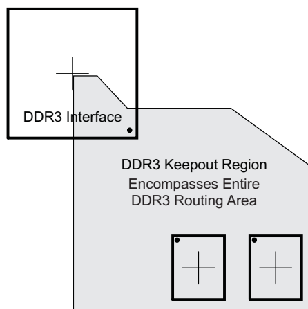
Figure 7-51. DDR3 Keepout Region
