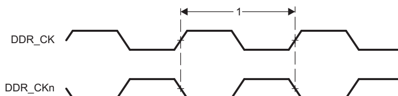
Figure 7-46. DDR3 Memory Interface Clock Timing
