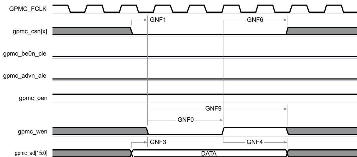
Figure 7-31. GPMC and NAND Flash—Data Write Cycle
