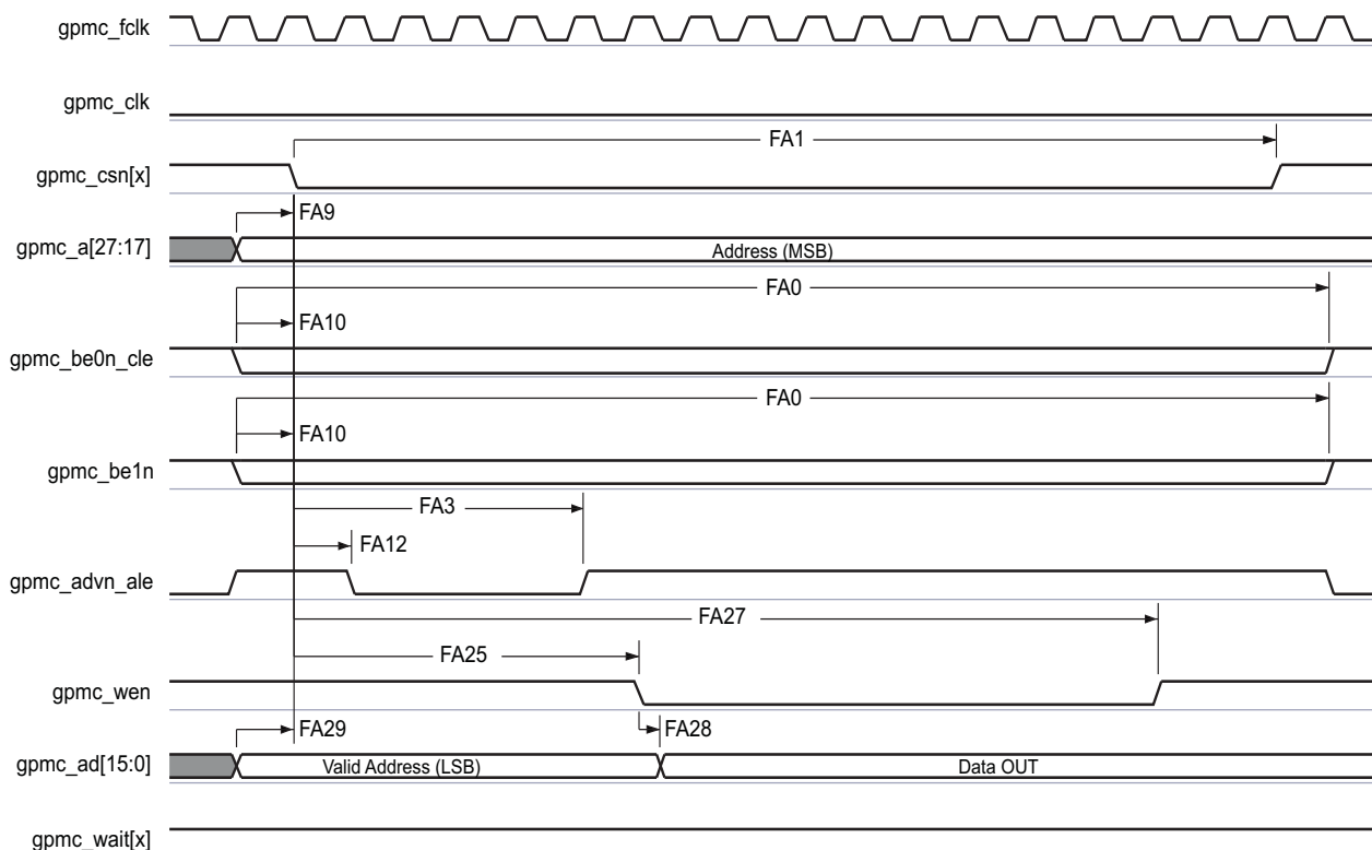
Figure 7-27. GPMC and Multiplexed NOR Flash—Asynchronous Write—Single Word
