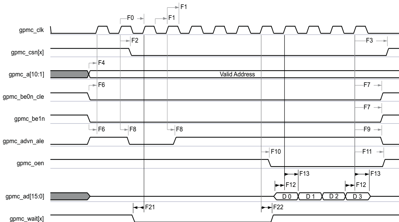
Figure 7-18. GPMC and NOR Flash—Synchronous Burst Read—4x16-bit (GpmcFCLKDivider = 0)
