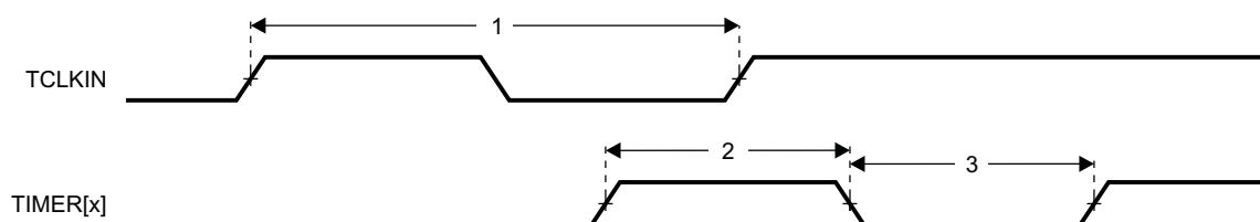
Figure 7-2. Timer Timing
