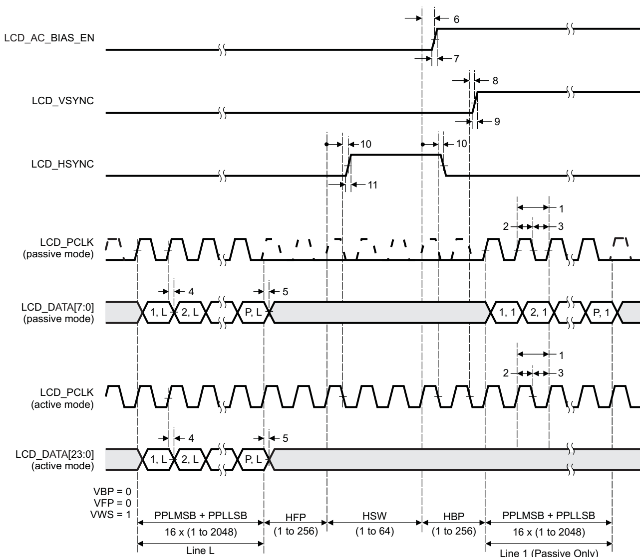
Figure 7-84. LCD Raster-Mode Control Signal Activation
