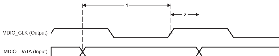
Figure 7-106. PRU-ICSS MDIO_DATA Timing - Input Mode
