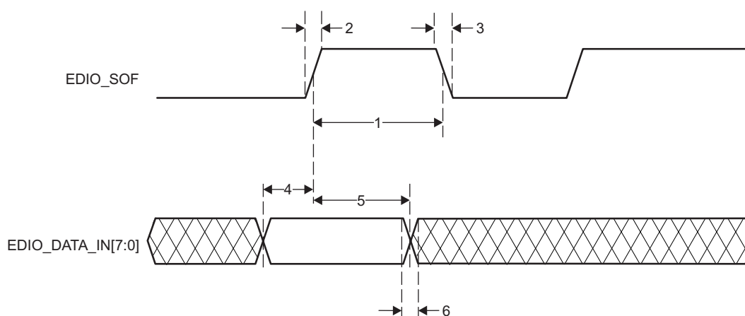
Figure 7-104. PRU-ICSS ECAT Input Validated with SOF
