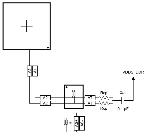
Figure 7-60. CK Routing for One DDR3 Device
