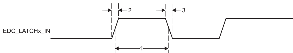
Figure 7-105. PRU-ICSS ECAT LATCHx_IN Timing
