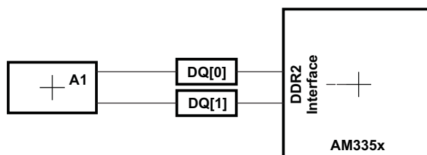
Figure 7-45. DQS[x] and DQ[x] Routing and Topology
