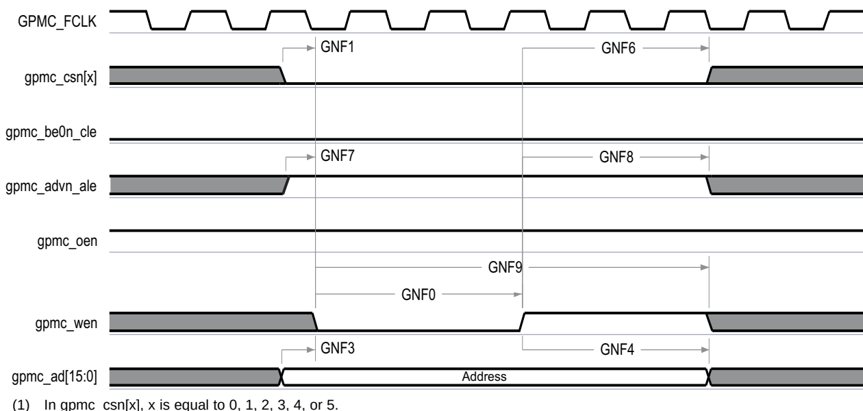
Figure 7-29. GPMC and NAND Flash—Address Latch Cycle
