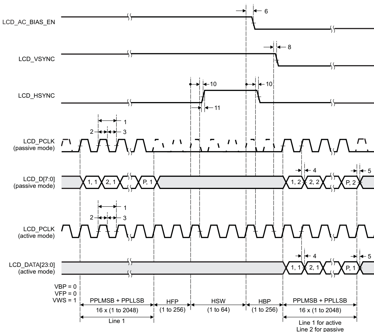
Figure 7-85. LCD Raster-Mode Control Signal Deactivation
