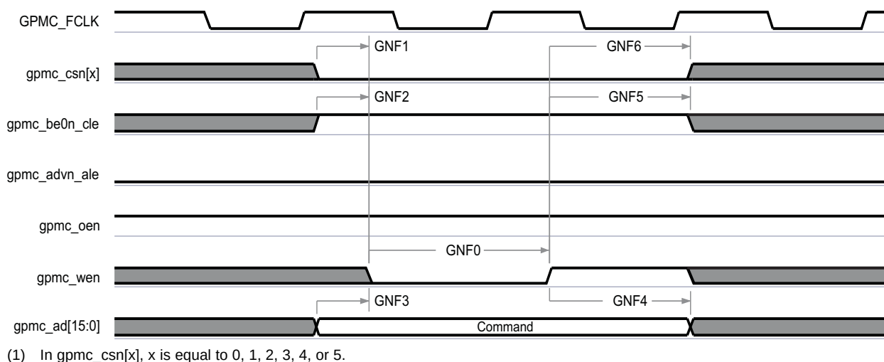
Figure 7-28. GPMC and NAND Flash—Command Latch Cycle
