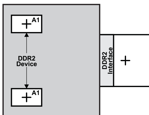
Figure 7-42. DDR2 Keepout Region
