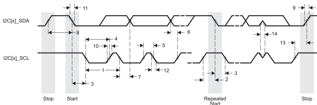
Figure 7-68. I²C Receive Timing
