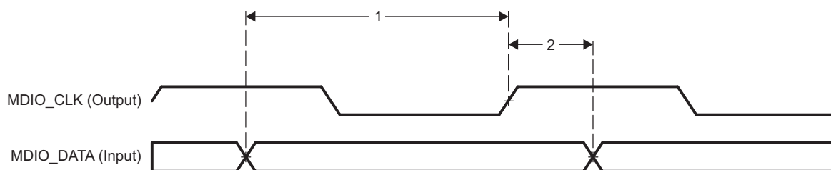
Figure 7-3. MDIO_DATA Timing - Input Mode
