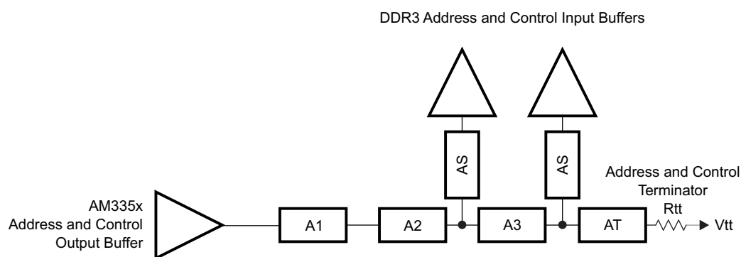
Figure 7-53. ADDR_CTRL Topology for Two DDR3 Devices
