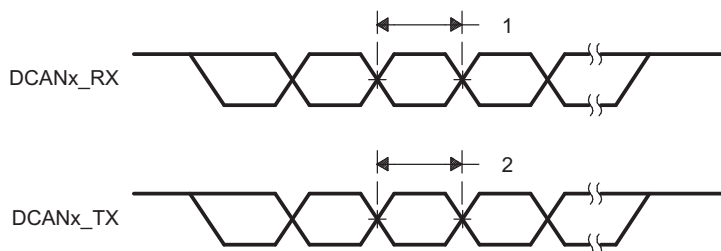
Figure 7-1. DCANx Timings
