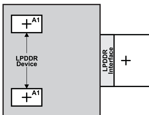
Figure 7-35. LPDDR Keepout Region
