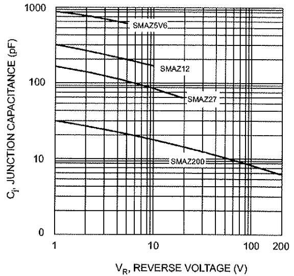
Fig. 2 Junction Capacitance vs Reverse Voltage
