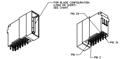
75556-5100 SHOWN (W/O PEG)
