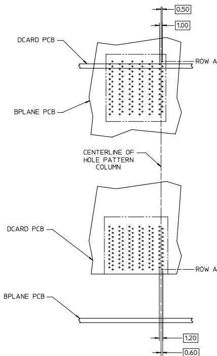
36 PAIR ORTHOGONAL MIDPLANE NODE (USES TWO 6 COLUMN I-TRAC HEADERS)
