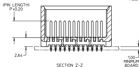
SECTION Z-Z
