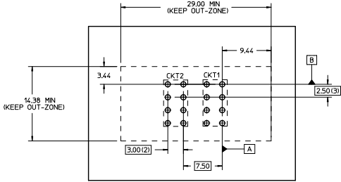
RECOMMENDED PCB LAYOUT AND KEEP-OUT ZONE
