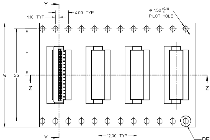
DETAIL 1
