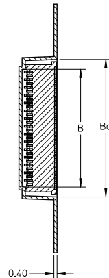
SECTION Y-Y
