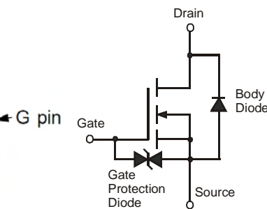
Equivalent Circuit
