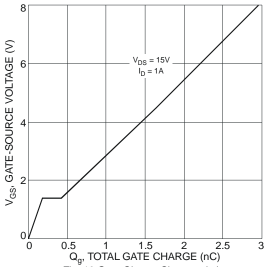
Fig. 16 Gate-Charge Characteristics
