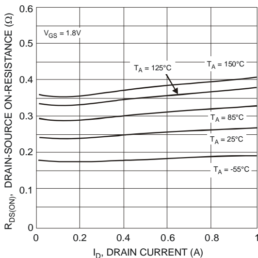
Fig. 8 Typical On-Resistance vs. Drain Current and Temperature
