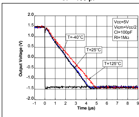
Figure 16. Negative slew rate at V_{CC} = 5\text{ V} with C_I = 100\text{ pF}
