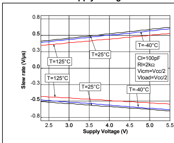
Figure 14. Positive and negative slew rate vs. supply voltage
