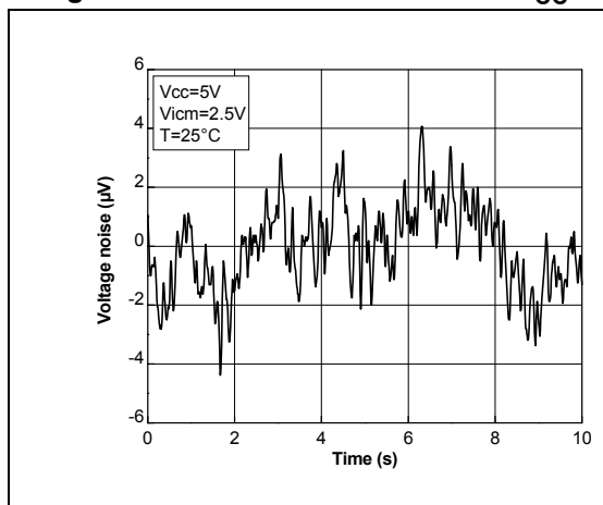
Figure 18. 0.1 Hz to 10 Hz noise at V_{CC} = 5\text{ V}
