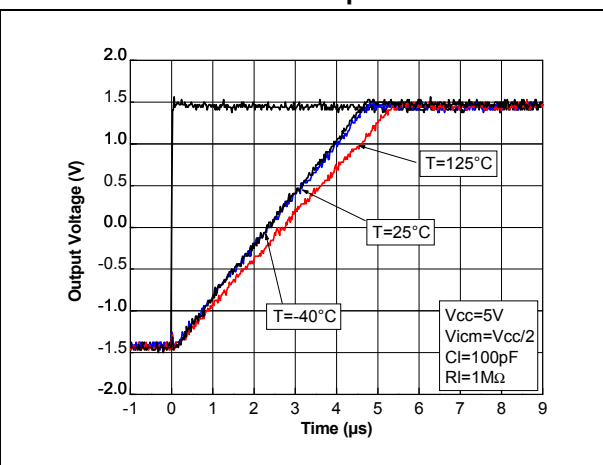
Figure 15. Positive slew rate at V_{CC} = 5\text{ V} with C_I = 100\text{ pF}
