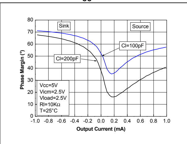
Figure 13. Phase margin vs. output current at VCC = 5 V
