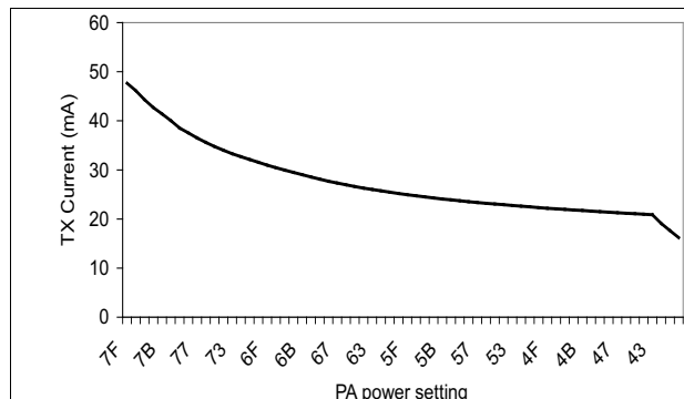
Figure 4-1. TX Current at 868 MHz vs PA Power Setting
