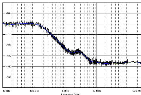
Figure 4-8. Phase Noise in 868-MHz Band
