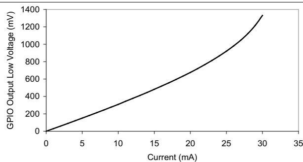
Figure 4-10. GPIO Output Low Voltage vs Current Being Sunk
