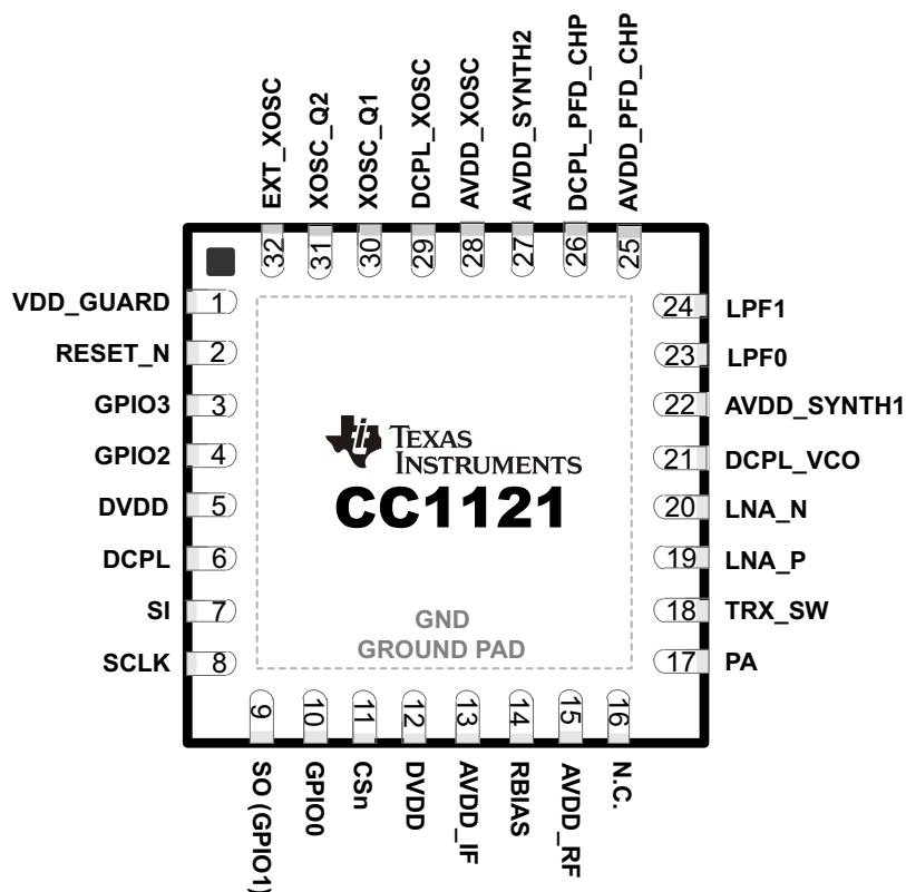
Figure 3-1. Package 5-mm × 5-mm QFN
