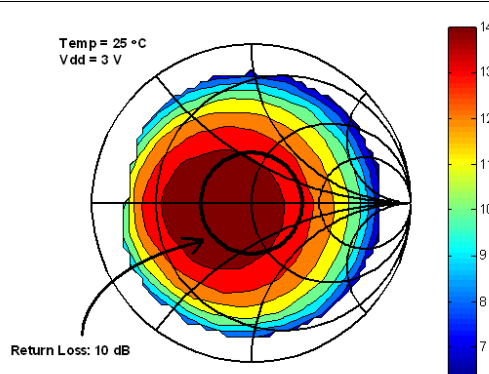
Figure 4-6. Output Power vs Load Impedance (+14-dBm Setting)
