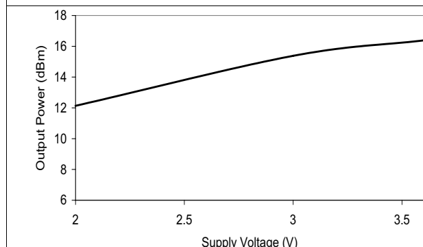
Figure 4-3. Output Power vs Voltage Max Setting, 170 MHz
