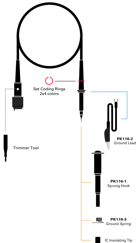
Passive Probe Accessories for PP006C Replacement Part Kit: PK116
