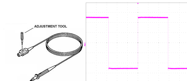
Adjusting Probe Compensation
