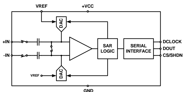
FIGURE 1. BLOCK DIAGRAM
