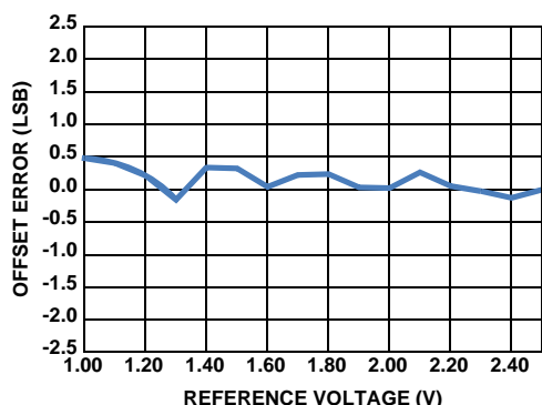
FIGURE 6. CHANGE IN OFFSET vs REFERENCE VOLTAGE
