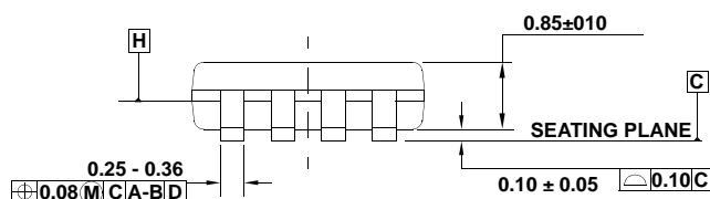
SIDE VIEW 1
