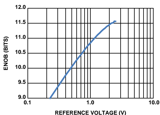
FIGURE 10. EFFECTIVE NUMBER OF BITS vs REFERENCE VOLTAGE
