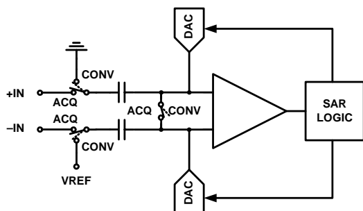
FIGURE 25. SAR ADC ARCHITECTURAL BLOCK DIAGRAM
