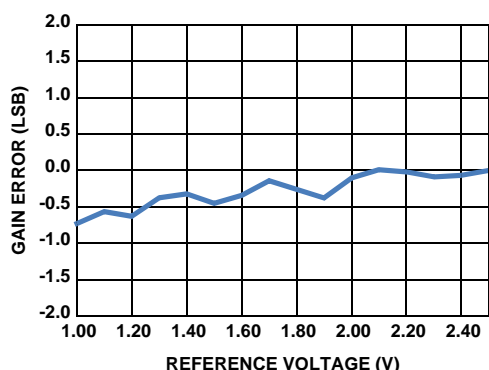
FIGURE 8. CHANGE IN GAIN vs REFERENCE VOLTAGE
