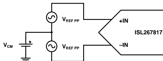
FIGURE 27. DIFFERENTIAL INPUT SIGNALING
