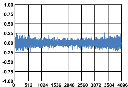
FIGURE 2. DIFFERENTIAL LINEARITY ERROR vs CODE
