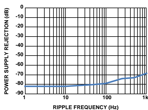
FIGURE 11. POWER SUPPLY REJECTION vs RIPPLE FREQUENCY
