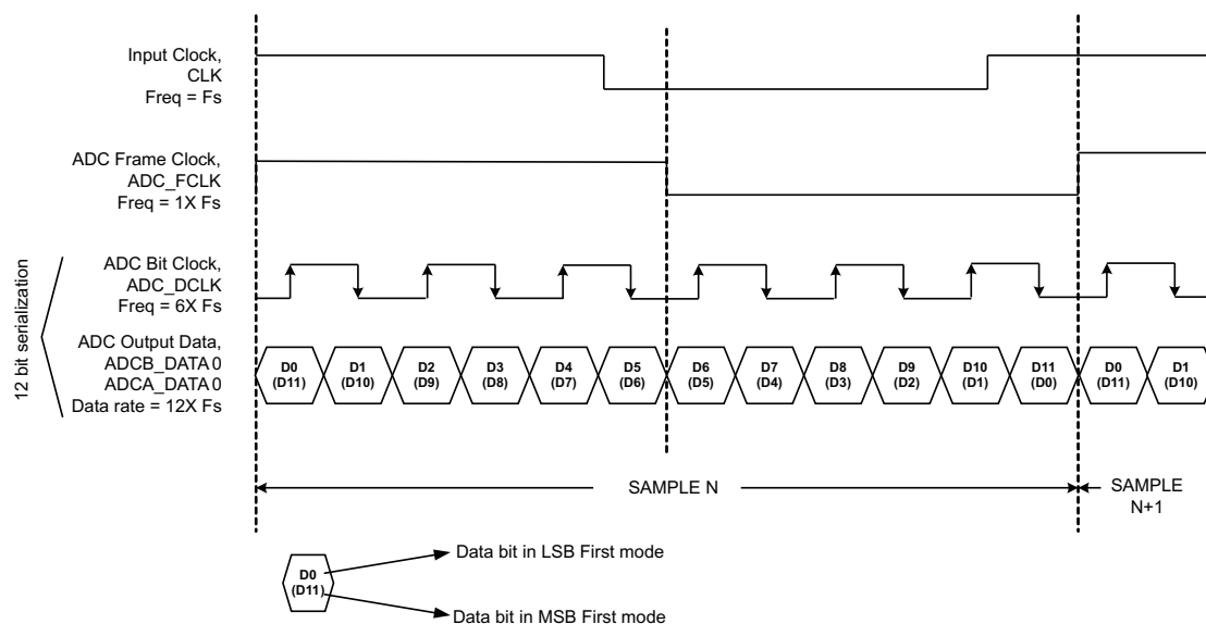
Figure 10-11. 1-WIRE MODE
