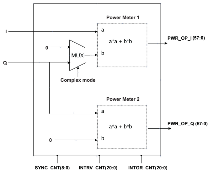
Figure 9-4. Fine Power Meter
