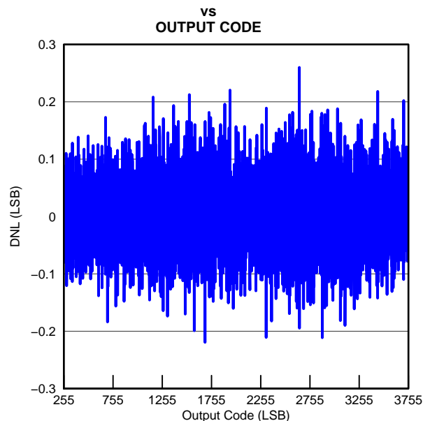
Figure 7-16. DNL Plot
