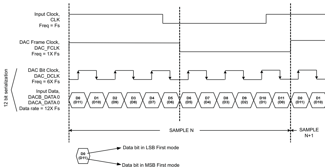
Figure 10-7. 1-WIRE MODE
