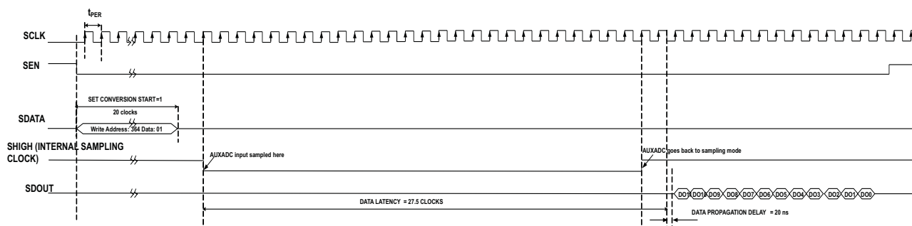
Figure 10-16. AUX ADC Timing Diagram
