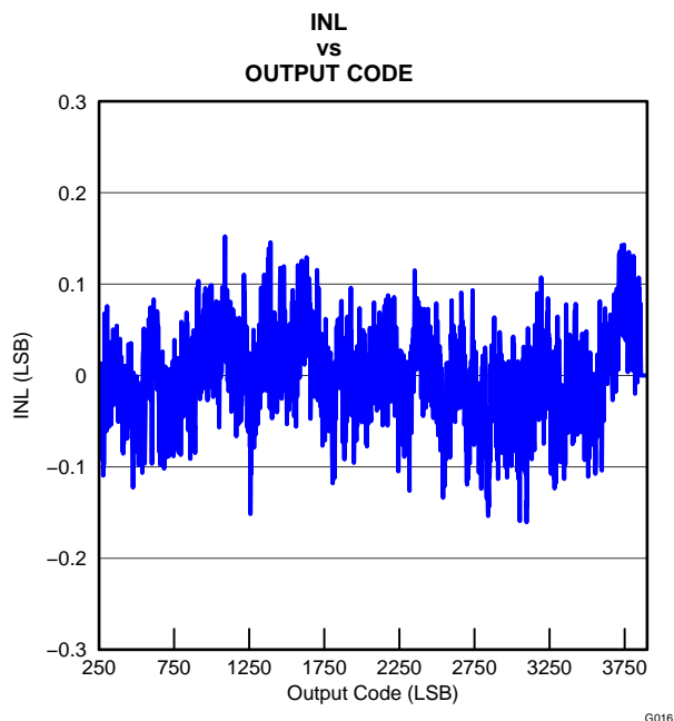
Figure 6-17. INL Plot
