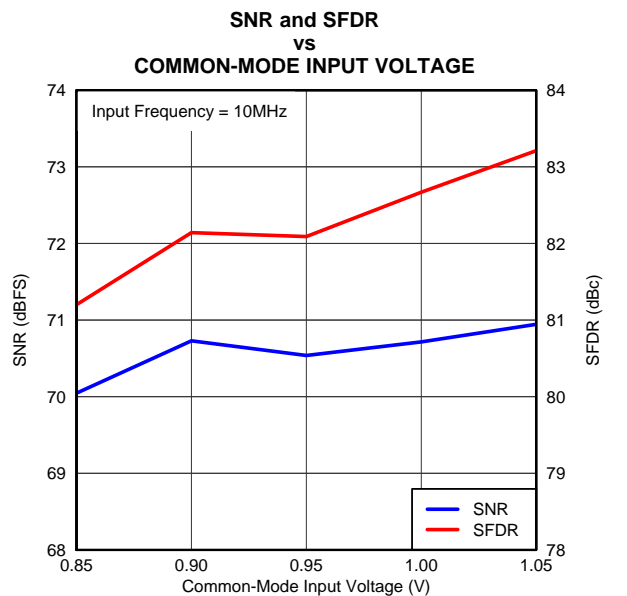
Figure 7-13. Performance Across Common-Mode Input Voltage
