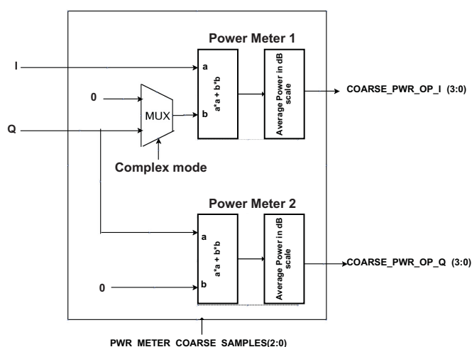
Figure 9-3. Coarse Power Meter
