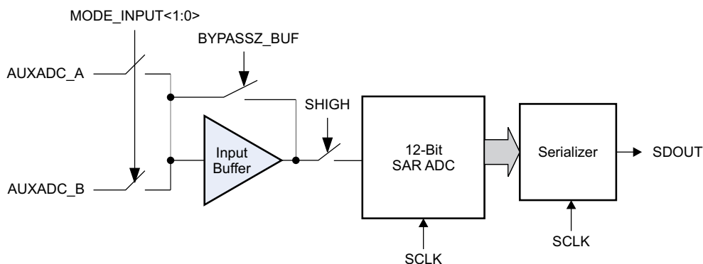
Figure 10-15. Auxiliary ADC Schematic
