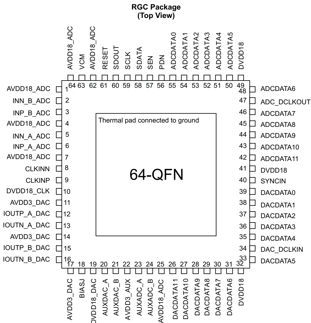
Figure 2-1. Device Pinout, CMOS Input/Output Mode
