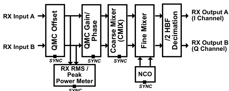
Figure 5-3. Signal Chain
