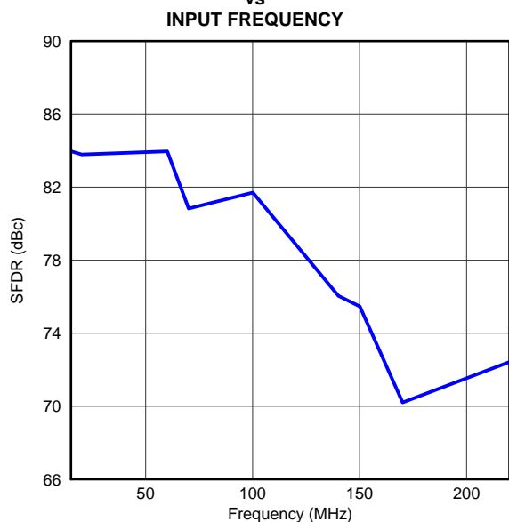
Figure 7-7. SFDR vs Input Frequency
