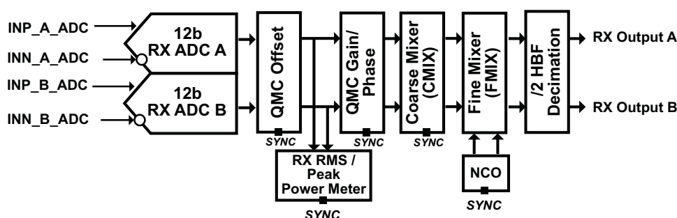
Figure 9-1. Signal Chain
