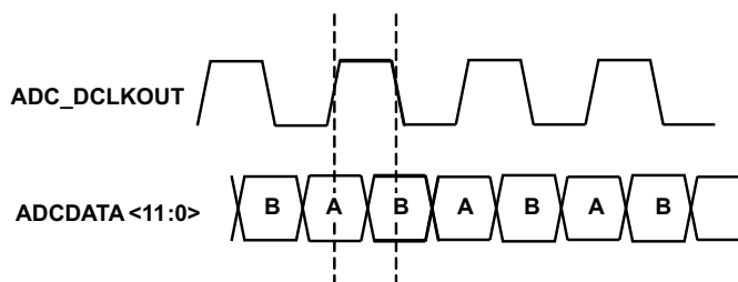
Figure 11-1. RX CMOS Output Interface
