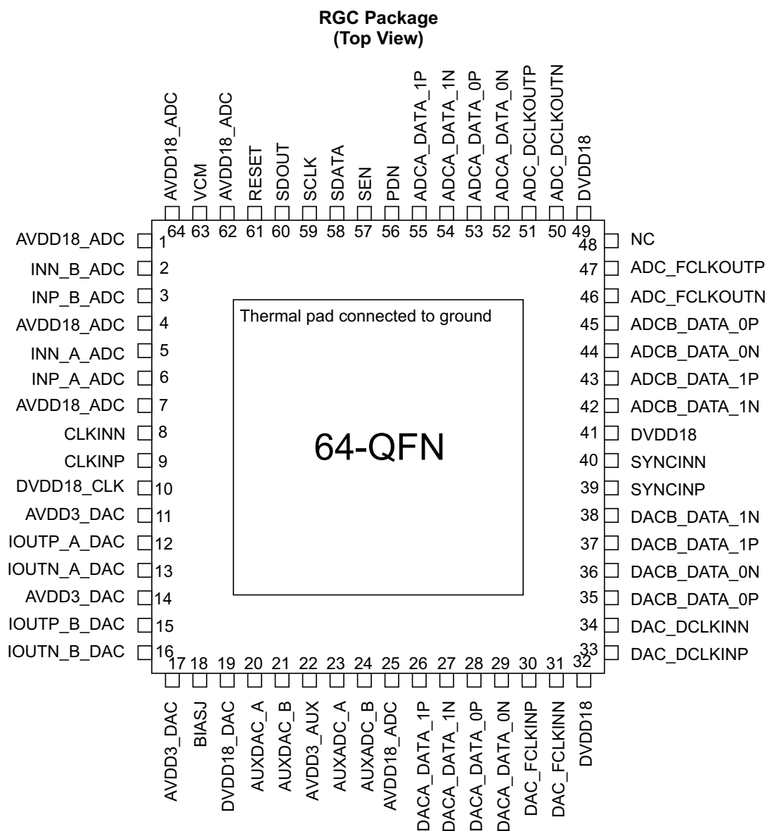
Figure 2-2. Device Pinout, LVDS Input/Output Mode
