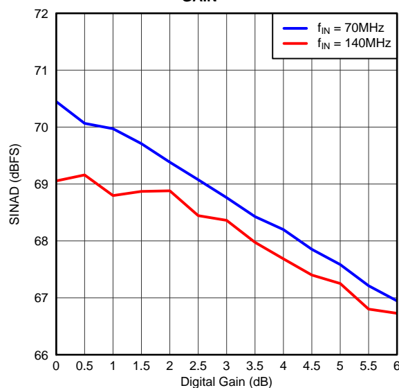
Figure 7-8. SINAD Across Gain
