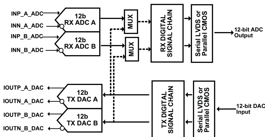
Figure 5-4. Signal Chain
