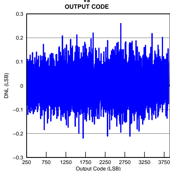
Figure 6-16. DNL Plot
