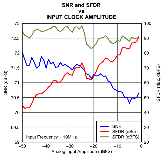
Figure 7-14. Performance Across Input Clock Amplitude
