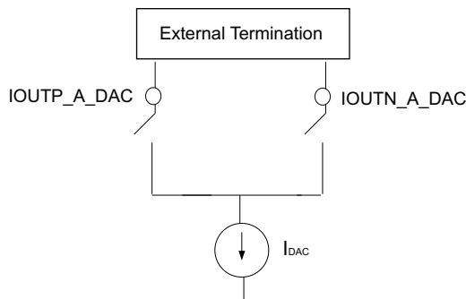
Figure 9-8. Current Steering Architecture of DAC
