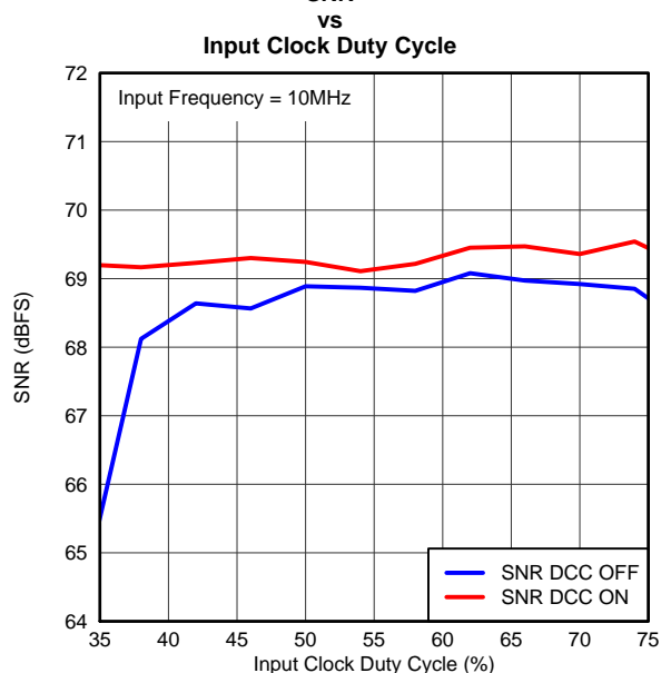
Figure 6-15. SNR vs Input Clock Duty Cycle
