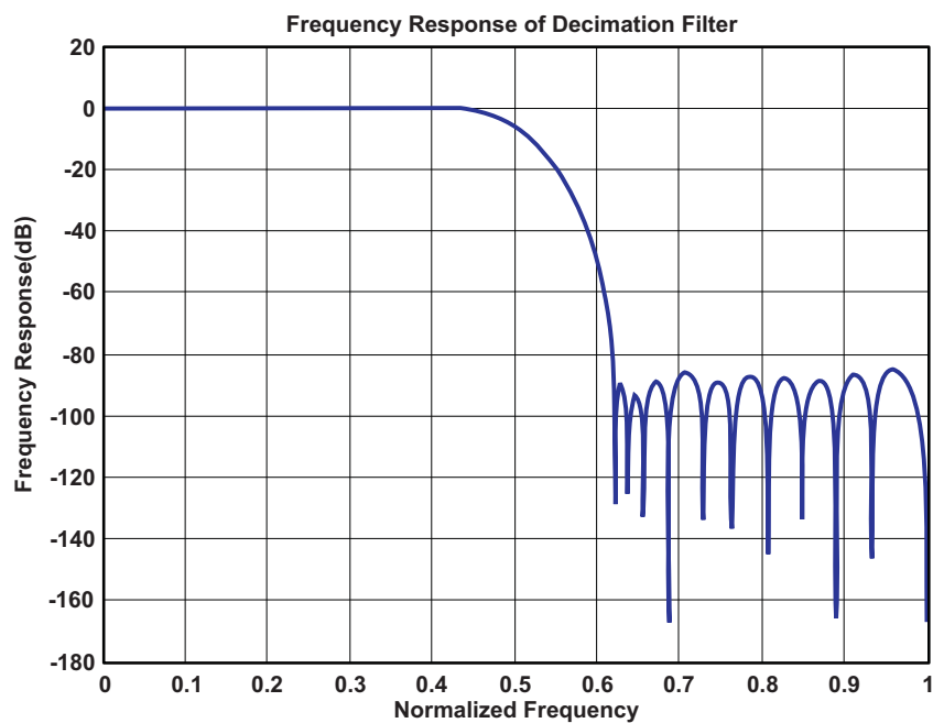
Figure 9-2. Decimation Filter Frequency Response (from 0 to F_{\text{ADCCLK}}/2 )
