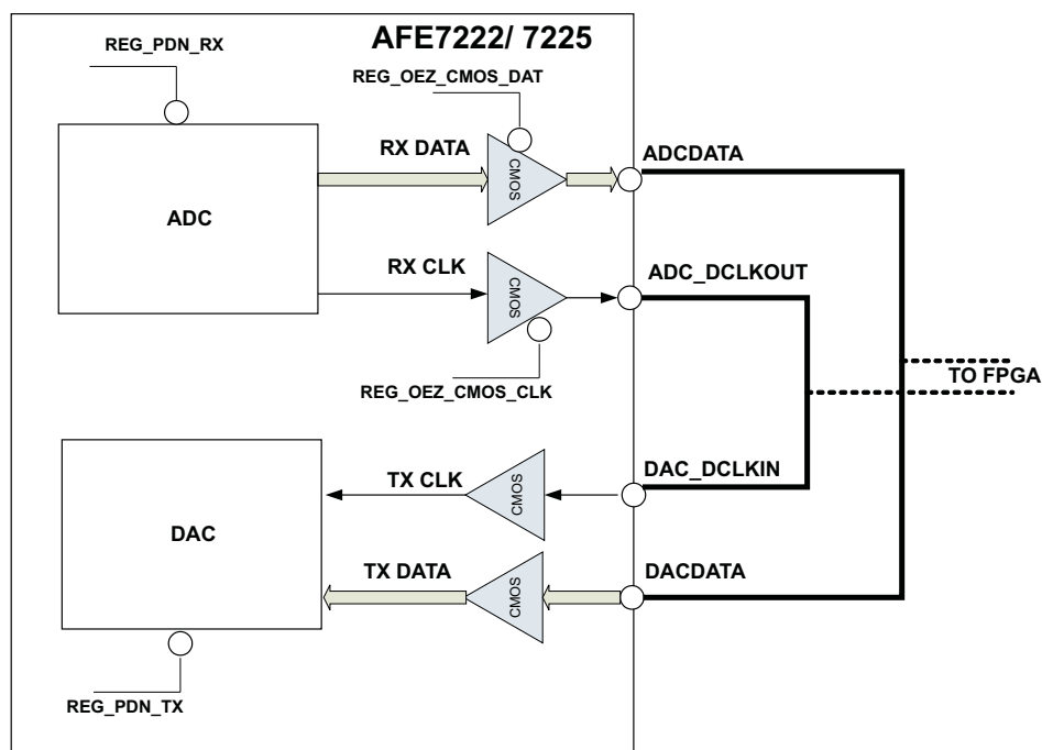
Figure 10-21. I/O Interface
