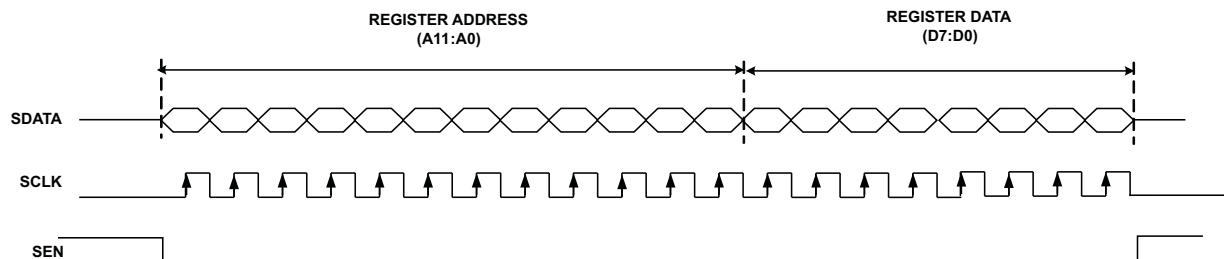
Figure 4-1. Timing
