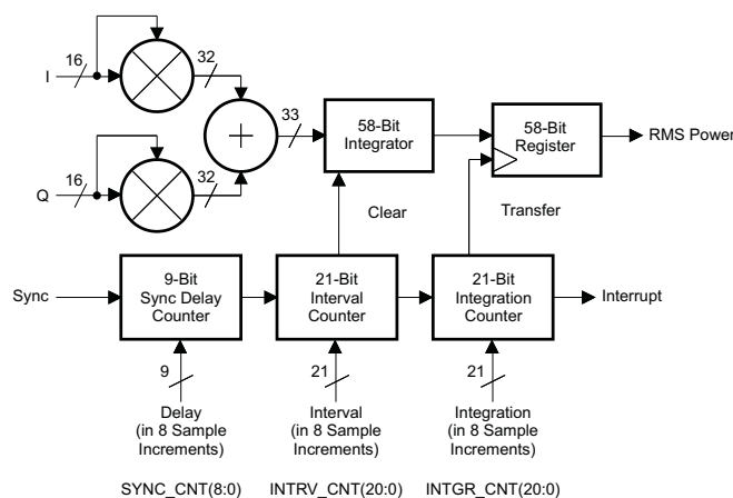
Figure 9-5. Power Meter Detailed Diagram
