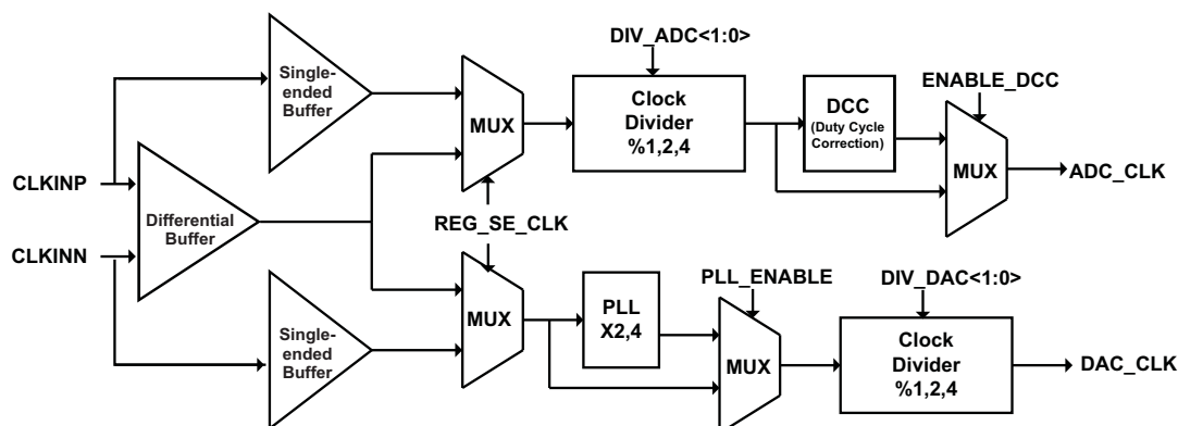
Figure 10-20. Block Diagram of Clocking Path
