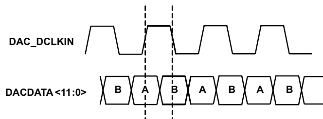
Figure 10-3. TX CMOS Interleaved Input
