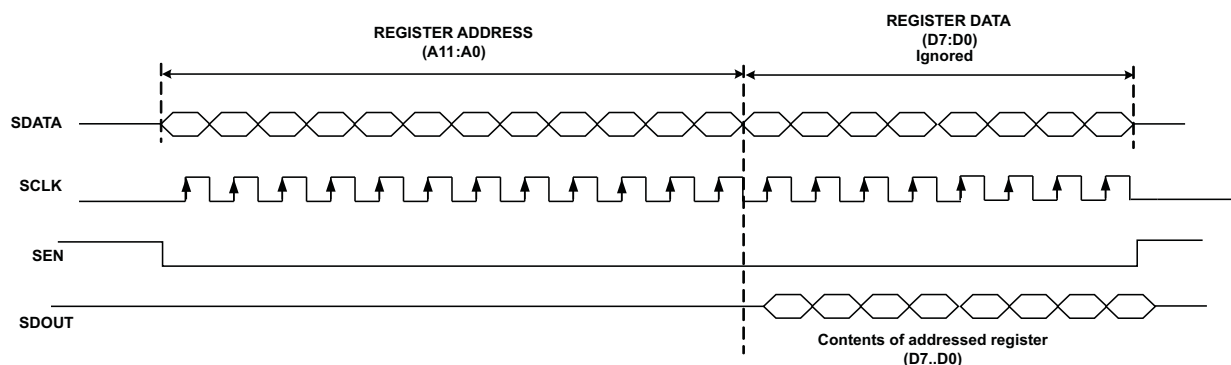
Figure 4-2. Timing
