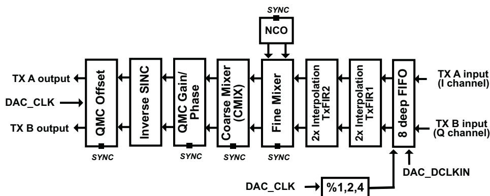
Figure 5-1. Signal Chain
