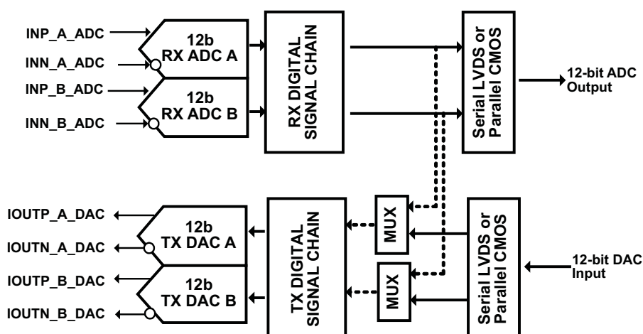
Figure 5-2. Loopback
