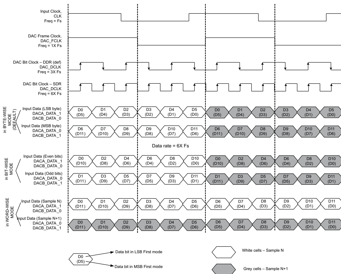
Figure 10-8. 2-WIRE MODE
