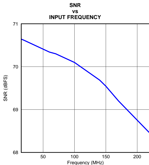
Figure 7-6. SNR vs Input Frequency
