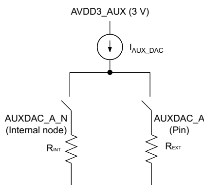
Figure 10-17. Auxiliary DAC Schematic
