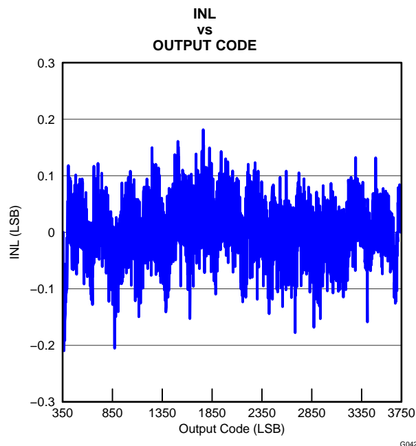
Figure 7-17. INL Plot
