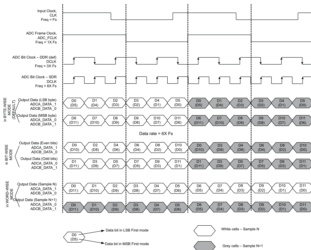
Figure 10-12. 2-WIRE MODE
