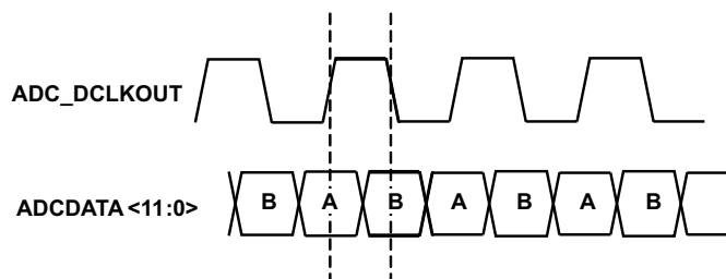
Figure 10-1. RX CMOS Interleaved Output
