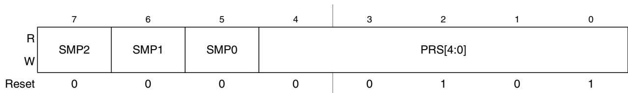
Figure 13-7. ATD Control Register 4 (ATDCTL4)
