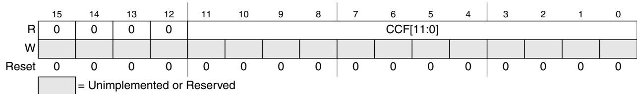
Figure 14-11. ATD Status Register 2 (ATDSTAT2)
