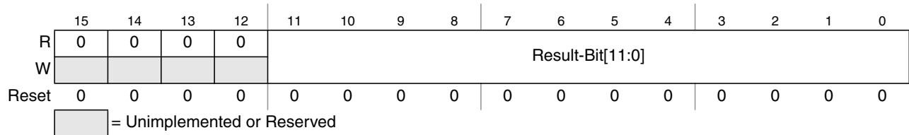
Figure 11-15. Right justified ATD conversion result register (ATDDRn)
