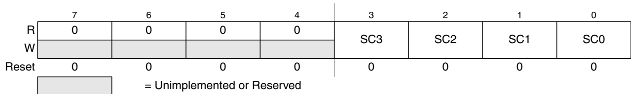
Figure 8-10. Debug State Control Register 2 (DBGSCR2)
