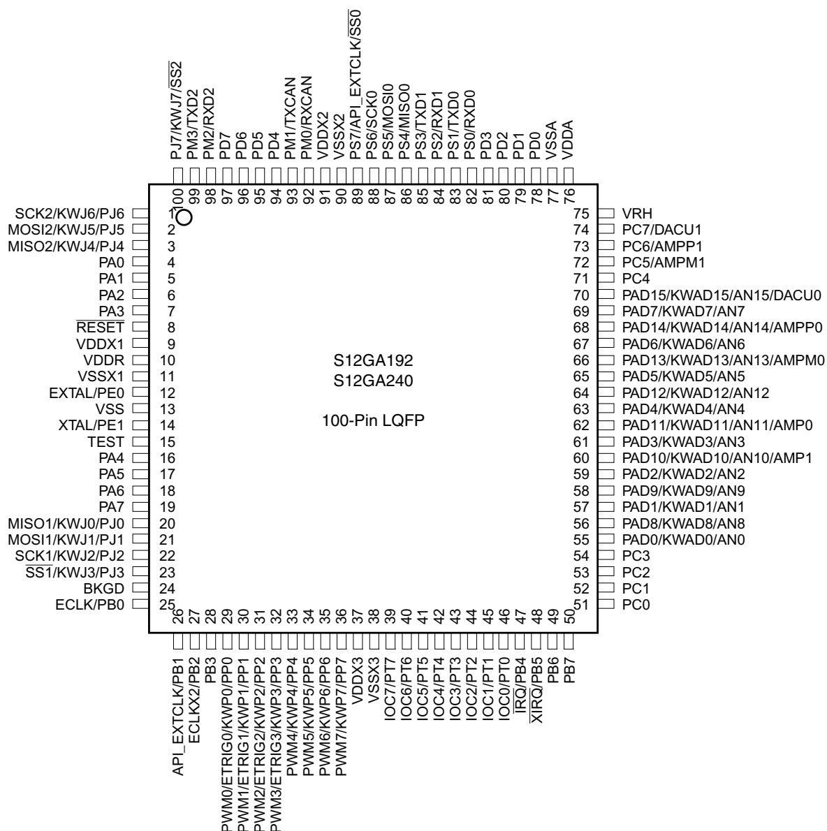
Figure 1-26. 100-Pin LQFP Pinout for S12GA192 and S12GA240
