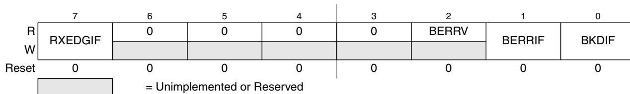
Figure 20-6. SCI Alternative Status Register 1 (SCIASR1)
