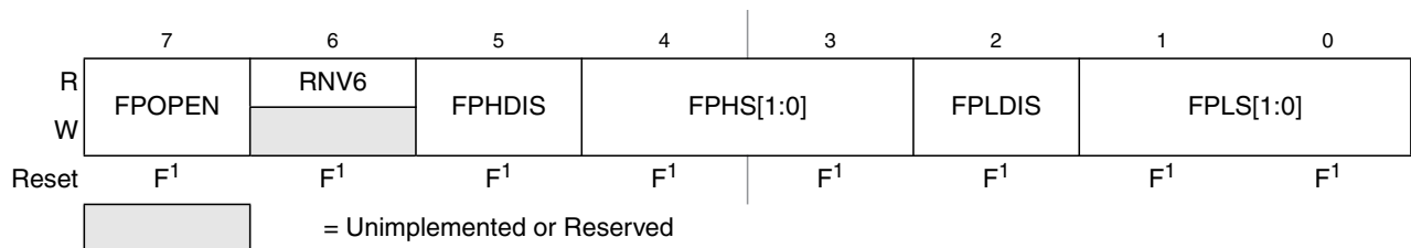
Figure 26-13. Flash Protection Register (FPROT)
