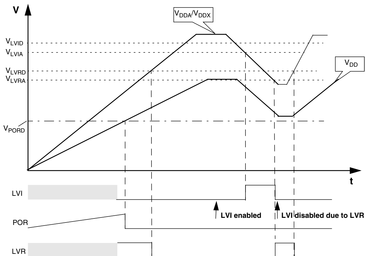
Figure A-6. Chip Power-up and Voltage Drops
