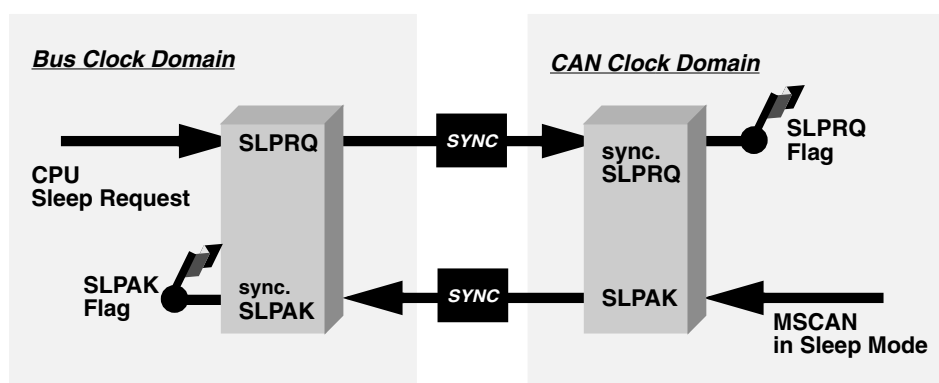
Figure 18-46. Sleep Request / Acknowledge Cycle
