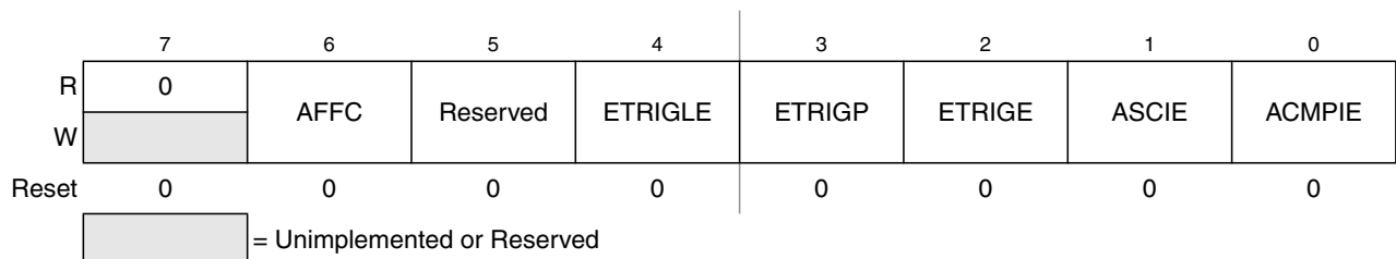
Figure 12-5. ATD Control Register 2 (ATDCTL2)
