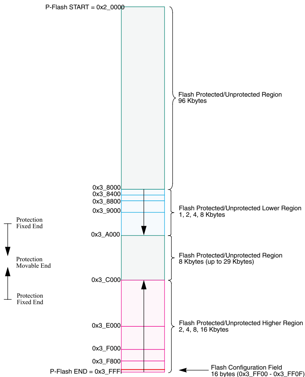
Figure 29-2. P-Flash Memory Map
