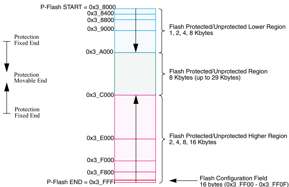
Figure 25-2. P-Flash Memory Map
