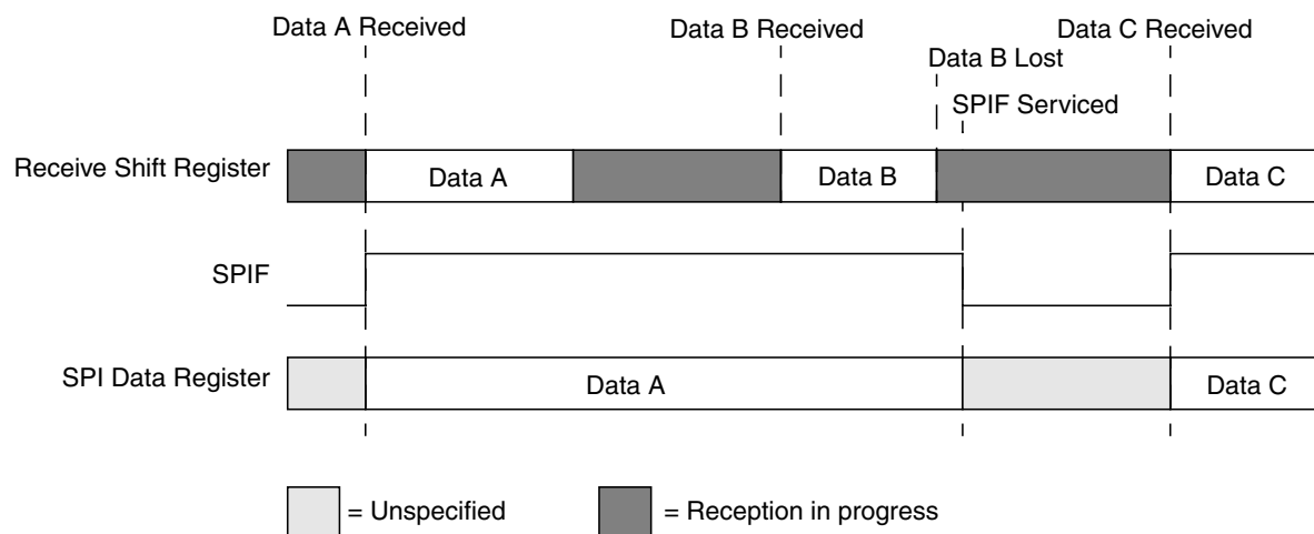
Figure 21-10. Reception with SPIF serviced too late
