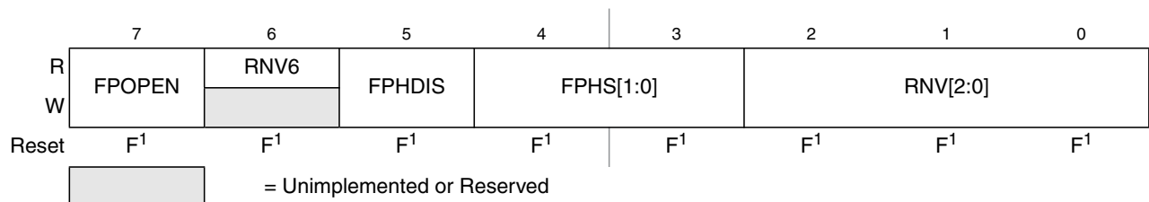
Figure 24-13. Flash Protection Register (FPROT)
