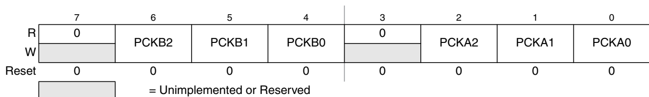
Figure 19-6. PWM Prescale Clock Select Register (PWMPRCLK)
