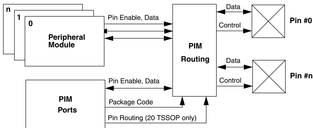
Figure 2-1. Block Diagram
