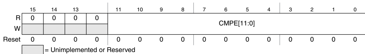
Figure 13-10. ATD Compare Enable Register (ATDCMPE)
