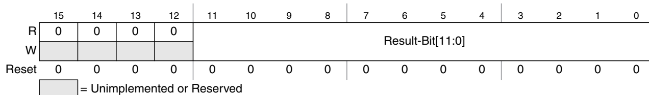
Figure 13-15. Right justified ATD conversion result register (ATDDR n )
