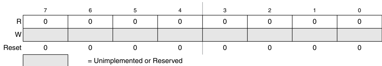
Figure 24-8. Flash Reserved0 Register (FRSV0)
