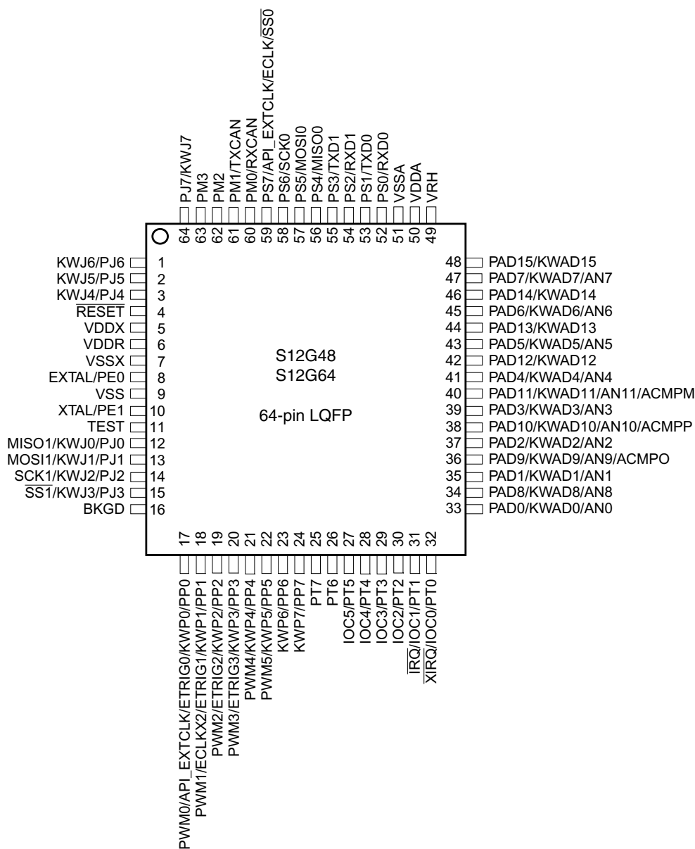
Figure 1-12. 64-Pin LQFP Pinout for S12G48 and S12G64
