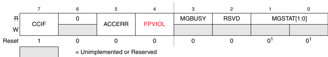
Figure 30-11. Flash Status Register (FSTAT)
