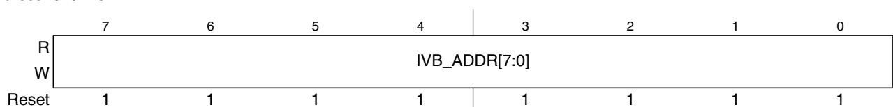
Figure 6-2. Interrupt Vector Base Register (IVBR)
