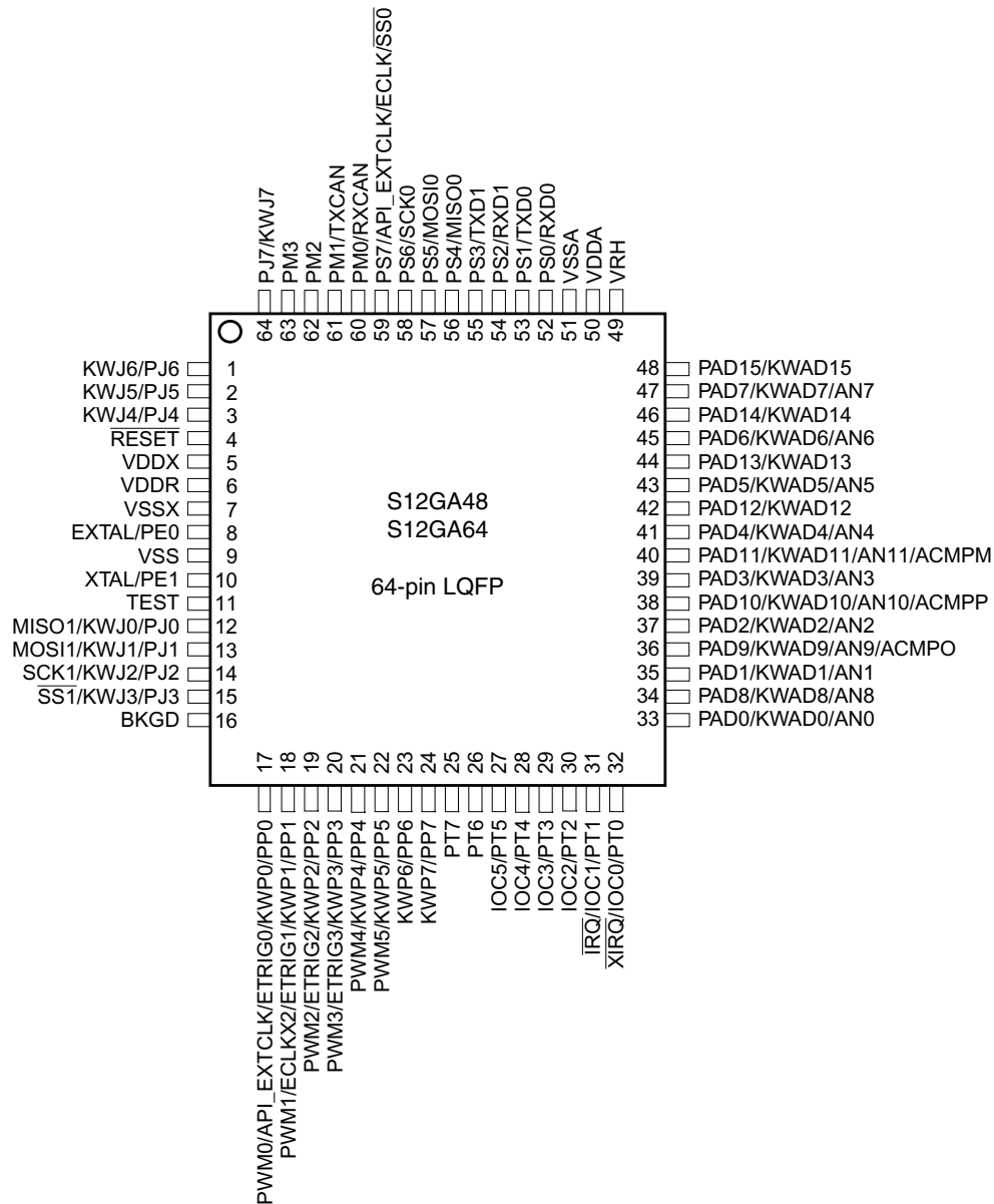
Figure 1-14. 64-Pin LQFP Pinout for S12GA48 and S12GA64
