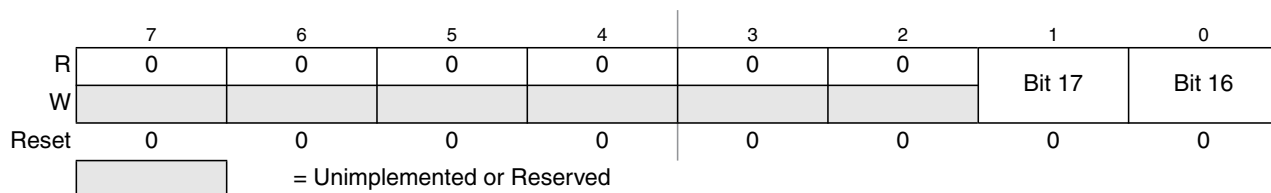
Figure 8-16. Debug Comparator Address High Register (DBGXAH)
