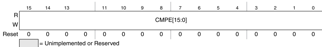
Figure 16-10. ATD Compare Enable Register (ATDCMPE)
