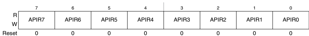
Figure 10-21. Autonomous Periodical Interrupt Rate Low Register (CPMUAPIRL)
