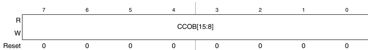
Figure 30-16. Flash Common Command Object High Register (FCCOBHI)
