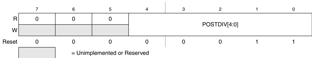
Figure 10-6. S12CPMU Post Divider Register (CPMUPOSTDIV)
