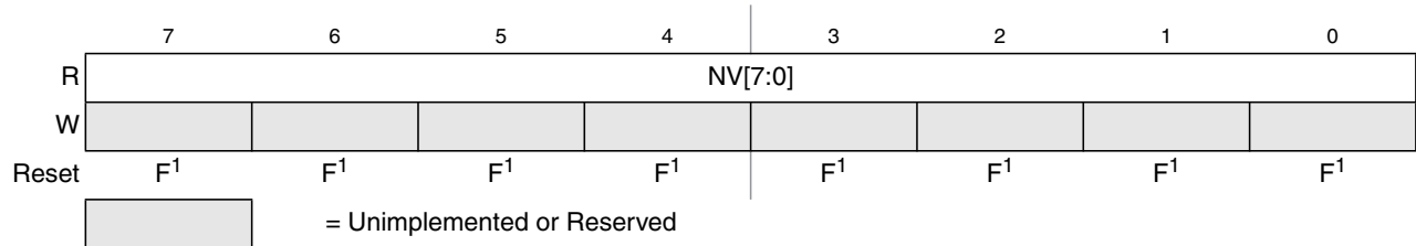
Figure 24-21. Flash Option Register (FOPT)
