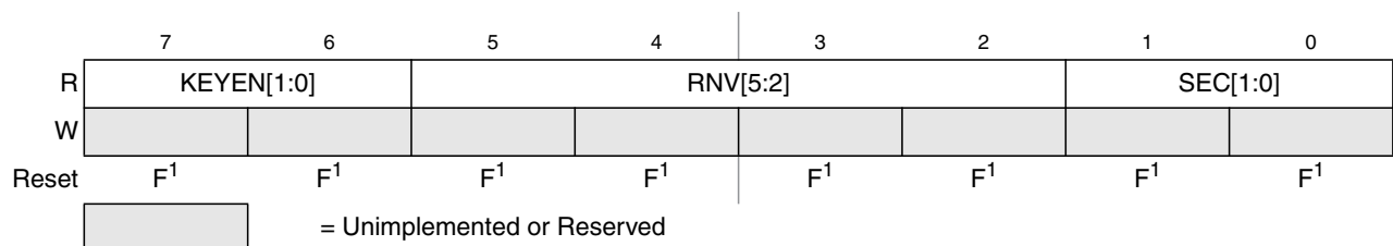
Figure 29-6. Flash Security Register (FSEC)
