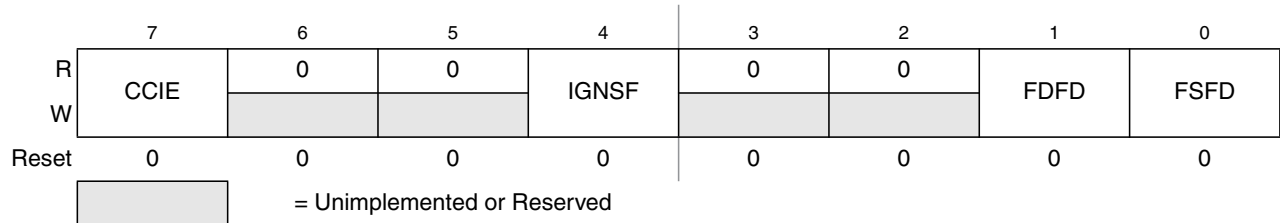
Figure 27-9. Flash Configuration Register (FCNFG)
