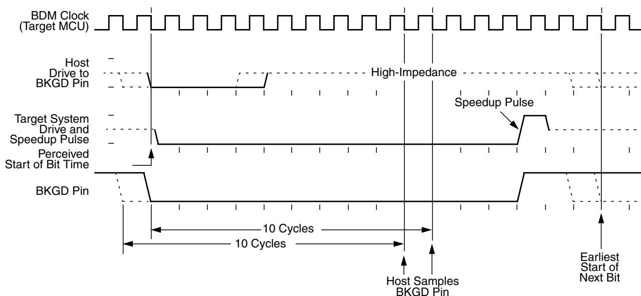
Figure 7-9. BDM Target-to-Host Serial Bit Timing (Logic 0)
