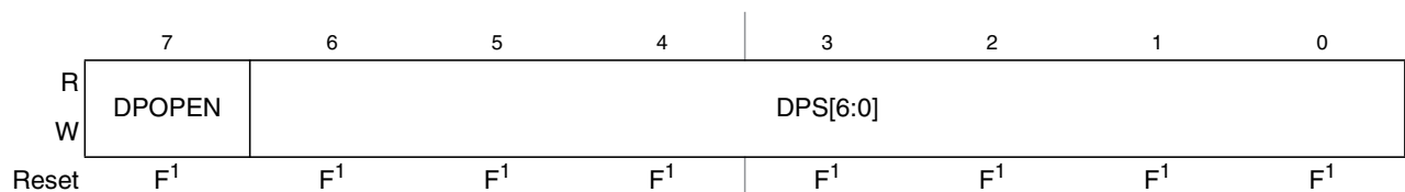
Figure 30-15. EEPROM Protection Register (EPROT)
