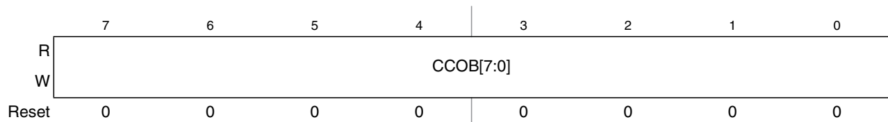
Figure 30-17. Flash Common Command Object Low Register (FCCOBLO)
