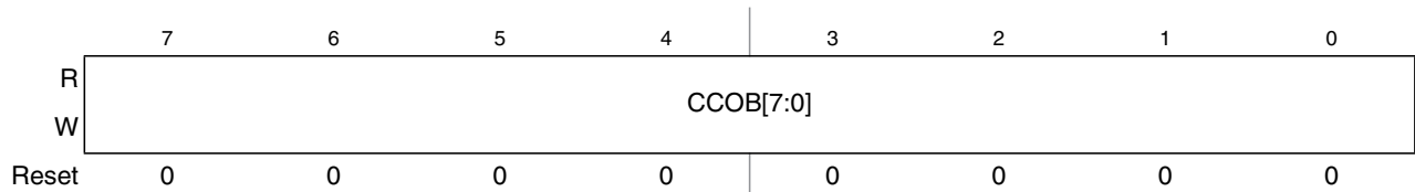
Figure 26-17. Flash Common Command Object Low Register (FCCOBLO)
