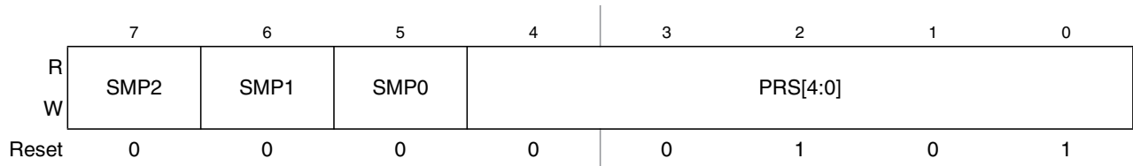
Figure 15-7. ATD Control Register 4 (ATDCTL4)
