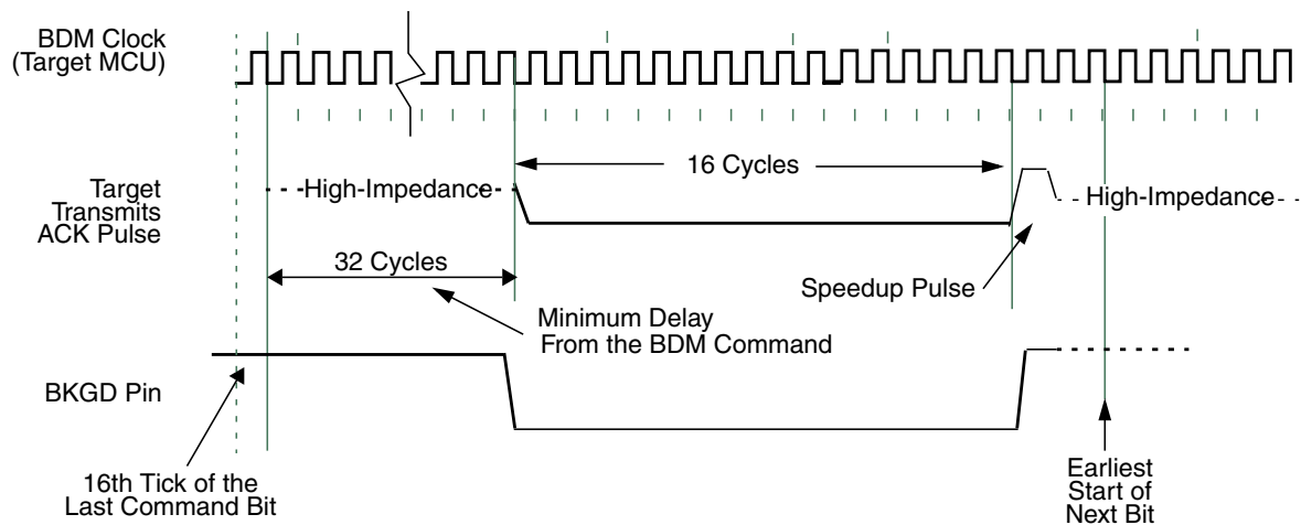
Figure 7-10. Target Acknowledge Pulse (ACK)
