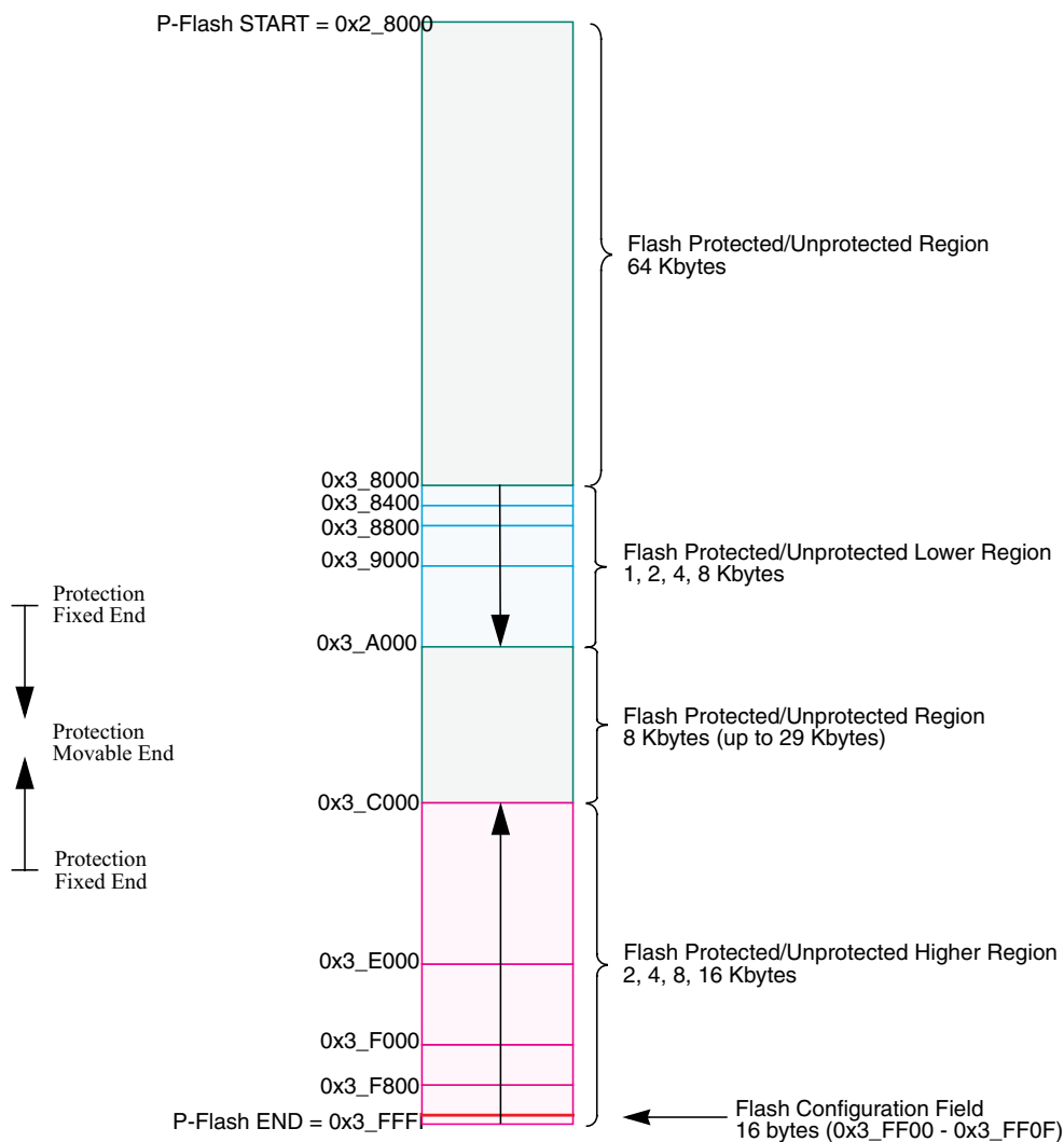
Figure 28-2. P-Flash Memory Map
