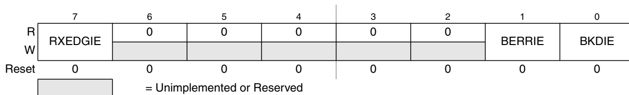
Figure 20-7. SCI Alternative Control Register 1 (SCIACR1)
