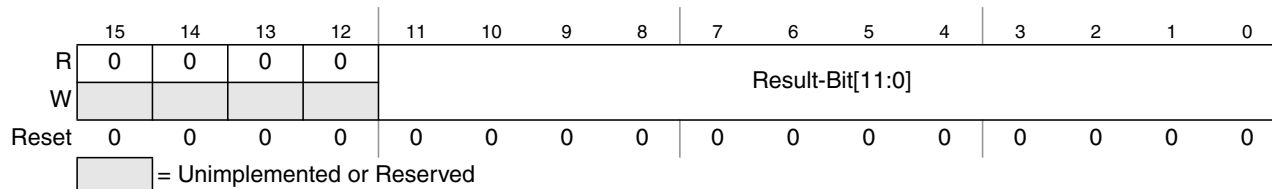
Figure 12-15. Right justified ATD conversion result register (ATDDRn)
