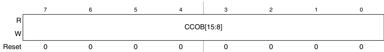
Figure 26-16. Flash Common Command Object High Register (FCCOBHI)
