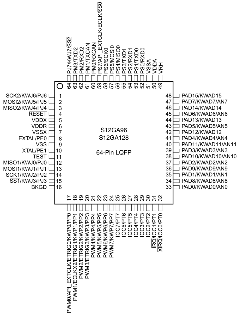
Figure 1-19. 64-Pin LQFP Pinout for S12GA96 and S12GA128
