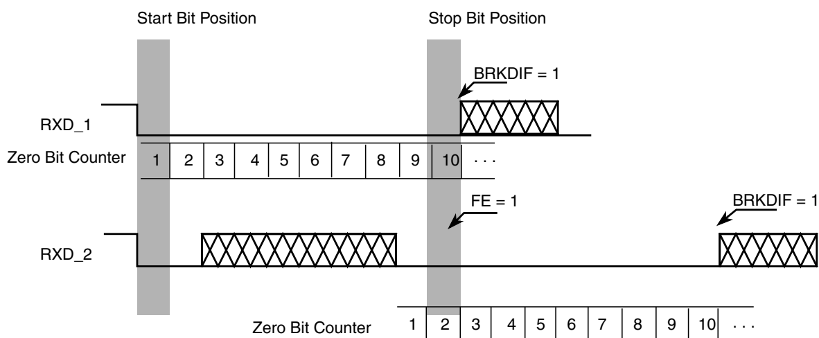
Figure 20-17. Break Detection if BRKDFE = 1 (M = 0)
