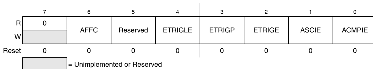
Figure 14-5. ATD Control Register 2 (ATDCTL2)
