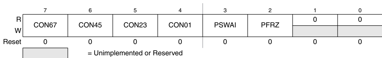
Figure 19-8. PWM Control Register (PWMCTL)
