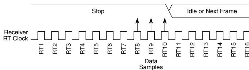
Figure 20-29. Fast Data
