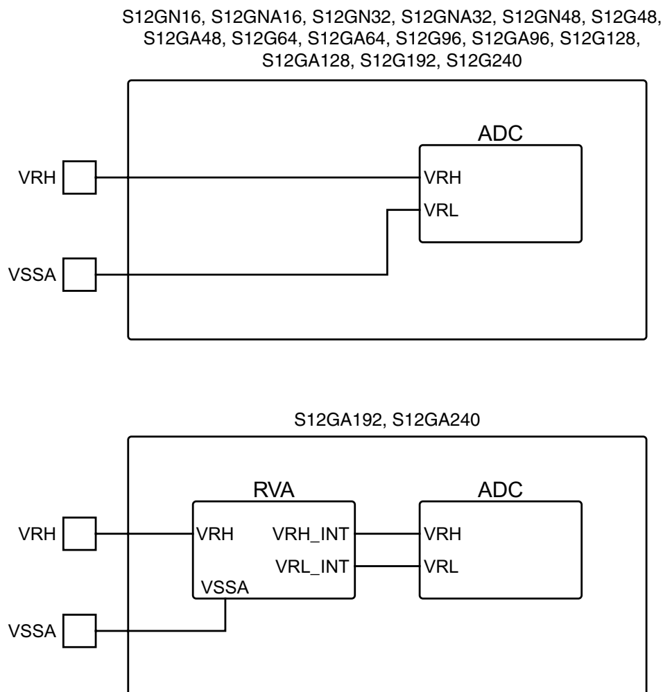
Figure 1-27. ADC VRH/VRL Signal Connection
