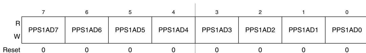
Figure 2-59. Port AD Polarity Select Register (PPS1AD)
