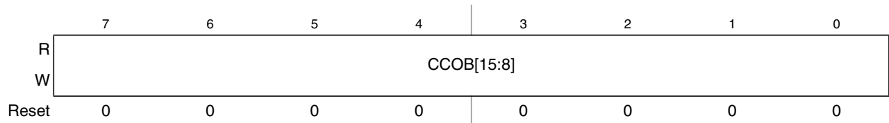
Figure 31-16. Flash Common Command Object High Register (FCCOBHI)
