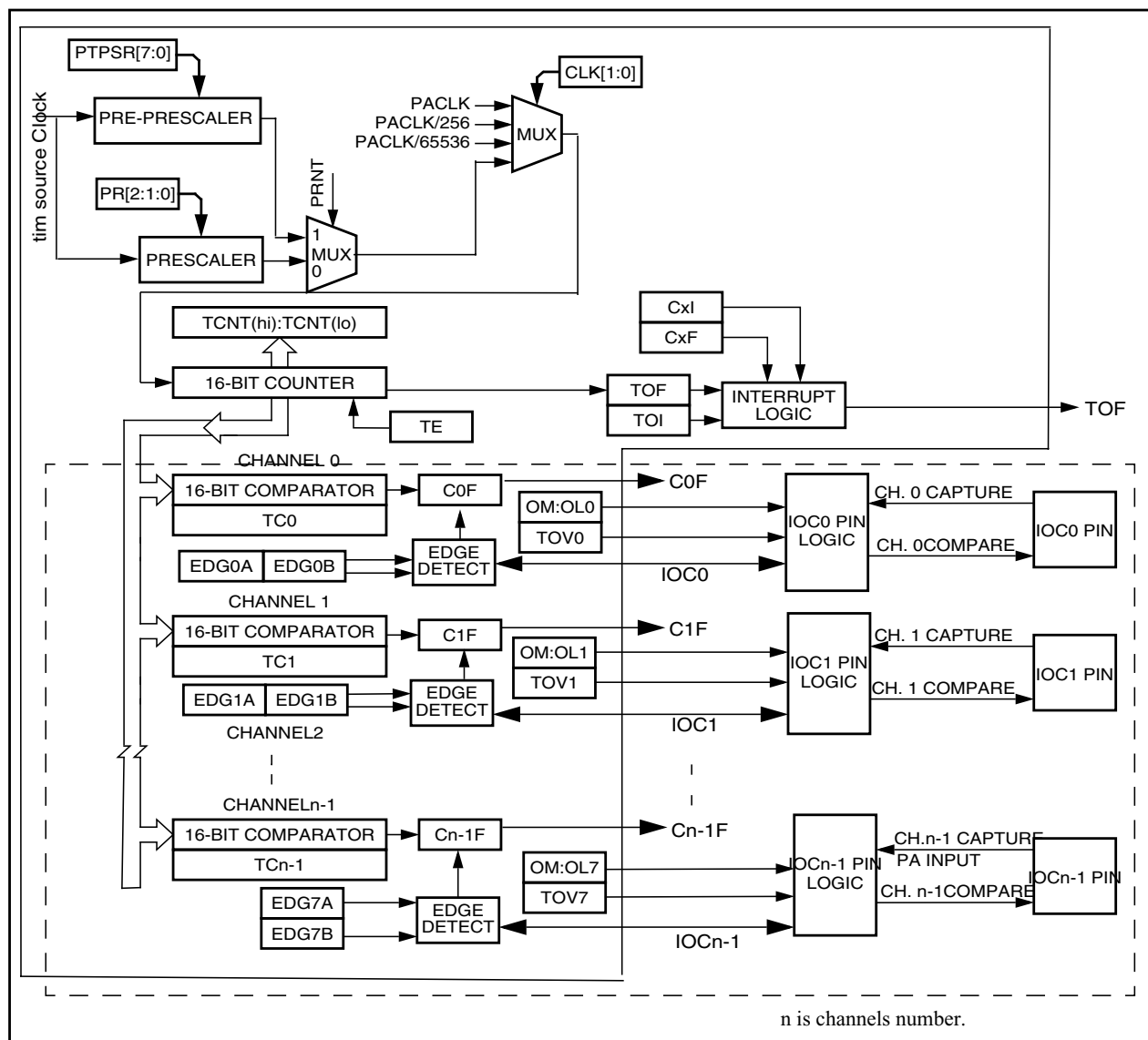
Figure 22-22. Detailed Timer Block Diagram
