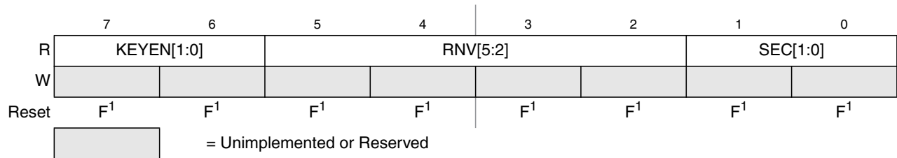
Figure 24-6. Flash Security Register (FSEC)
