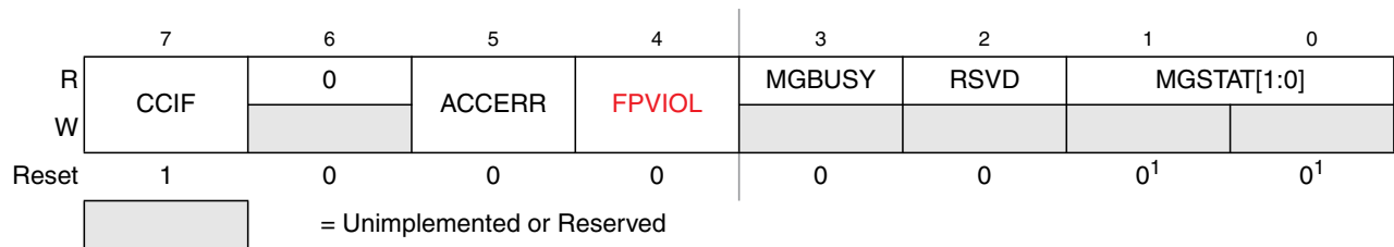
Figure 31-11. Flash Status Register (FSTAT)
