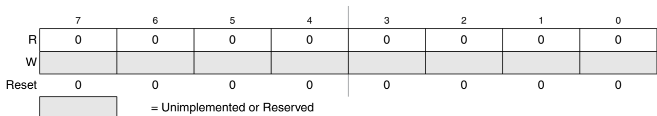
Figure 24-22. Flash Reserved5 Register (FRSV5)
