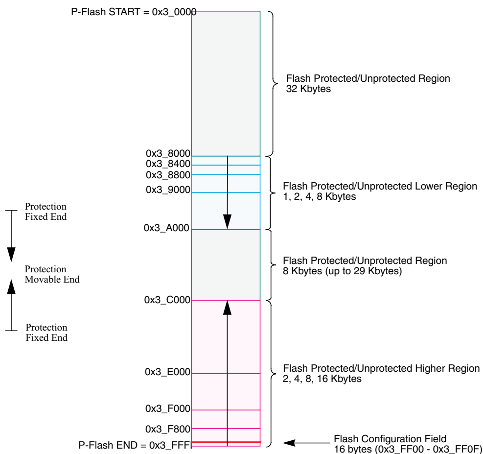
Figure 27-2. P-Flash Memory Map
