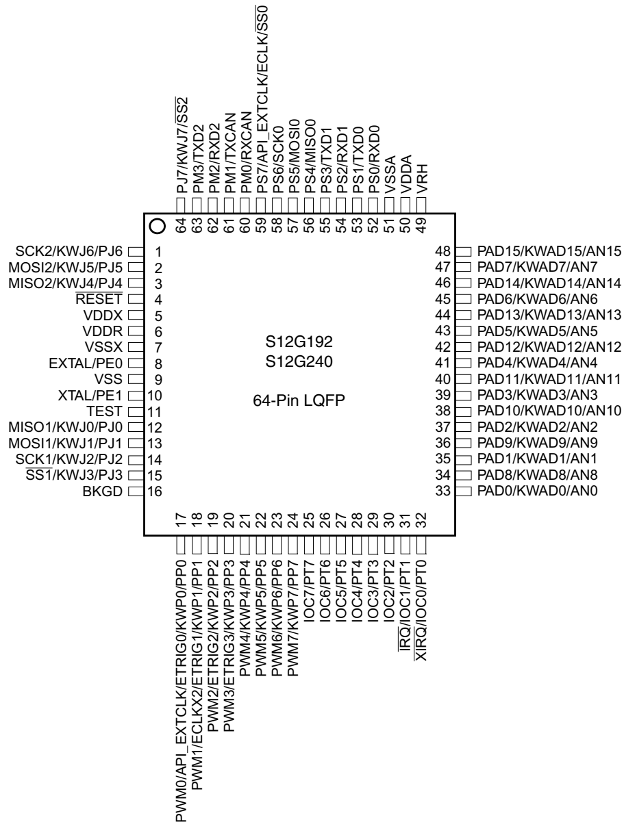
Figure 1-22. 64-Pin LQFP Pinout for S12G192 and S12G240
