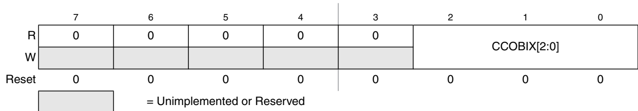
Figure 24-7. FCCOB Index Register (FCCOBIX)
