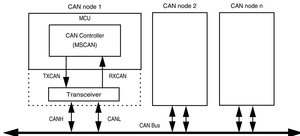
Figure 18-2. CAN System
