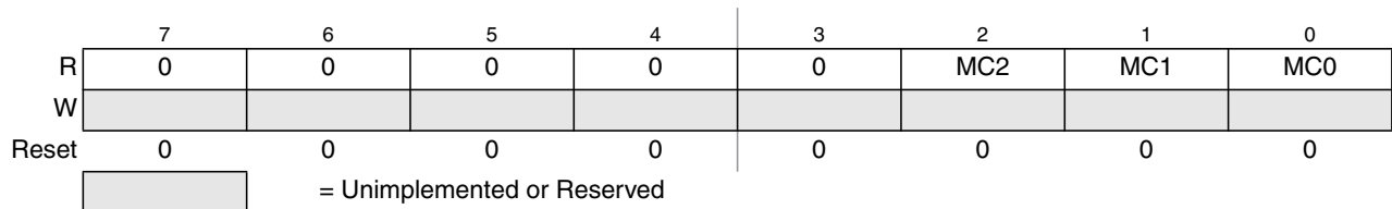
Figure 8-12. Debug Match Flag Register (DBGMFR)
