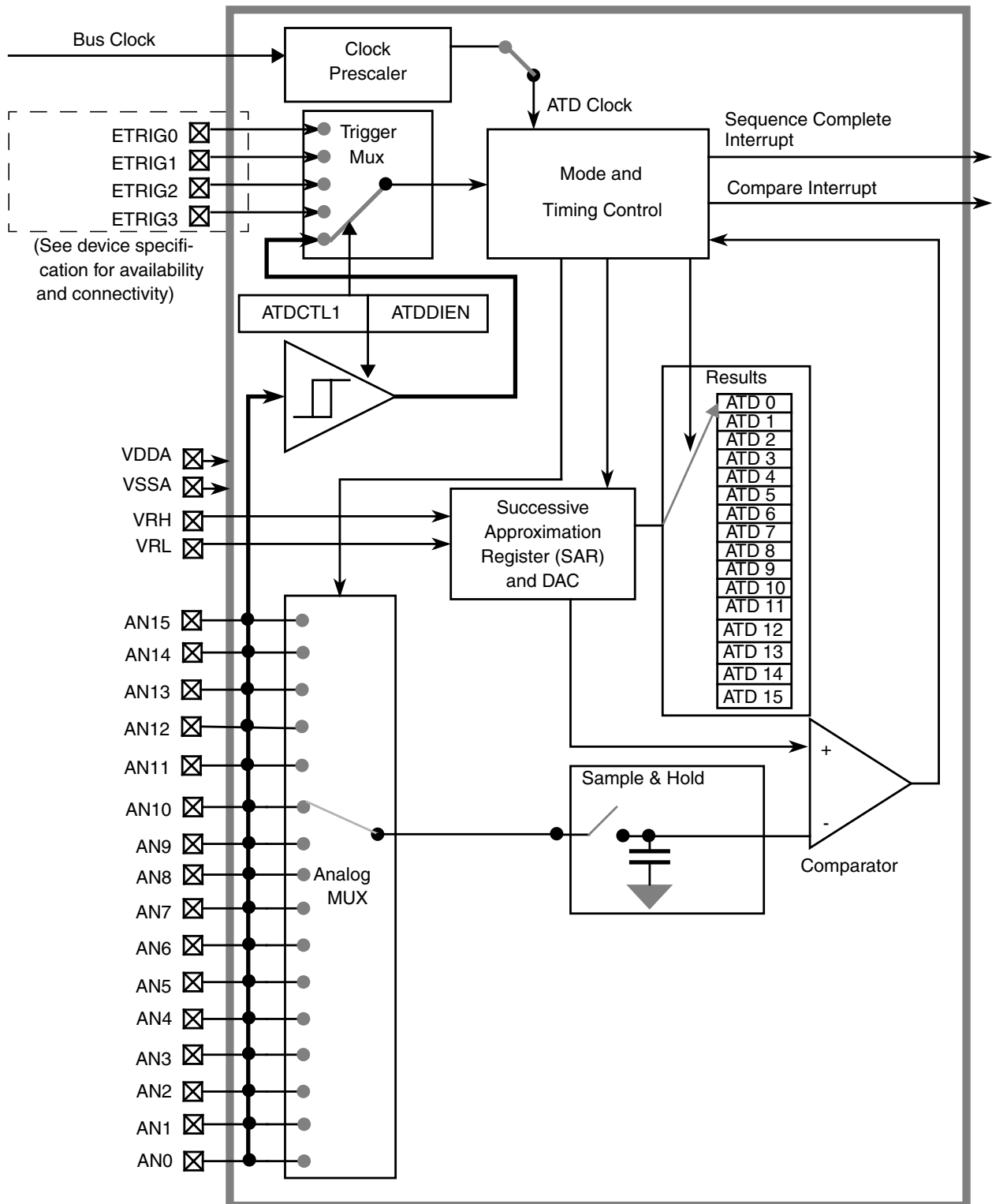
Figure 16-1. ADC12B16C Block Diagram
