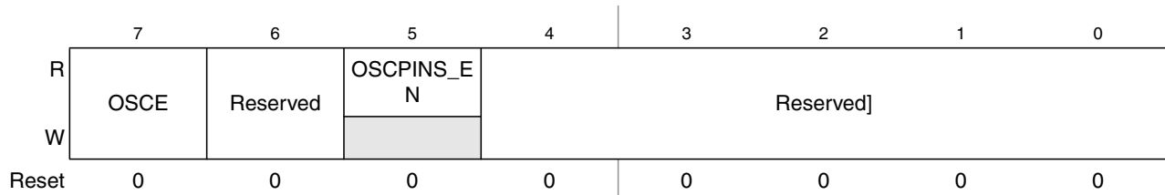
Figure 10-27. S12CPMU Oscillator Register (CPMUOSC)
