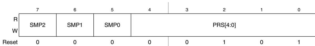
Figure 11-7. ATD Control Register 4 (ATDCTL4)
