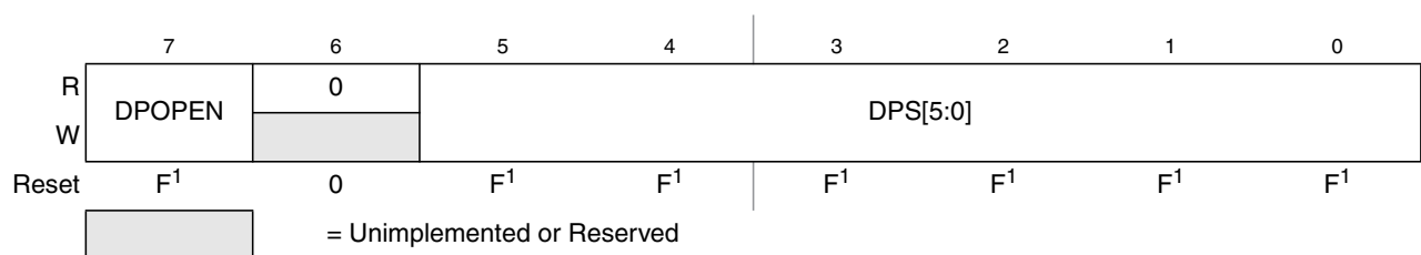
Figure 27-15. EEPROM Protection Register (EPROT)
