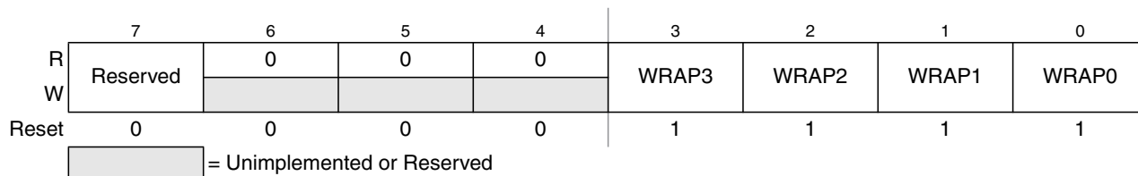
Figure 11-3. ATD Control Register 0 (ATDCTL0)
