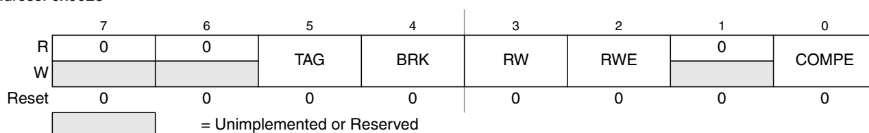
Figure 8-15. Debug Comparator Control Register DBGCCCTL (Comparator C)
