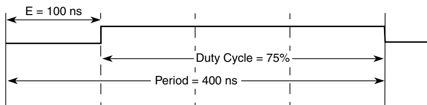
Figure 19-18. PWM Left Aligned Output Example Waveform
