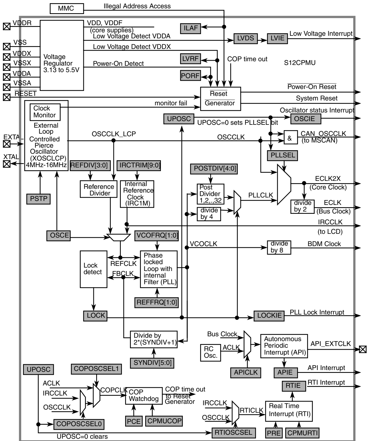
Figure 10-1. Block diagram of S12CPMU
