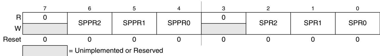
Figure 21-5. SPI Baud Rate Register (SPIBR)
