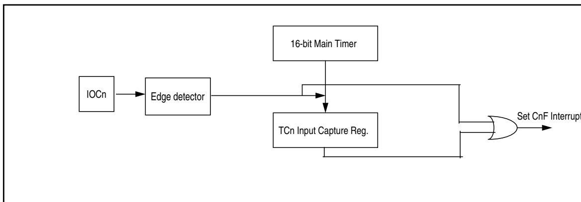
Figure 22-2. Interrupt Flag Setting
