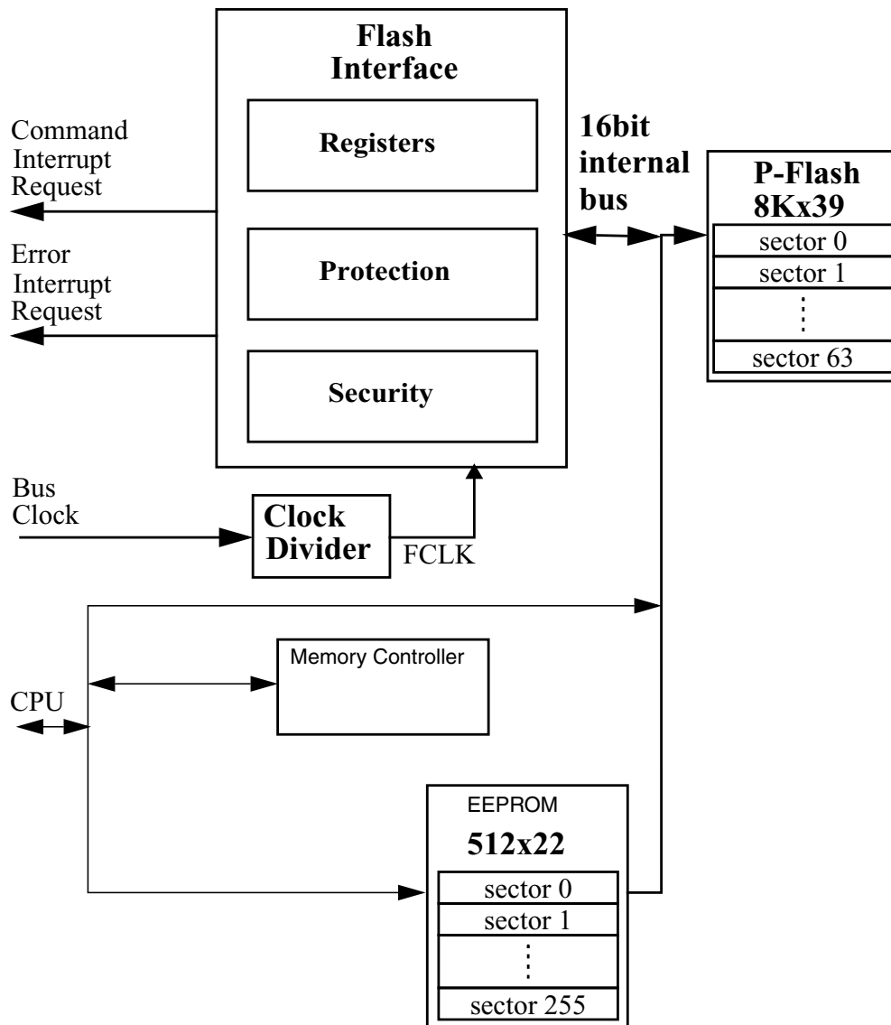
Figure 25-1. FTMRG32K1 Block Diagram
