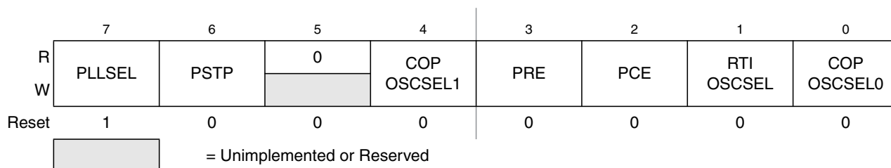
Figure 10-9. S12CPMU Clock Select Register (CPMUCLKS)
