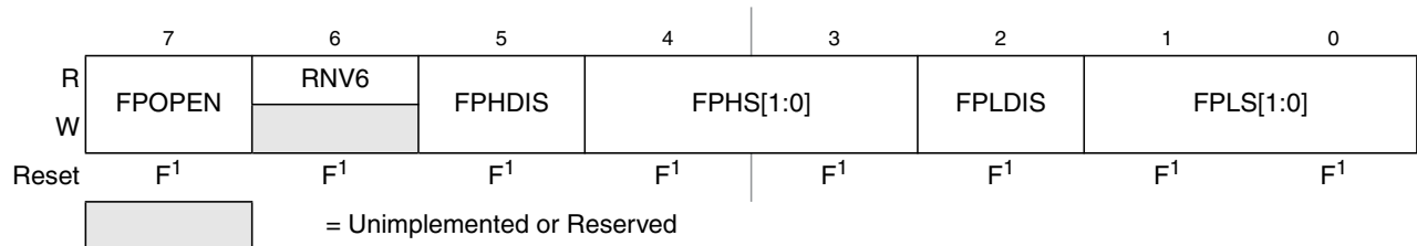
Figure 30-13. Flash Protection Register (FPROT)
