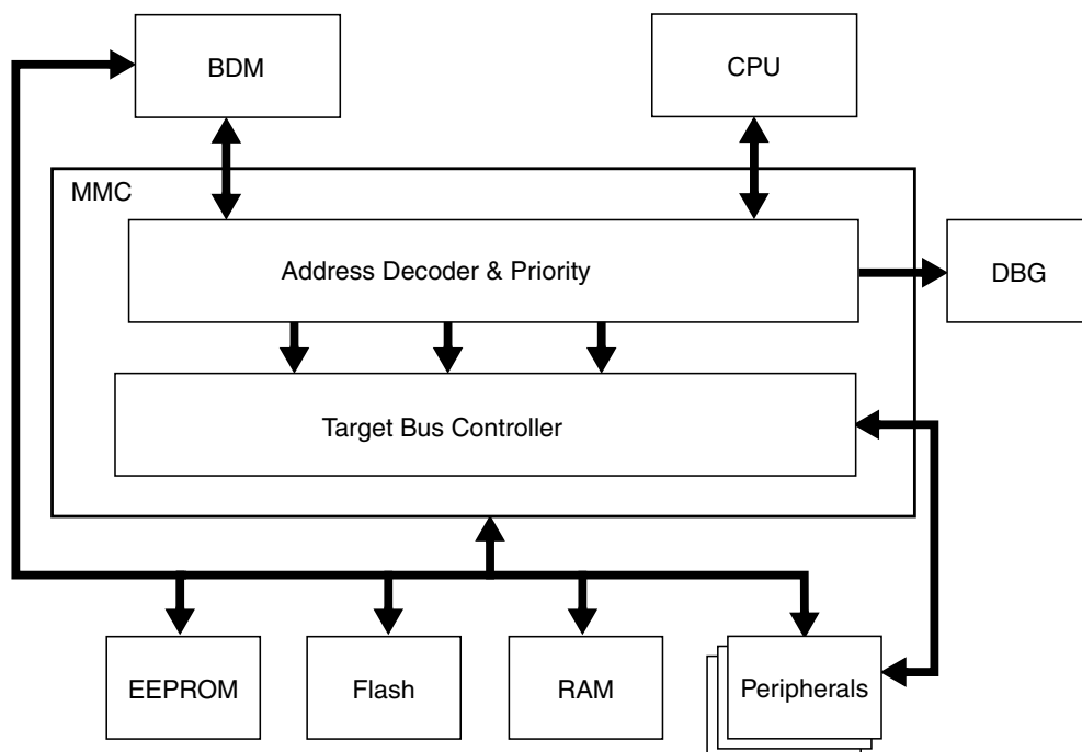
Figure 5-1. S12GMMC Block Diagram
