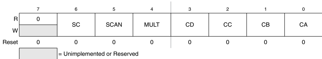
Figure 15-8. ATD Control Register 5 (ATDCTL5)
