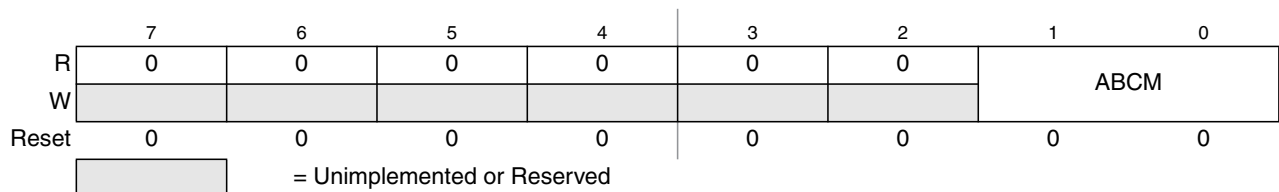
Figure 8-6. Debug Control Register2 (DBG2)
