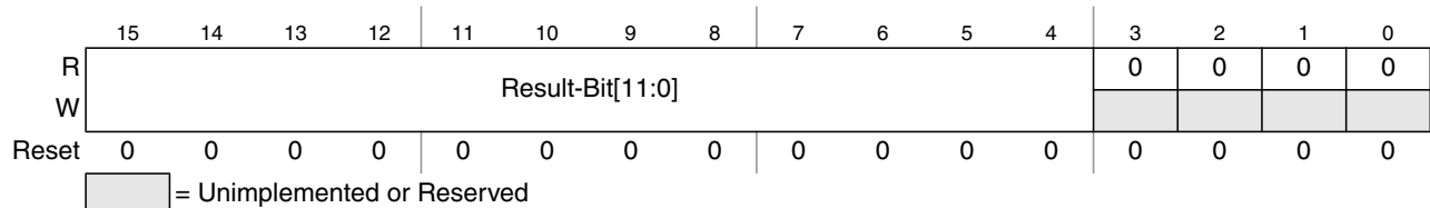
Figure 15-14. Left justified ATD conversion result register (ATDDR n )
