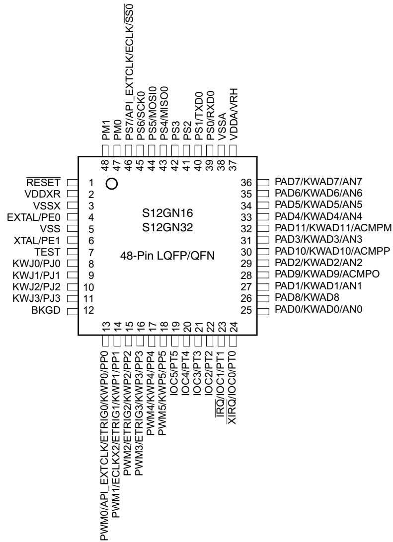
Figure 1-5. 48-Pin LQFP/QFN Pinout for S12GN16 and S12GN32
