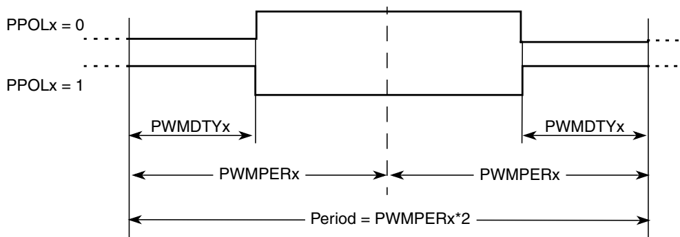
Figure 19-19. PWM Center Aligned Output Waveform
