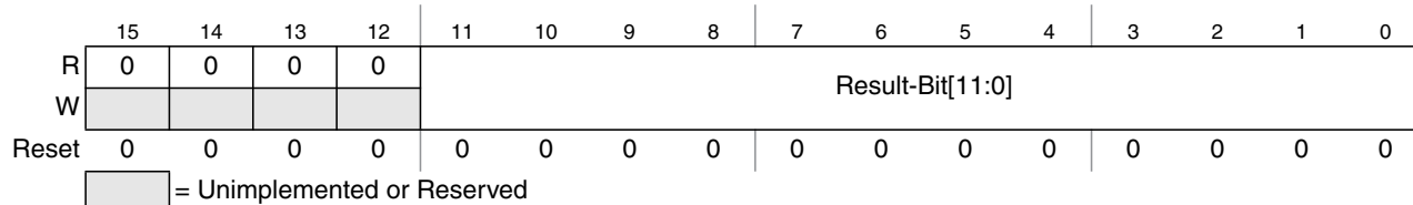
Figure 15-15. Right justified ATD conversion result register (ATDDRn)
