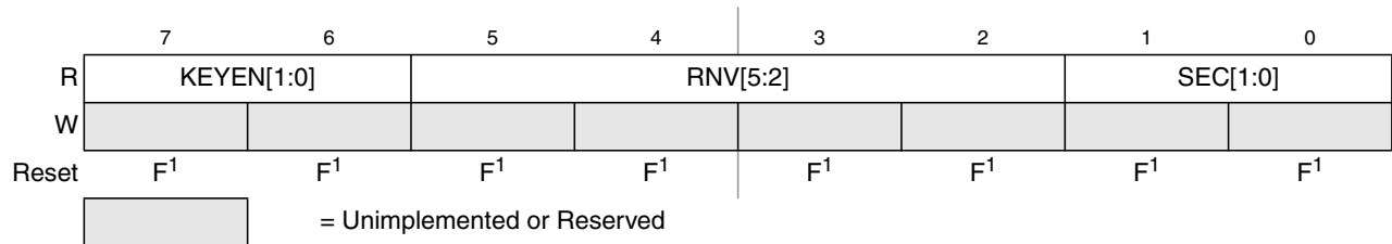
Figure 26-6. Flash Security Register (FSEC)
