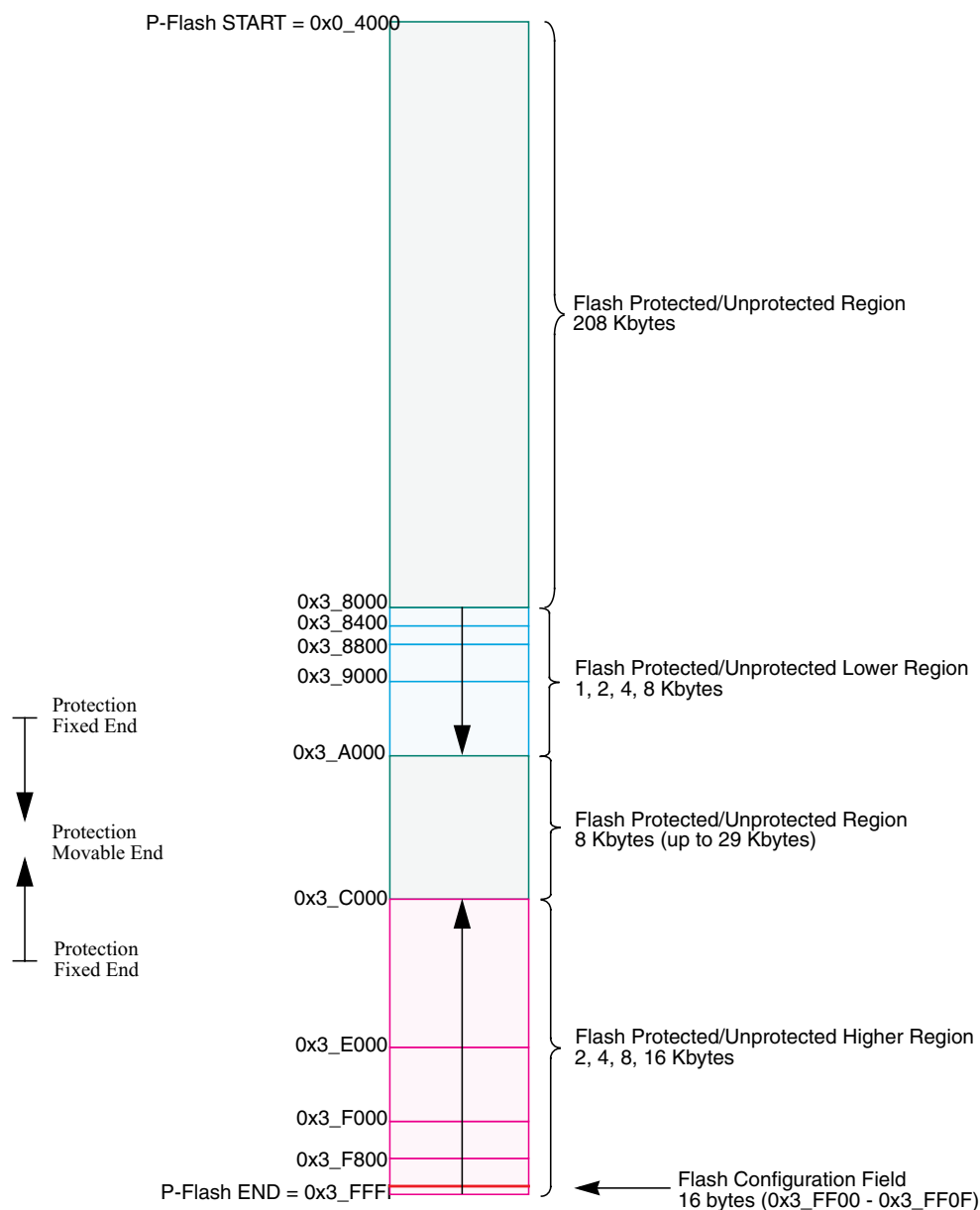
Figure 31-2. P-Flash Memory Map
