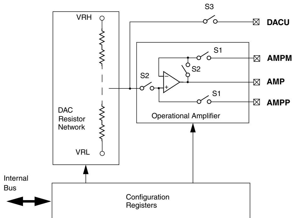
Figure 17-1. DAC_8B5V Block Diagram
