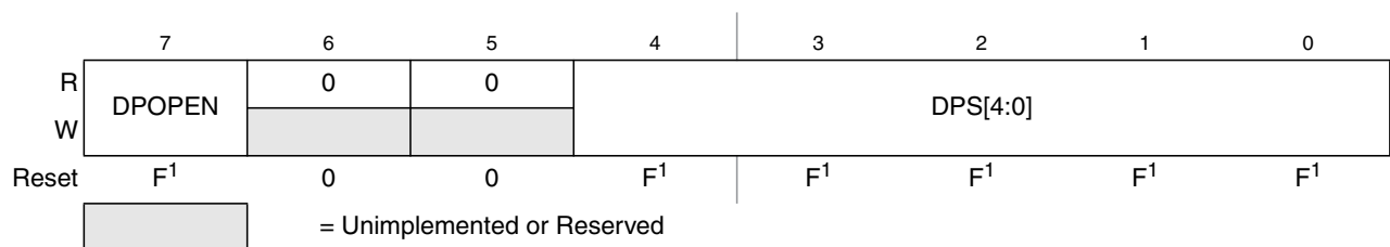
Figure 25-15. EEPROM Protection Register (EPROT)
