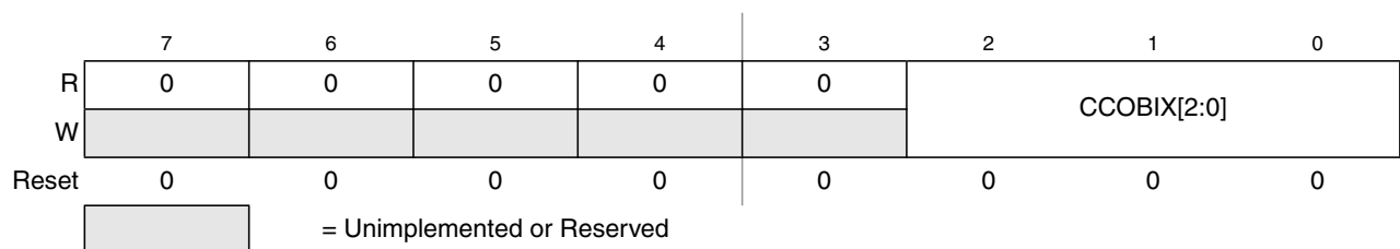
Figure 31-7. FCCOB Index Register (FCCOBIX)
