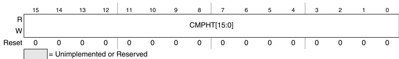
Figure 15-13. ATD Compare Higher Than Register (ATDCMPHT)
