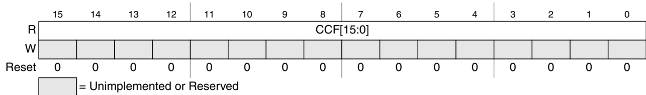
Figure 16-11. ATD Status Register 2 (ATDSTAT2)
