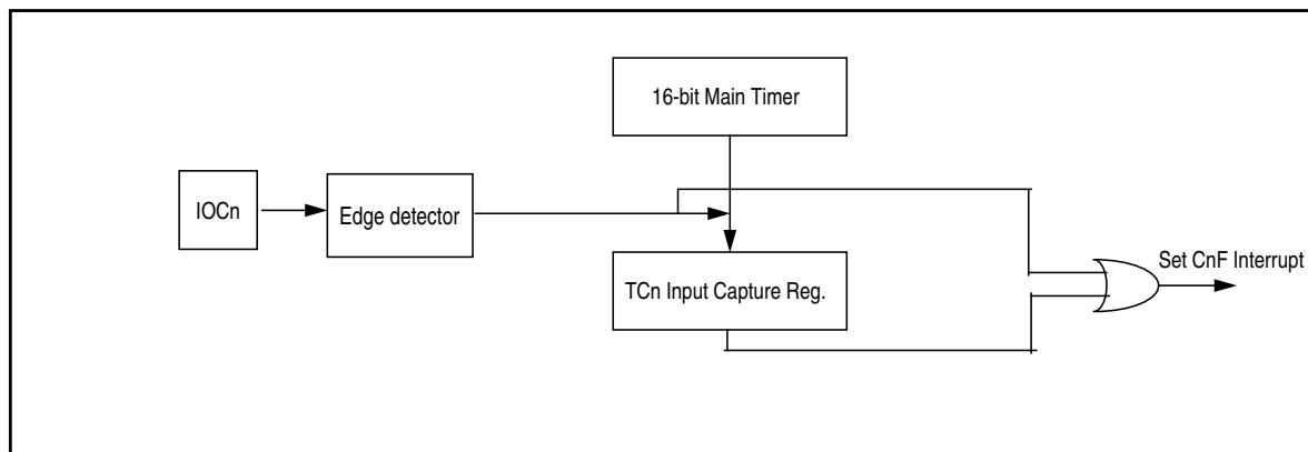
Figure 23-3. Interrupt Flag Setting
