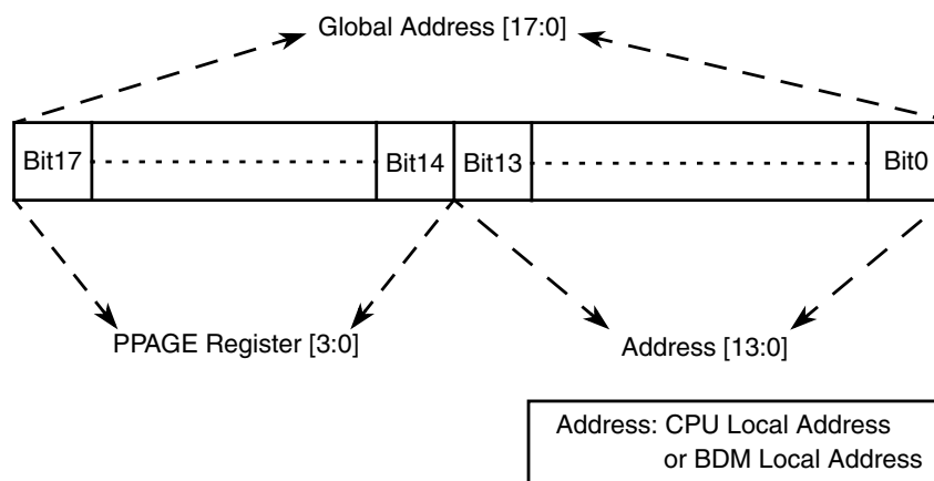
Figure 5-9. PPAGE Address Mapping
