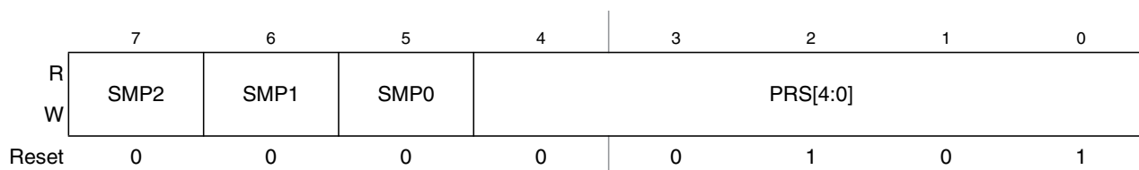
Figure 12-7. ATD Control Register 4 (ATDCTL4)
