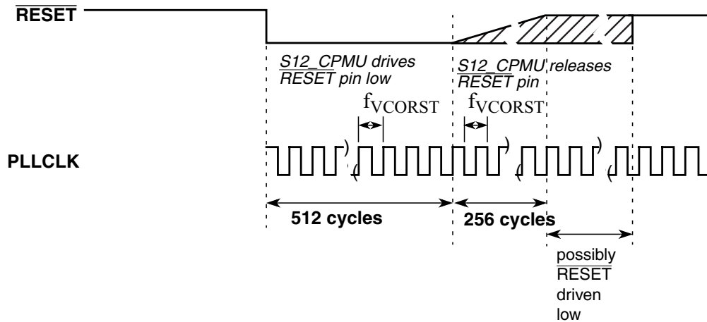
Figure 10-34. RESET Timing
