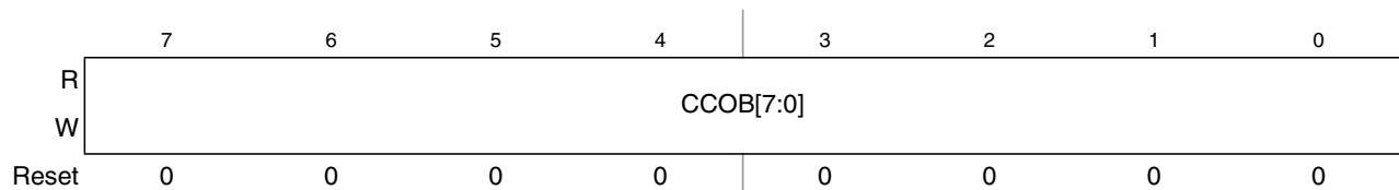
Figure 25-17. Flash Common Command Object Low Register (FCCOBLO)
