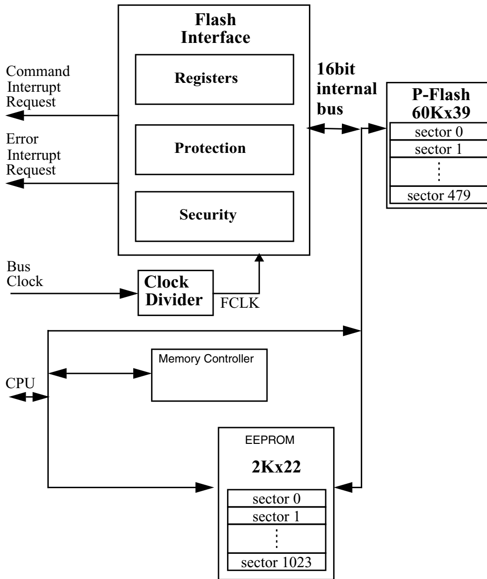
Figure 31-1. FTMRG240K2 Block Diagram
