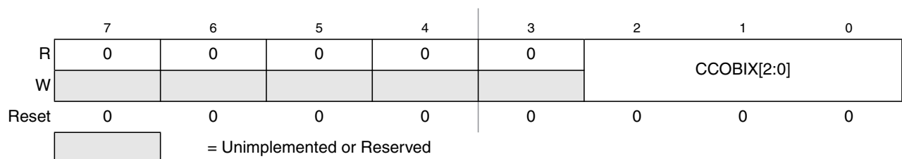
Figure 30-7. FCCOB Index Register (FCCOBIX)
