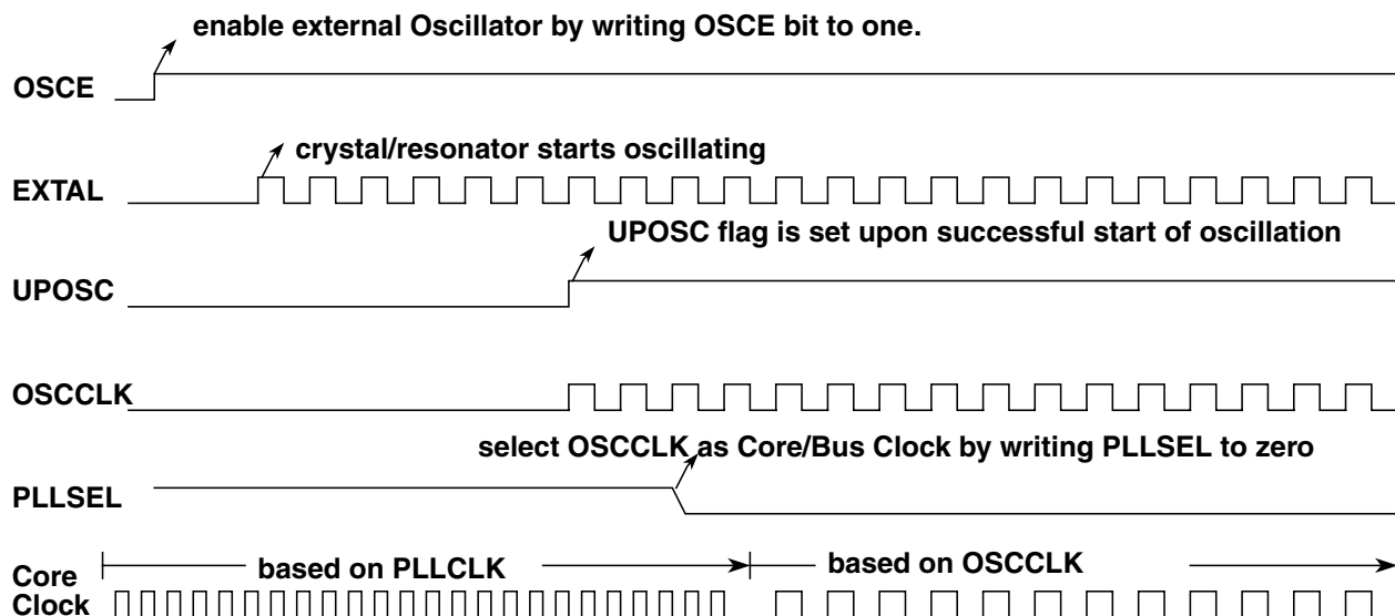
Figure 10-33. Enabling the External Oscillator
