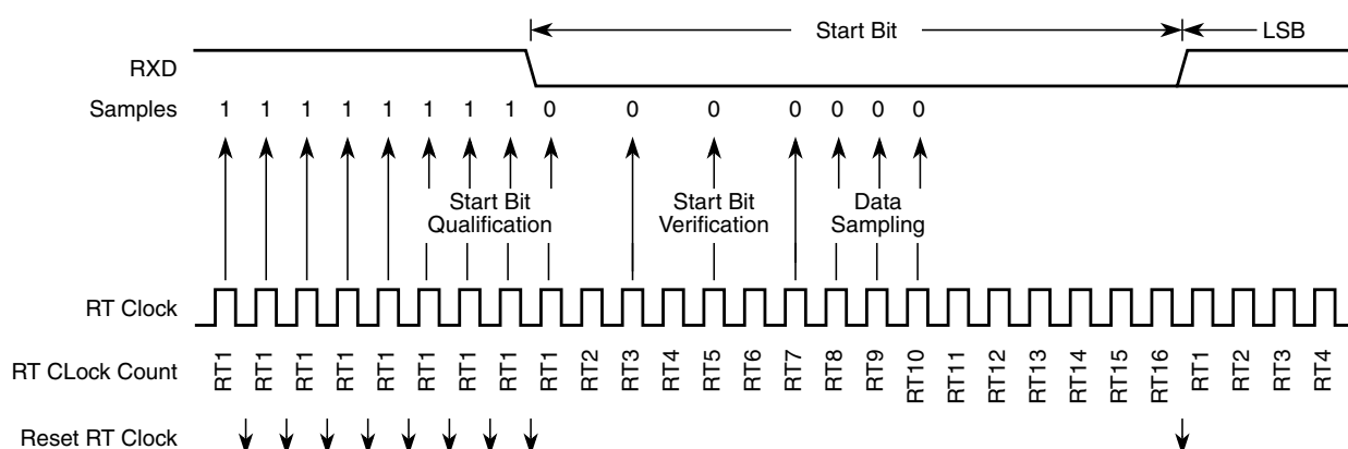
Figure 20-21. Receiver Data Sampling
