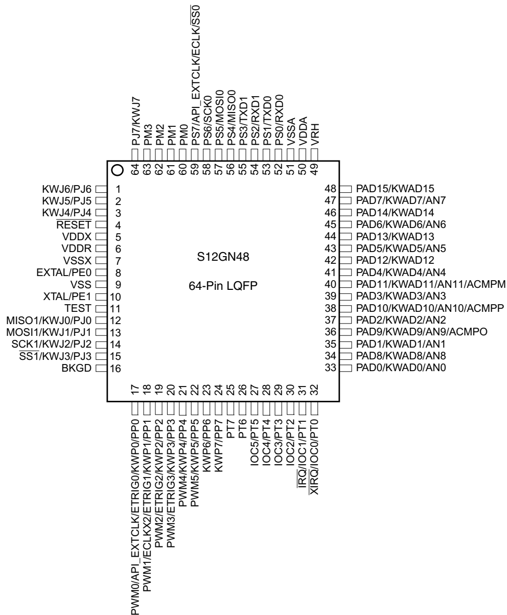
Figure 1-9. 64-Pin LQFP Pinout for S12GN48
