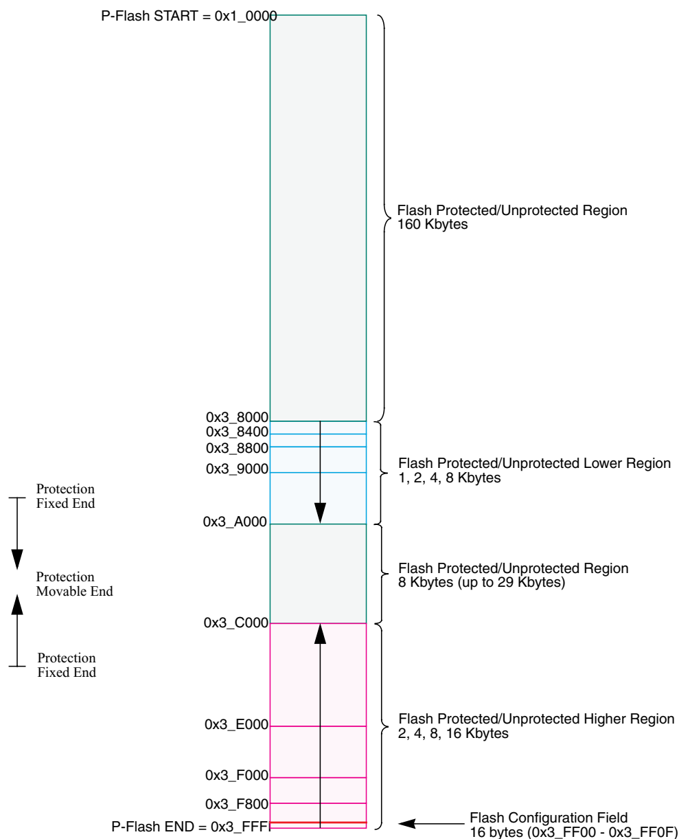
Figure 30-2. P-Flash Memory Map
