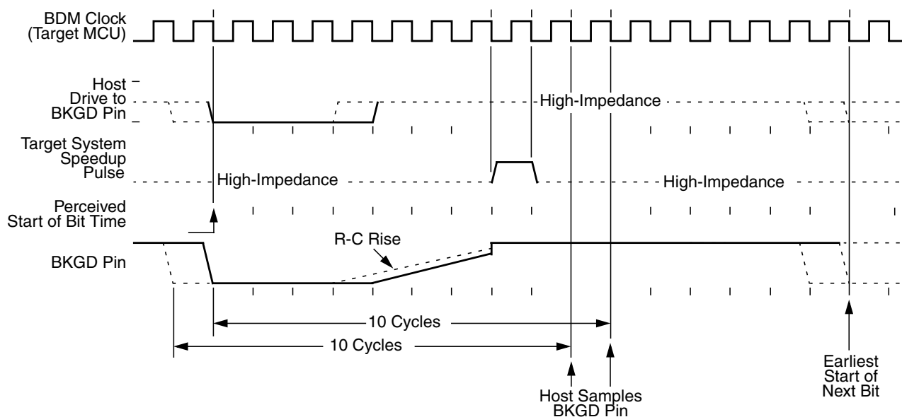
Figure 7-8. BDM Target-to-Host Serial Bit Timing (Logic 1)
