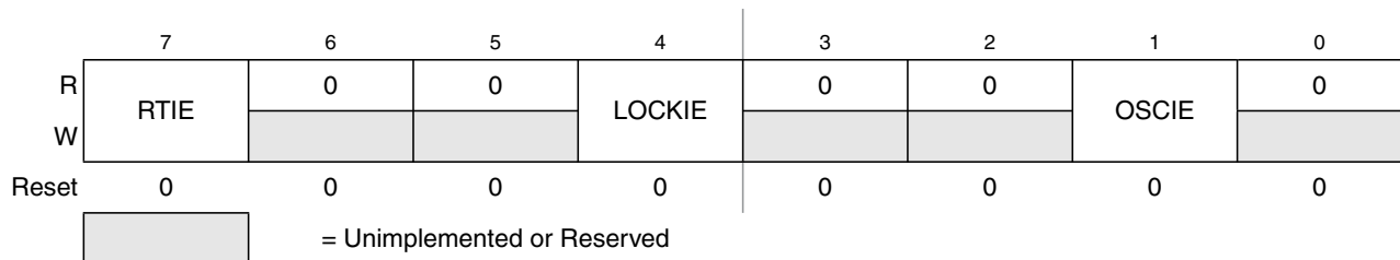
Figure 10-8. S12CPMU Interrupt Enable Register (CPMUINT)
