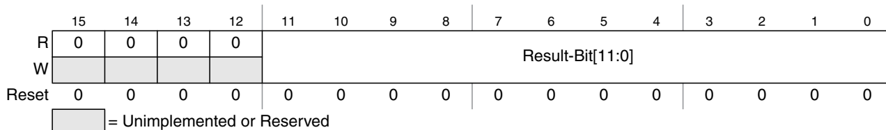
Figure 14-15. Right justified ATD conversion result register (ATDDRn)
