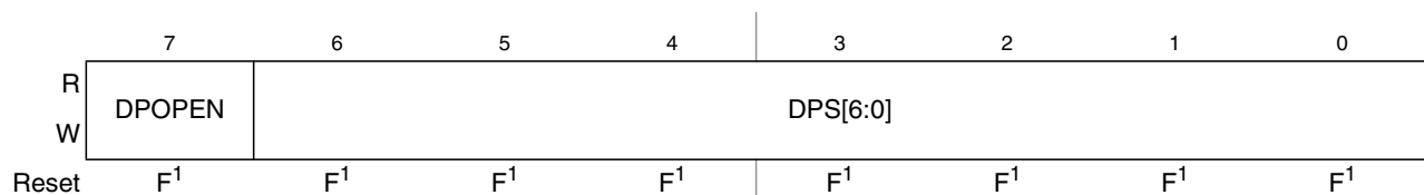
Figure 28-15. EEPROM Protection Register (EPROT)
