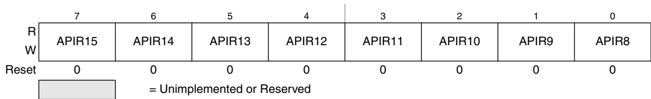
Figure 10-20. Autonomous Periodical Interrupt Rate High Register (CPMUAPIRH)
