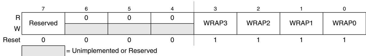
Figure 14-3. ATD Control Register 0 (ATDCTL0)
