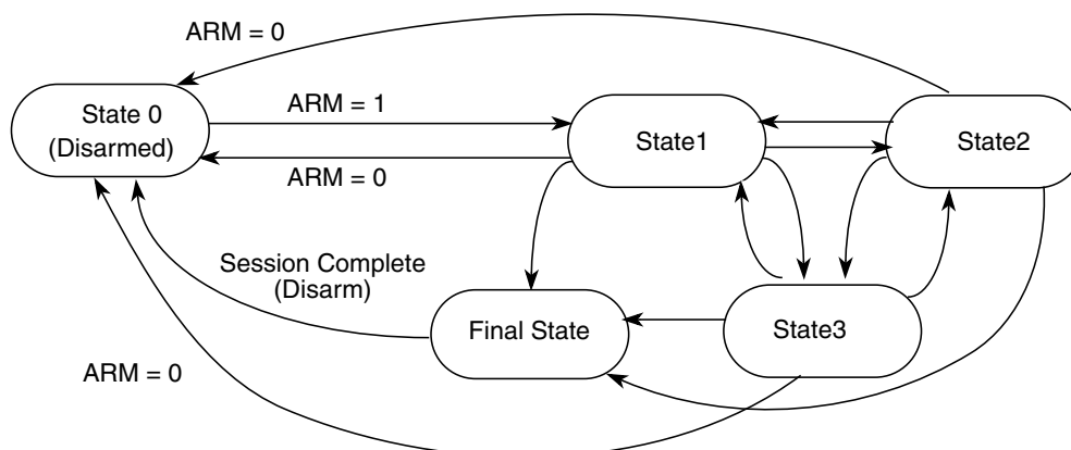
Figure 8-24. State Sequencer Diagram
