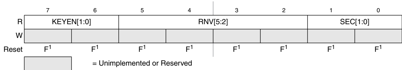
Figure 27-6. Flash Security Register (FSEC)
