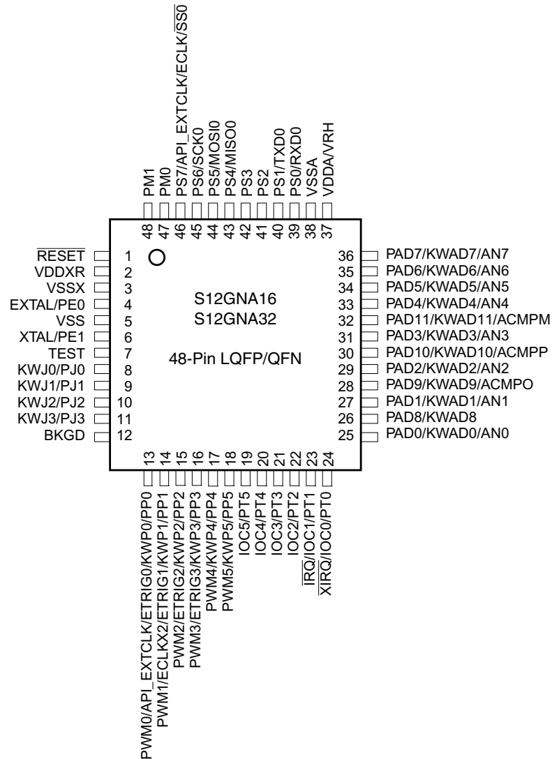
Figure 1-6. 48-Pin LQFP/QFN Pinout for S12GNA16 and S12GNA32
