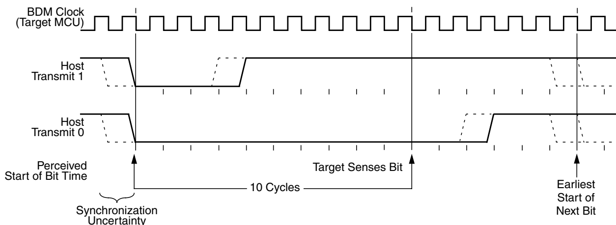
Figure 7-7. BDM Host-to-Target Serial Bit Timing
