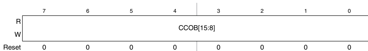
Figure 28-16. Flash Common Command Object High Register (FCCOBHI)
