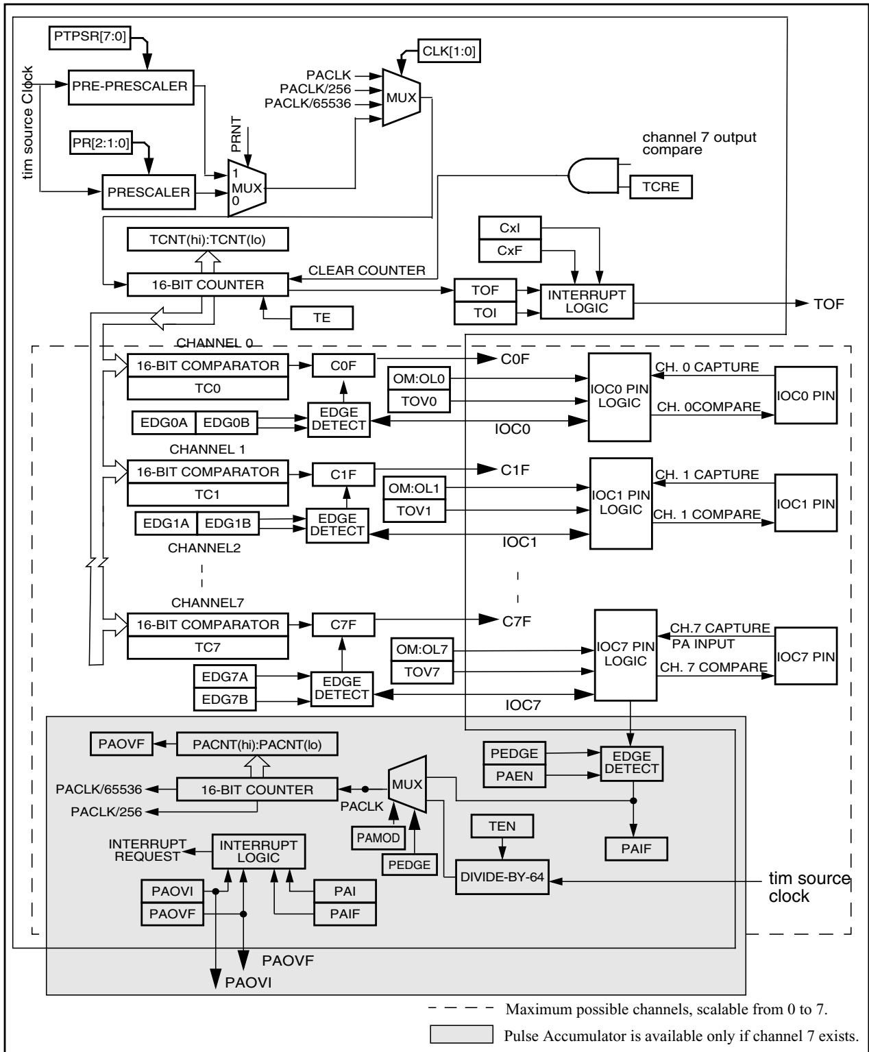
Figure 23-30. Detailed Timer Block Diagram
