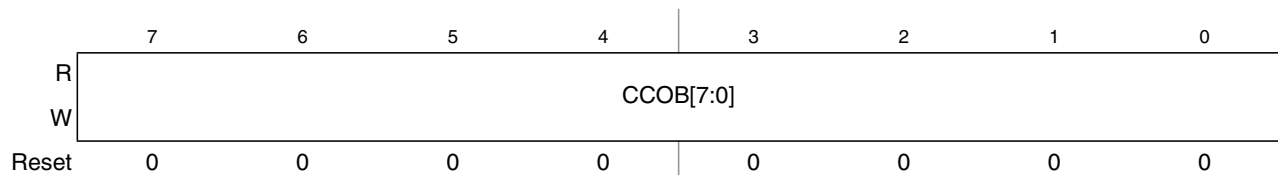
Figure 24-16. Flash Common Command Object Low Register (FCCOBLO)
