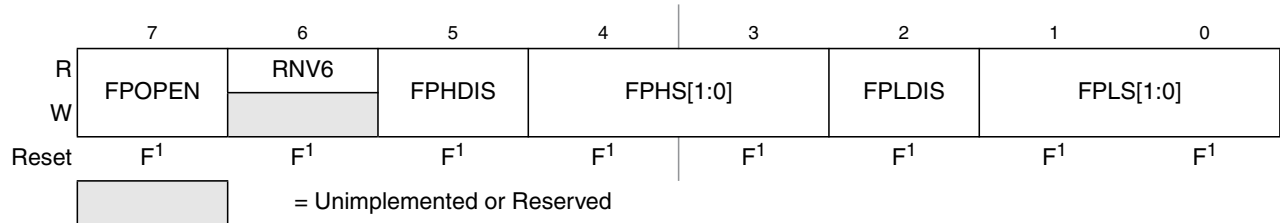
Figure 29-13. Flash Protection Register (FPROT)
