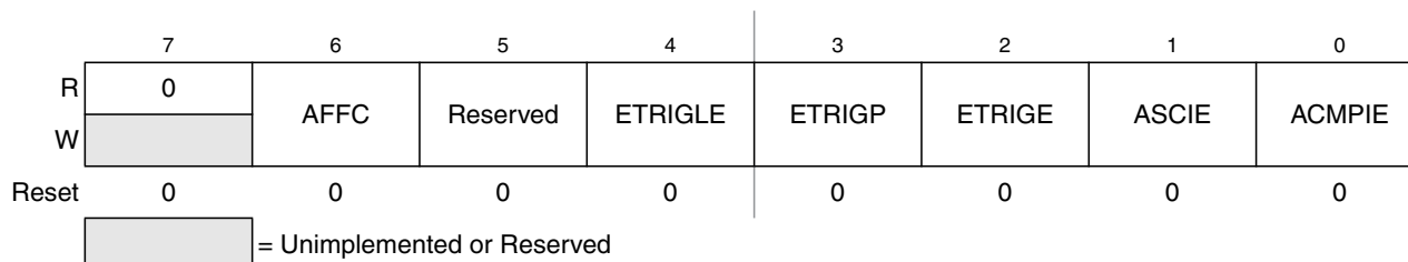
Figure 16-5. ATD Control Register 2 (ATDCTL2)
