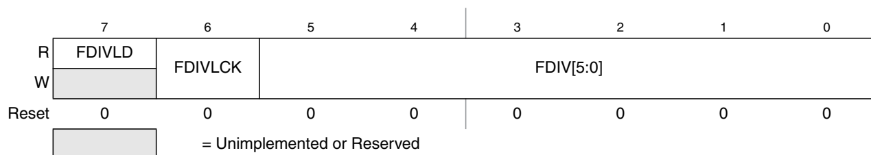
Figure 29-5. Flash Clock Divider Register (FCLKDIV)
