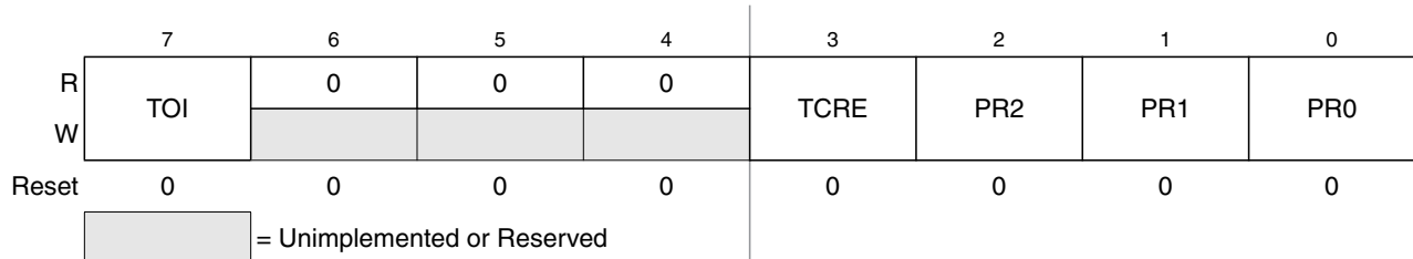
Figure 23-19. Timer System Control Register 2 (TSCR2)
