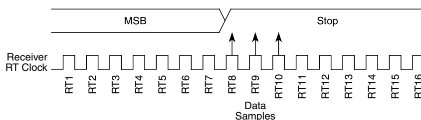
Figure 20-28. Slow Data
