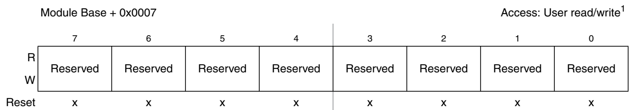
Figure 17-5. Reserved Registerfv_dac_8b5v_RESERVED
