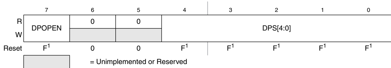
Figure 24-14. EEPROM Protection Register (EEPROT)
