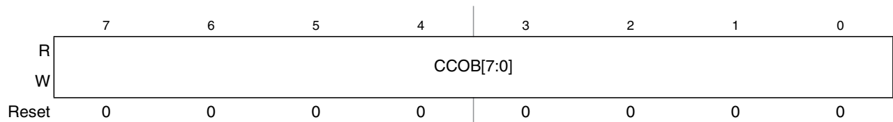
Figure 27-17. Flash Common Command Object Low Register (FCCOBLO)
