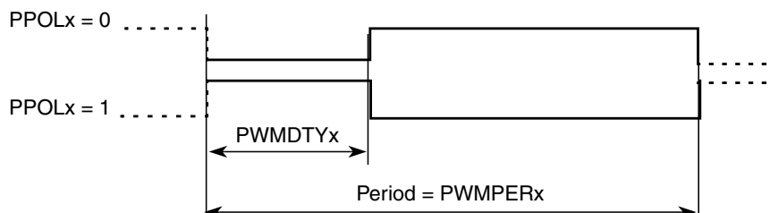
Figure 19-17. PWM Left Aligned Output Waveform
