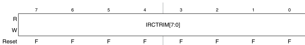
Figure 10-24. S12CPMU IRC1M Trim Low Register (CPMUIRCTRIML)
