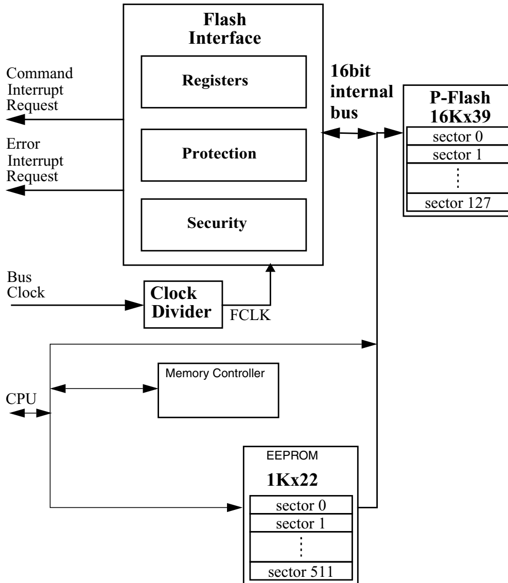
Figure 27-1. FTMRG64K1 Block Diagram
