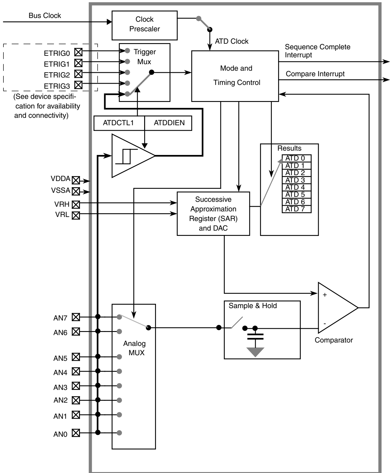
Figure 12-1. ADC12B8C Block Diagram
