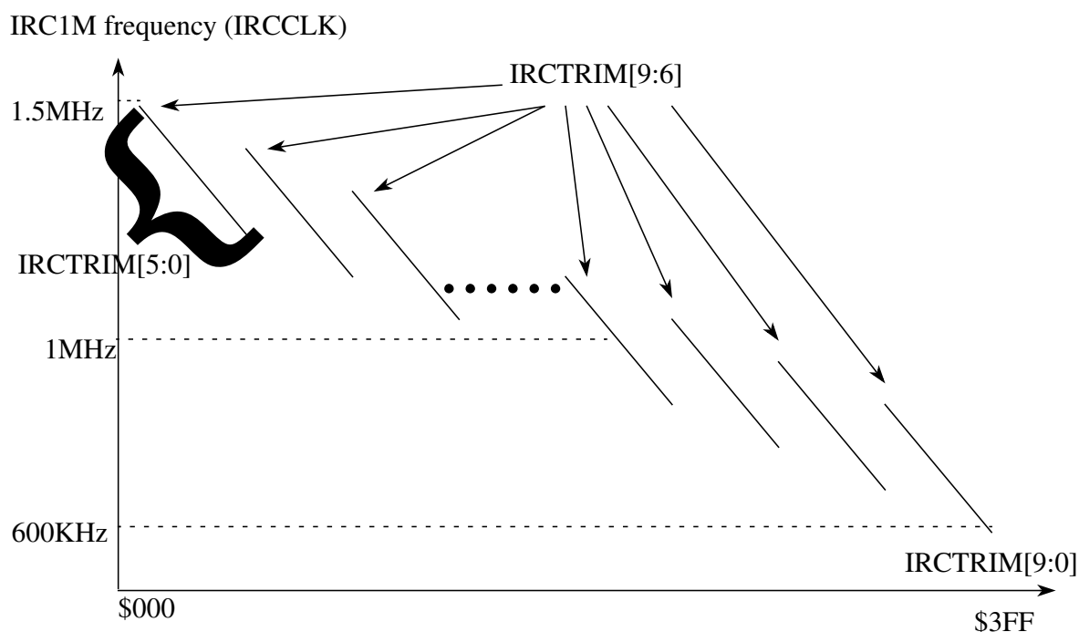
Figure 10-25. IRC1M Frequency Trimming Diagram
