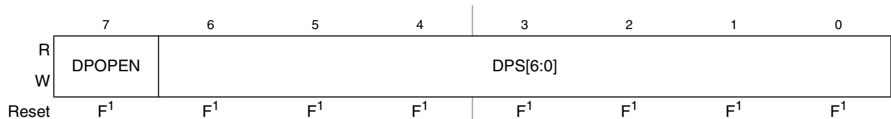
Figure 31-15. EEPROM Protection Register (EPROT)
