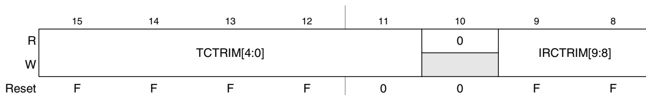
Figure 10-23. S12CPMU IRC1M Trim High Register (CPMUIRCTRIMH)
