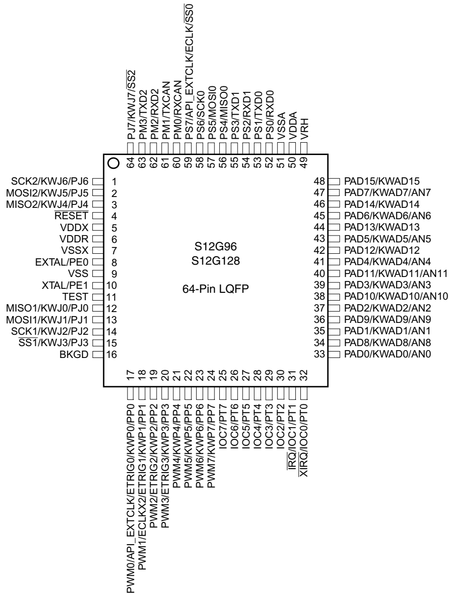
Figure 1-16. 64-Pin LQFP Pinout for S12G96 and S12G128
