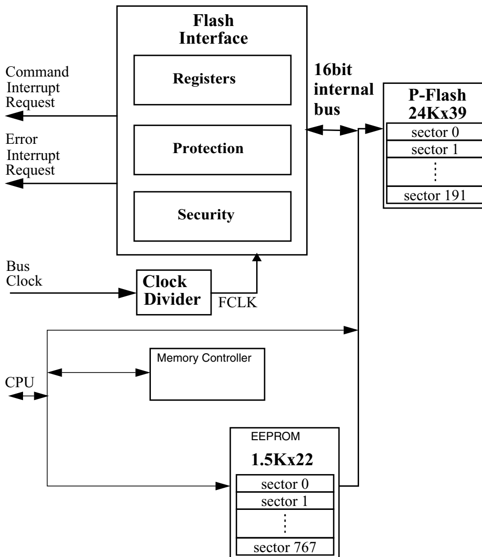
Figure 28-1. FTMRG96K1 Block Diagram
