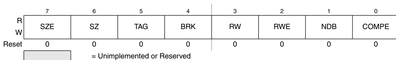
Figure 8-13. Debug Comparator Control Register DBGACTL (Comparator A)
