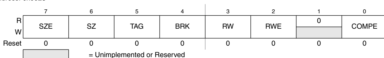
Figure 8-14. Debug Comparator Control Register DBGBCTL (Comparator B)
