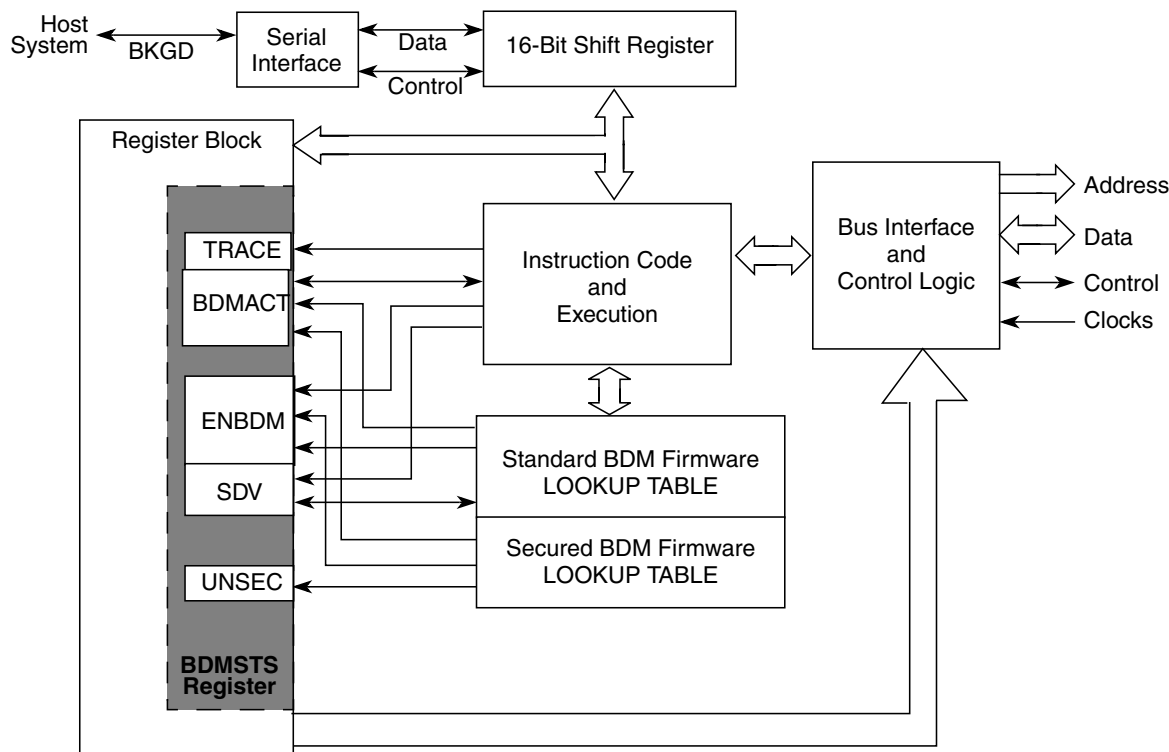
Figure 7-1. BDM Block Diagram
