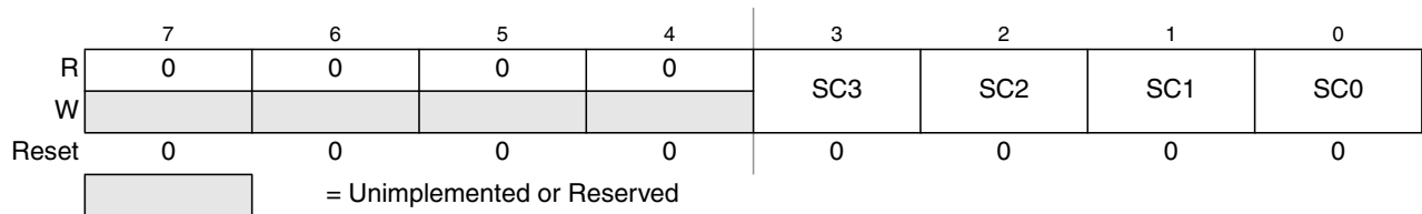
Figure 8-11. Debug State Control Register 3 (DBGSCR3)
