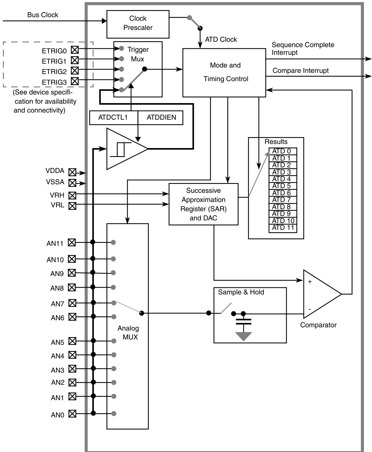
Figure 13-1. ADC10B12C Block Diagram
