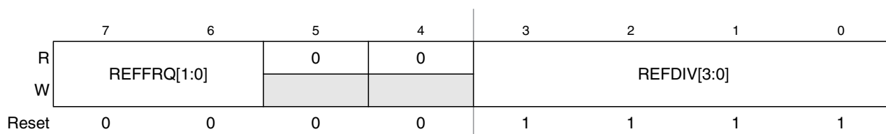
Figure 10-5. S12CPMU Reference Divider Register (CPMUREFDIV)
