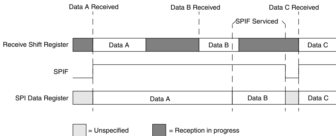
Figure 21-9. Reception with SPIF serviced in Time
