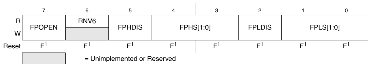
Figure 28-13. Flash Protection Register (FPROT)
