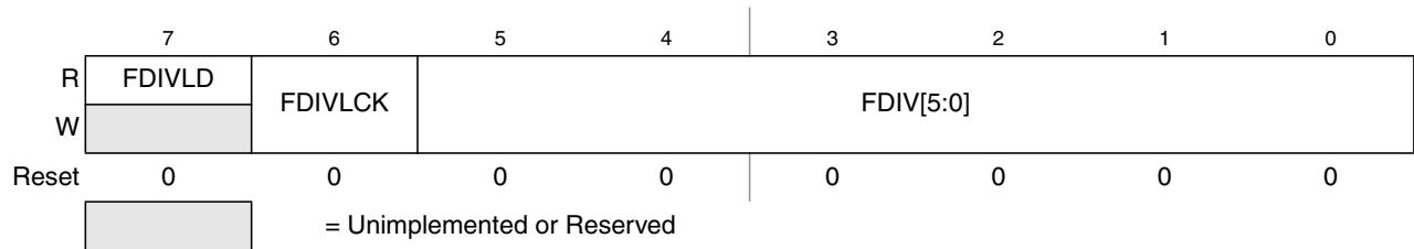
Figure 30-5. Flash Clock Divider Register (FCLKDIV)
