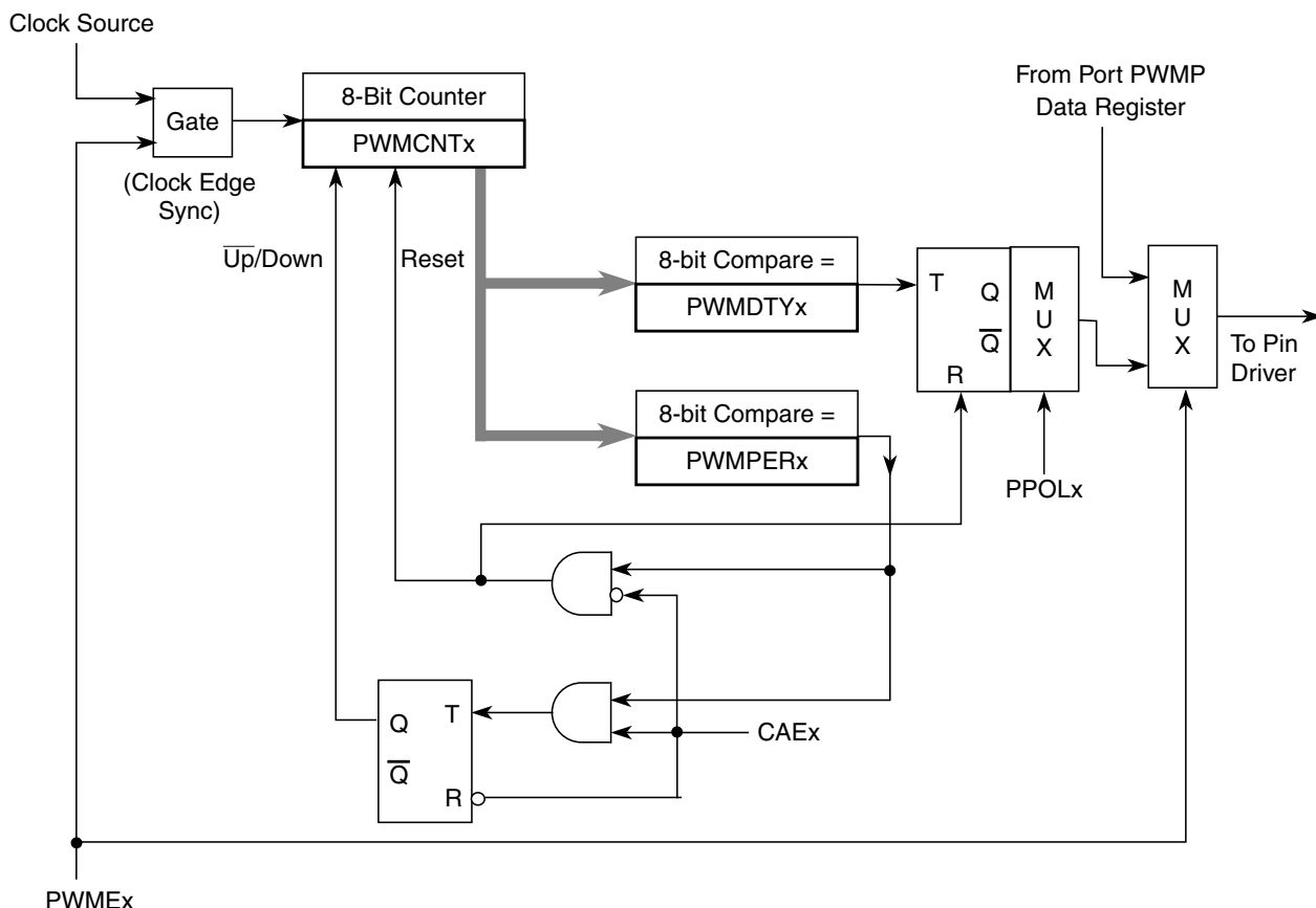
Figure 19-16. PWM Timer Channel Block Diagram
