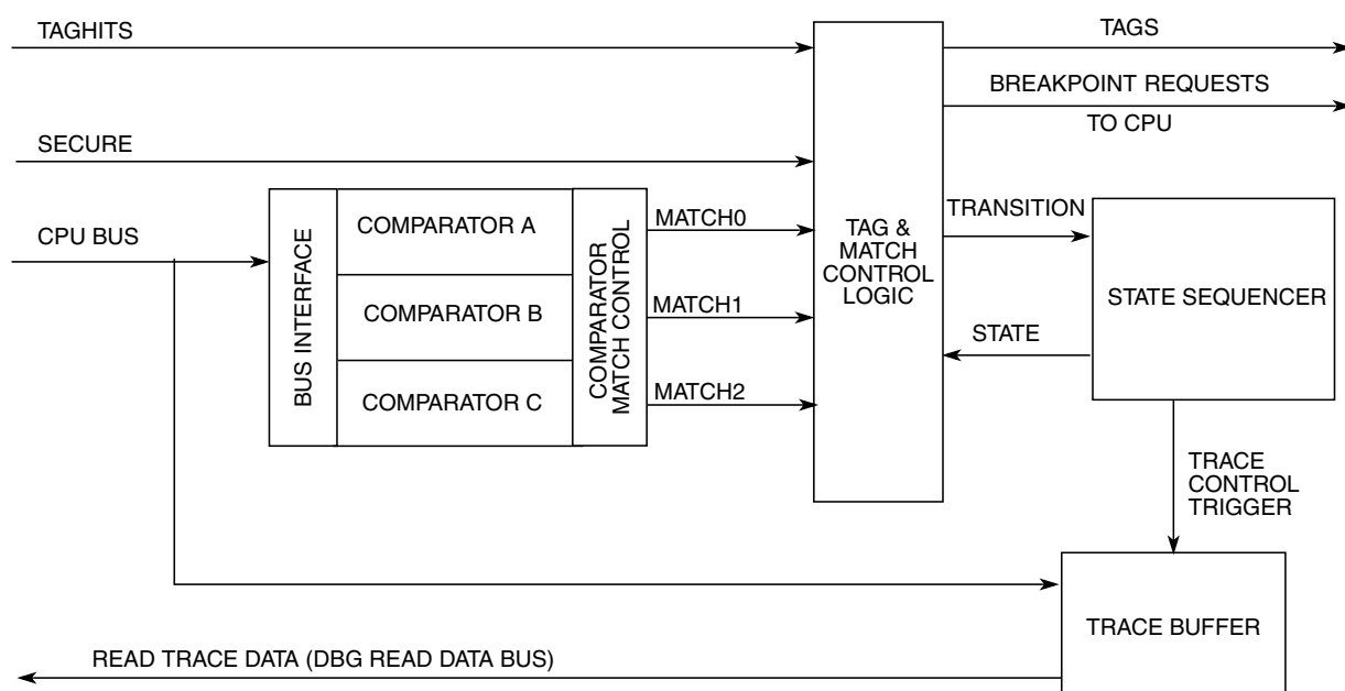
Figure 8-23. DBG Overview
