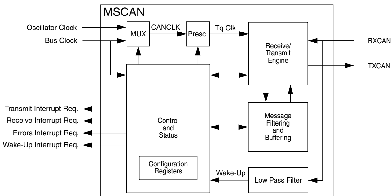
Figure 18-1. MSCAN Block Diagram
