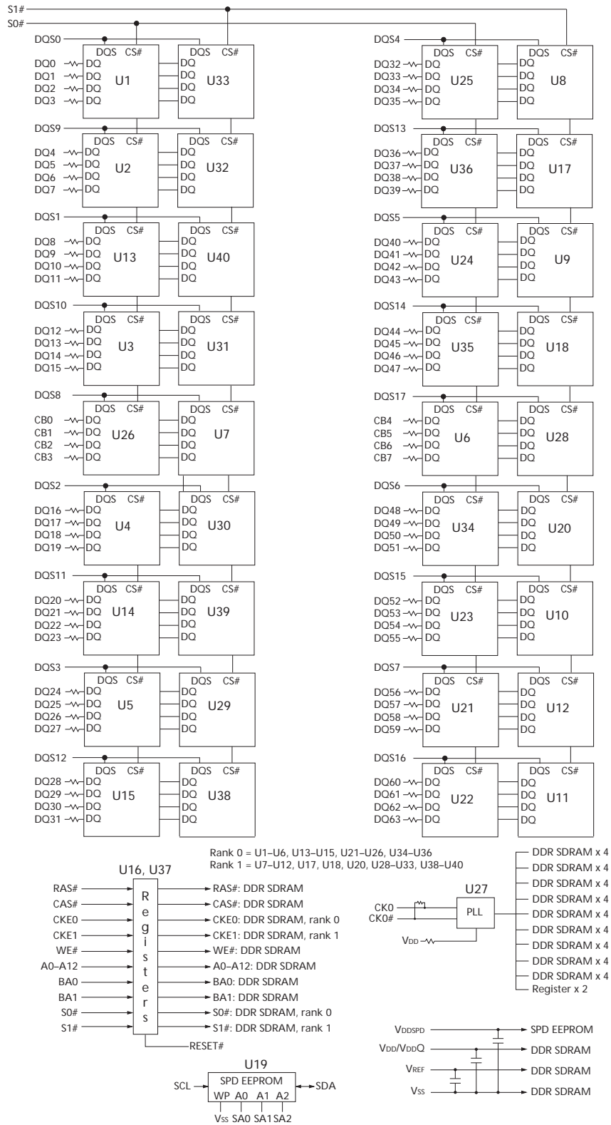
Figure 5: Functional Block Diagram – Standard-Height Layout (1GB)
