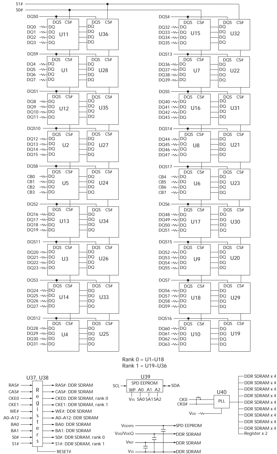
Figure 4: Functional Block Diagram – Tall-Height Layout (1GB, 2GB)
