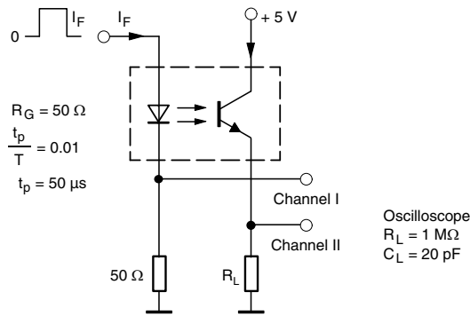
95 10804-3 Fig. 2 - Test Circuit, Non-Saturated Operation
