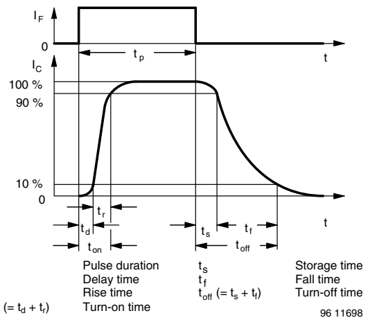
Fig. 4 - Switching Times
