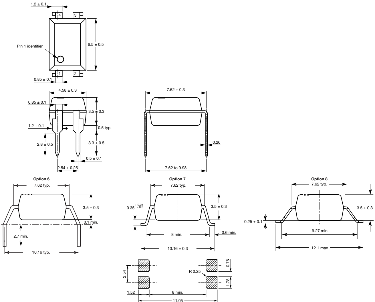
Fig. 17 - Package Drawings
