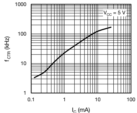
Fig. 15 - Frequency (-3 dB) vs. Collector Current
