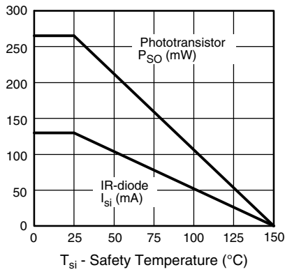
Fig. 4 - Derating Diagram
