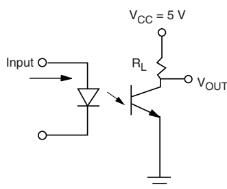
Fig. 2 - Test Circuit
