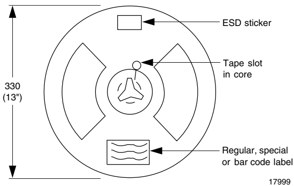
Fig. 20 - Reel Dimensions (3000 units per reel)
