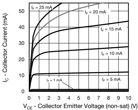
Fig. 7 - Collector Current vs. Collector Emitter Voltage (non-saturated)
