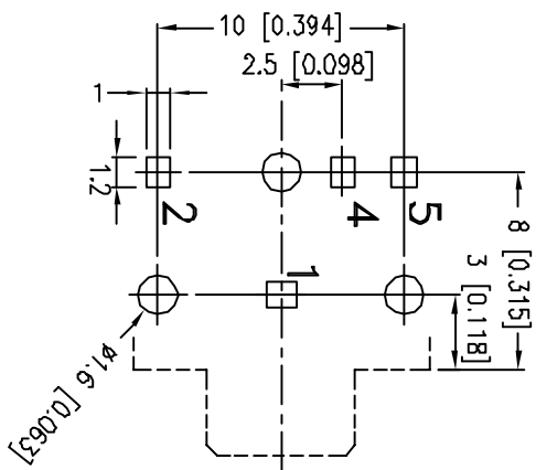
HOLE LAYOUT (TOP VIEW)
