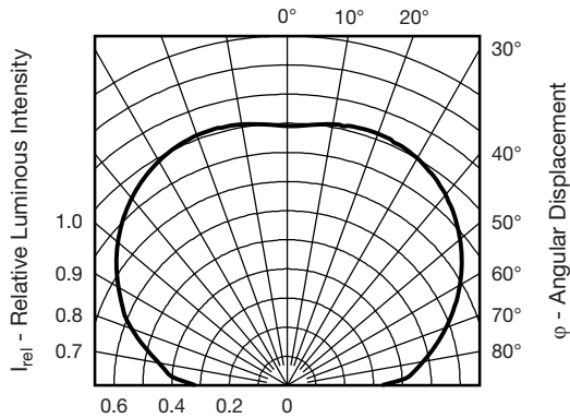
Fig. 19 - Relative Luminous Intensity vs. Angular Displacement
