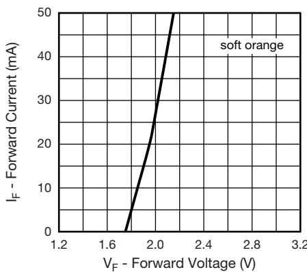
Fig. 3 - Forward Current vs. Forward Voltage (soft orange)
