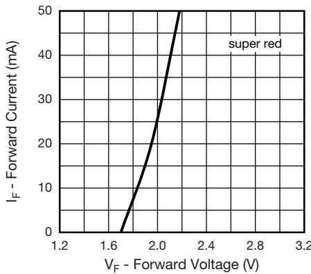
Fig. 2 - Forward Current vs. Forward Voltage (super red)
