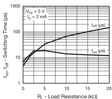
Fig. 16 - Switching Time vs. Load Resistance
