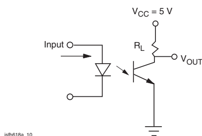
Fig. 3 - Test Circuit
