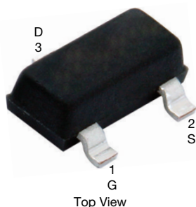
SOT-23 (TO-236)
