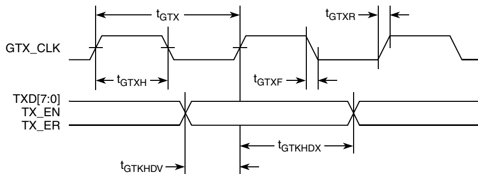
Figure 12. GMII Transmit AC Timing Diagram
