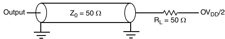
Figure 63. Timers AC Test Load
