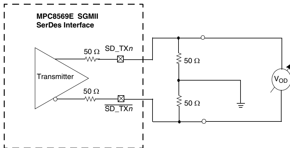
Figure 28. SGMII Transmitter DC Measurement Circuit
