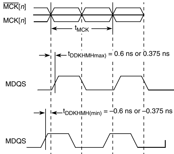
Figure 9. Timing Diagram for t_{DDKHMH}
