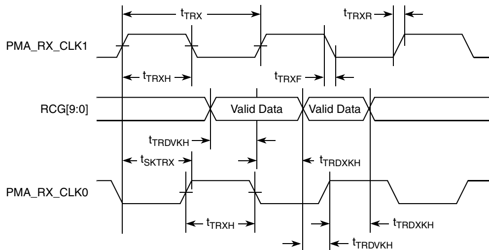
Figure 24. TBI Receive AC Timing Diagram
