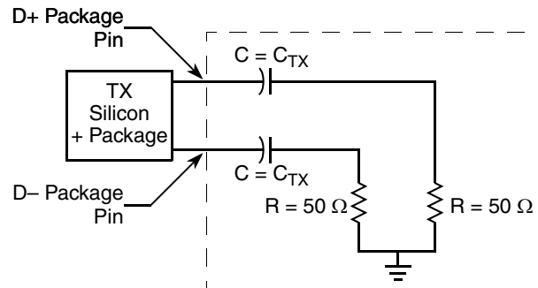
Figure 29. SGMII AC Test/Measurement Load
