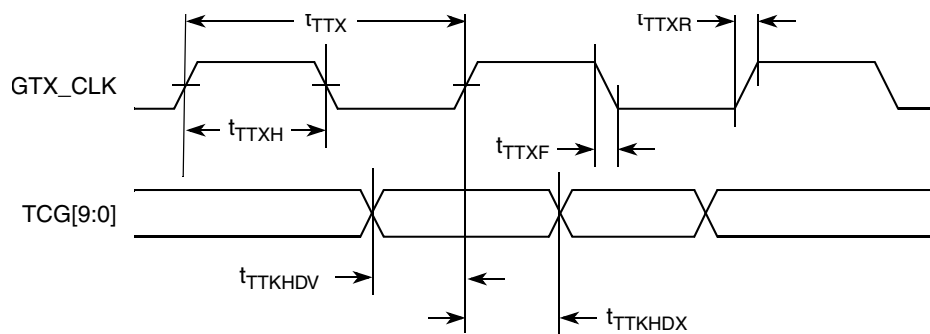
Figure 22. TBI Transmit AC Timing Diagram
