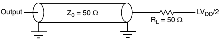
Figure 16. MII AC Test Load
