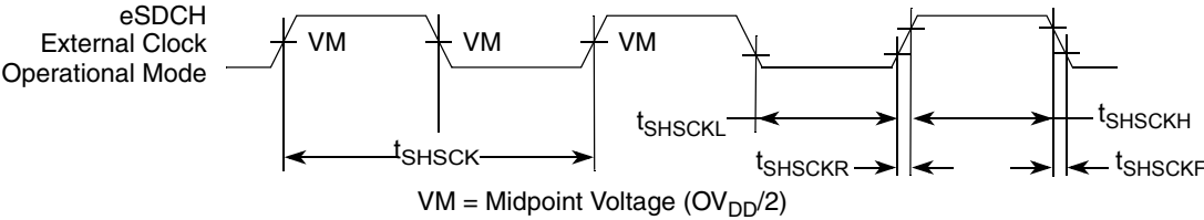
Figure 61. eSDHC Clock Input Timing Diagram
