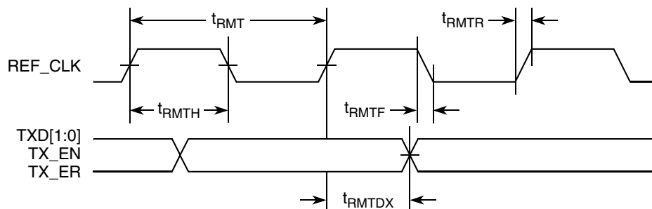
Figure 19. RMII Transmit AC Timing Diagram
