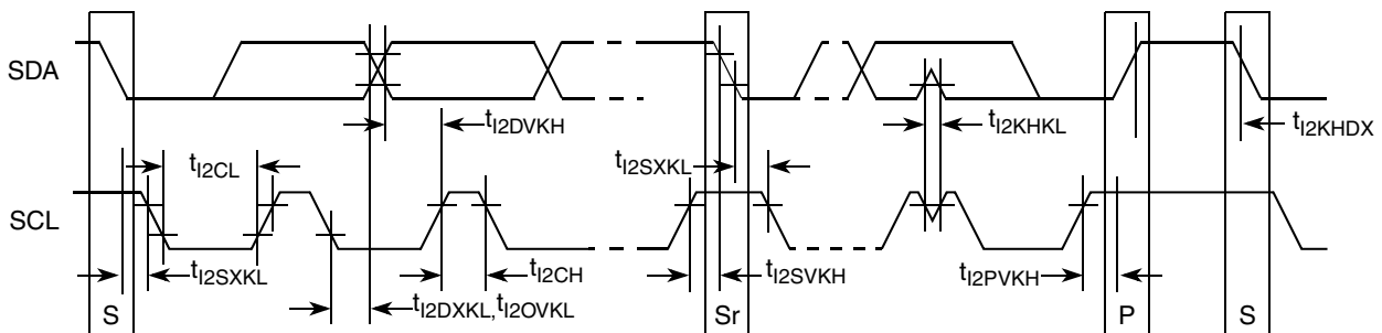
Figure 50. I 2 C Bus AC Timing Diagram
