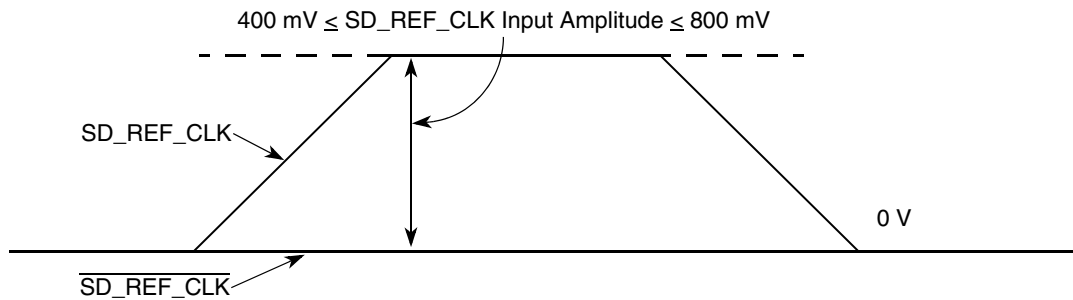
Figure 42. Single-Ended Reference Clock Input DC Requirements
