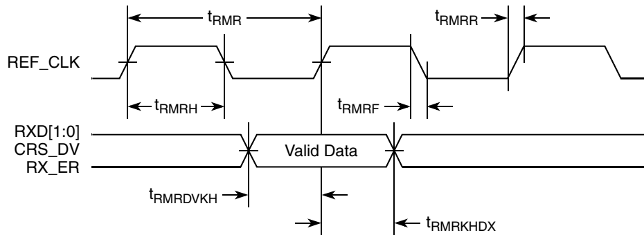
Figure 21. RMII Receive AC Timing Diagram
