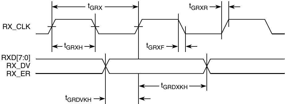
Figure 14. GMII Receive AC Timing Diagram
