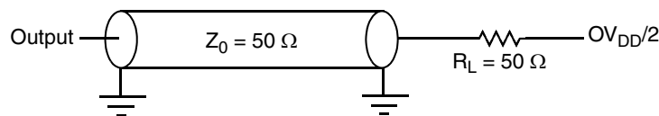
Figure 51. GPIO AC Test Load
