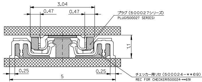
嵌合断面図(参考) MATED DRAWING
