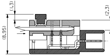
SECT B-B (SCALE:4-1)
