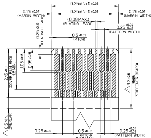
適合するFPC推奨寸法 APPLICABLE FPC RECOMMENDED DIMENSION
