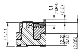
SECTION Z-Z
