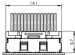
嵌合図 MATED CONNECTORES
