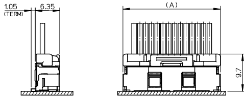
嵌合図 MATED CONNECTORS
