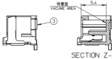
SECTION Z-Z
