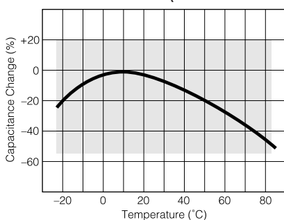
Char. E/Y5U (Temp.Range:-25 to 85 °C max.Cap.Change:+20, -55 %)
