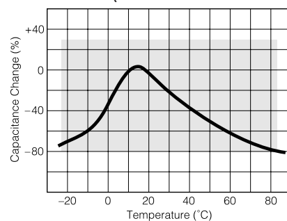
Char. F/Y5V (Temp.Range:-25 to 85 °C max.Cap.Change:+30, -80 %)
