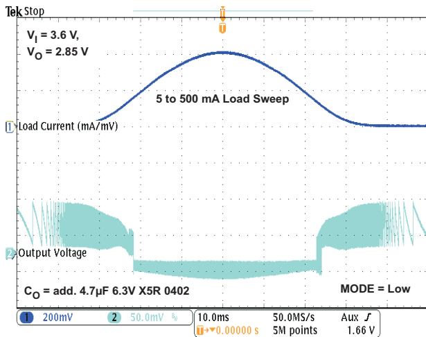
AC LOAD TRANSIENT RESPONSE
