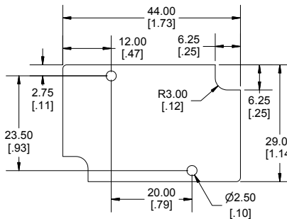
MAXIMUM P.C. BOARD SIZE
