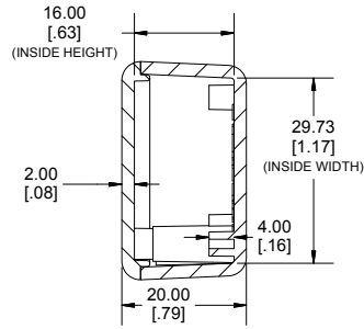
END VIEW SECTION B-B
